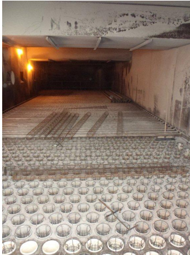
Figure 7: Inside one of the existing FFP's at the power station
