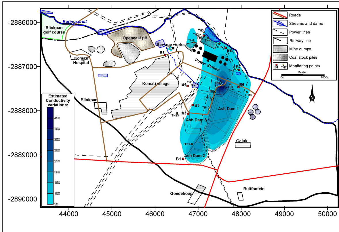
Figure 16. Simulated electrical conductivity increase (mS/m): Current situation.
