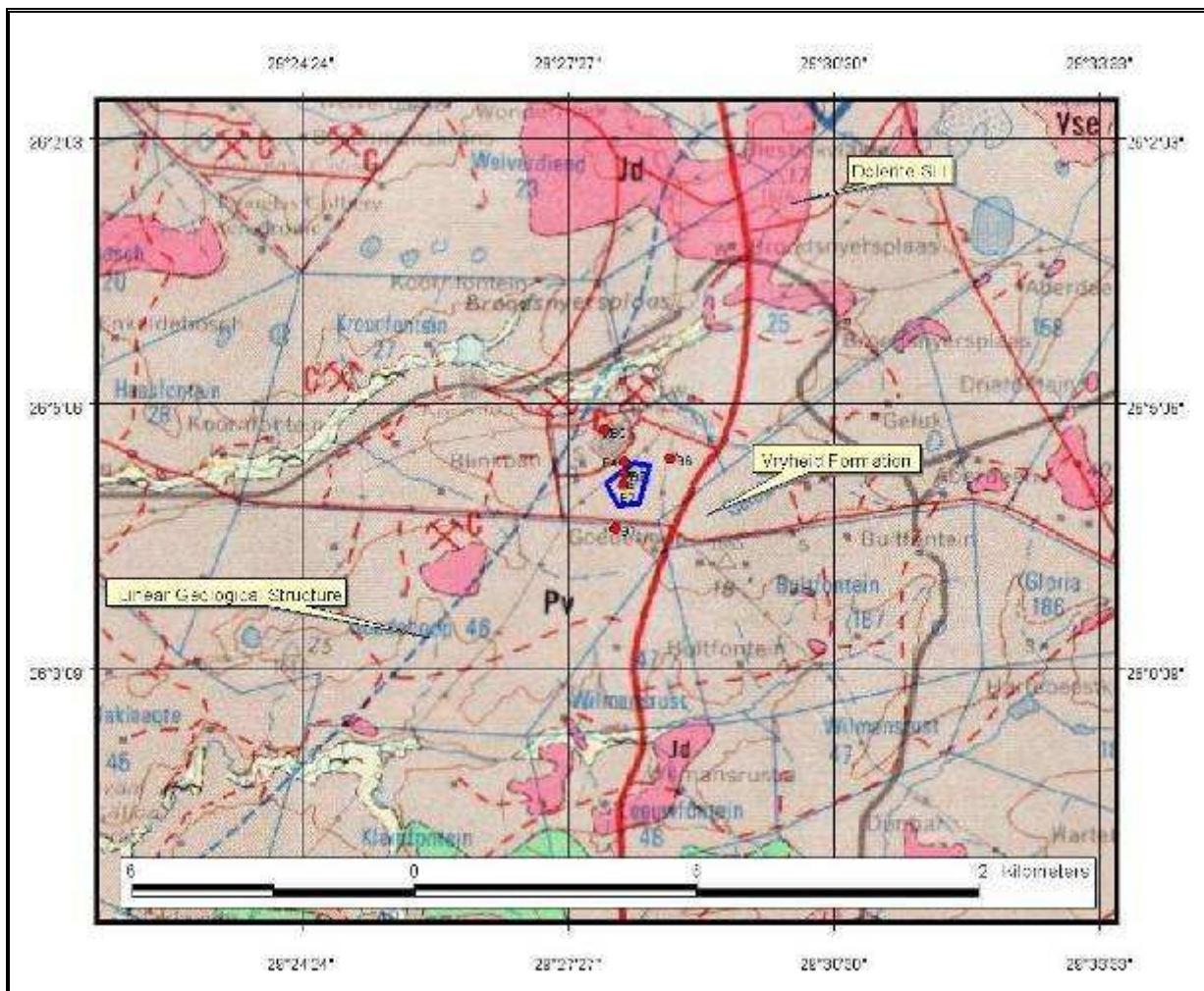
Figure 3: Regional Geology.
