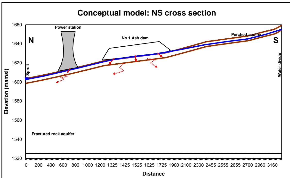
Figure 9. Conceptual groundwater model of the current situation.
