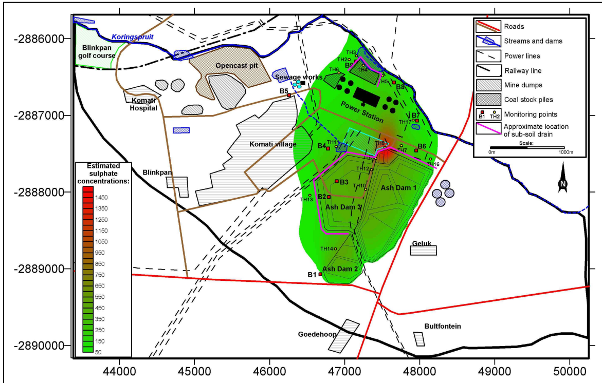
Figure 17. Simulated sulphate concentrations (mg/l): Potential future impact including extension to ash dams and remedial measures
