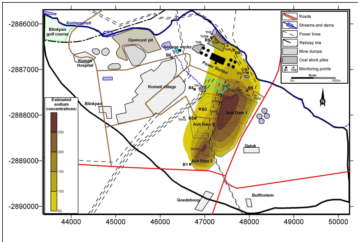
Figure 15. Simulated sodium concentrations (mg/l): Current situation.
