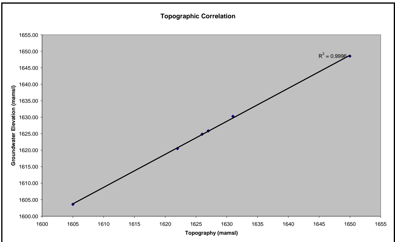
Figure 5. Correlation between topography and groundwater elevation (mamsl).
