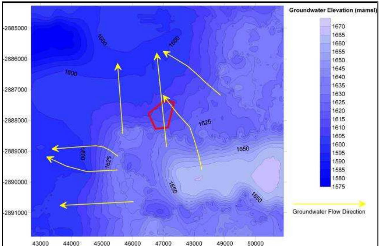
Figure 6. Interpolated local groundwater gradients and flow directions.
