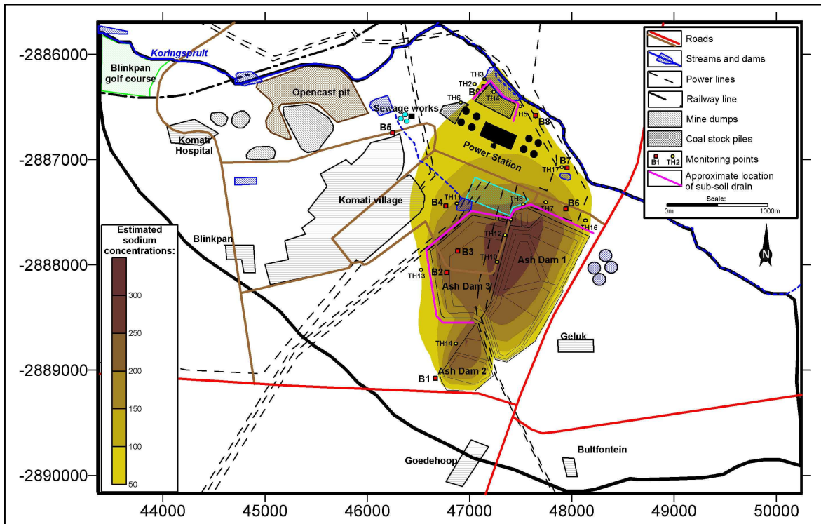
Figure 18. Simulated sodium concentrations (mg/l): Potential future impact including extension to ash dams and remedial measures.
