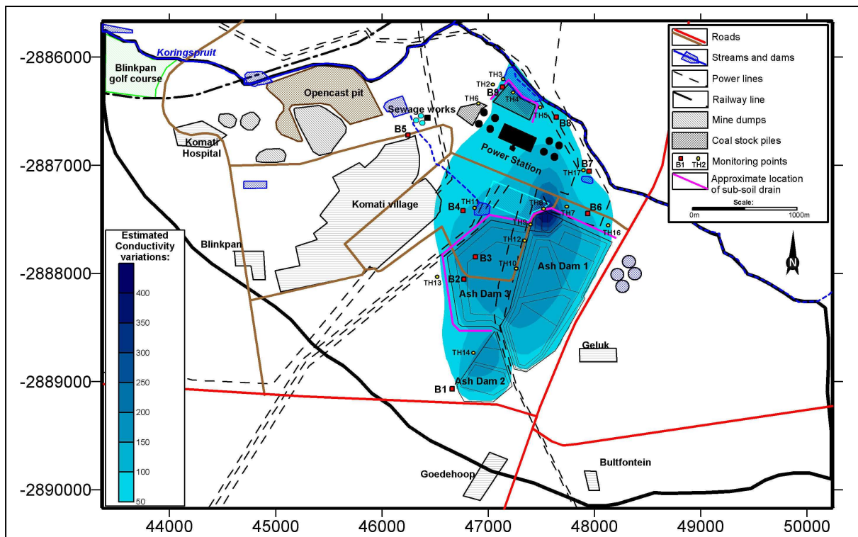
Figure 19. Simulated electrical conductivity increase (mS/m): Potential future impact including extension to ash dams and remedial measures.
