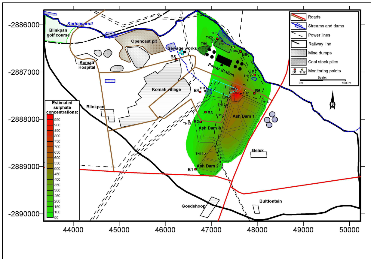
Figure 14. Simulated sulphate concentrations (mg/l): Current situation.
