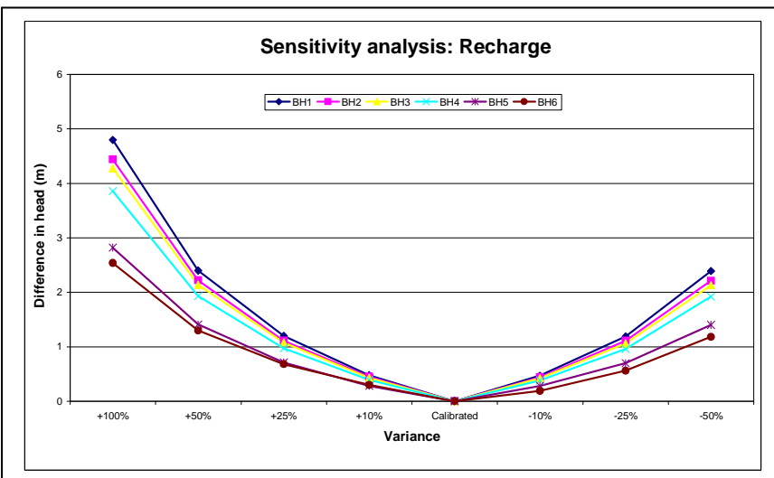
Figure 13. Results of the sensitivity analysis.
