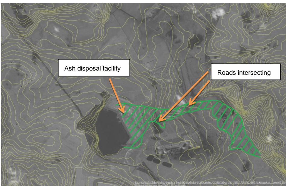
B. Recent aerial imagery showing power station infrastructure in relation to historic wetland
