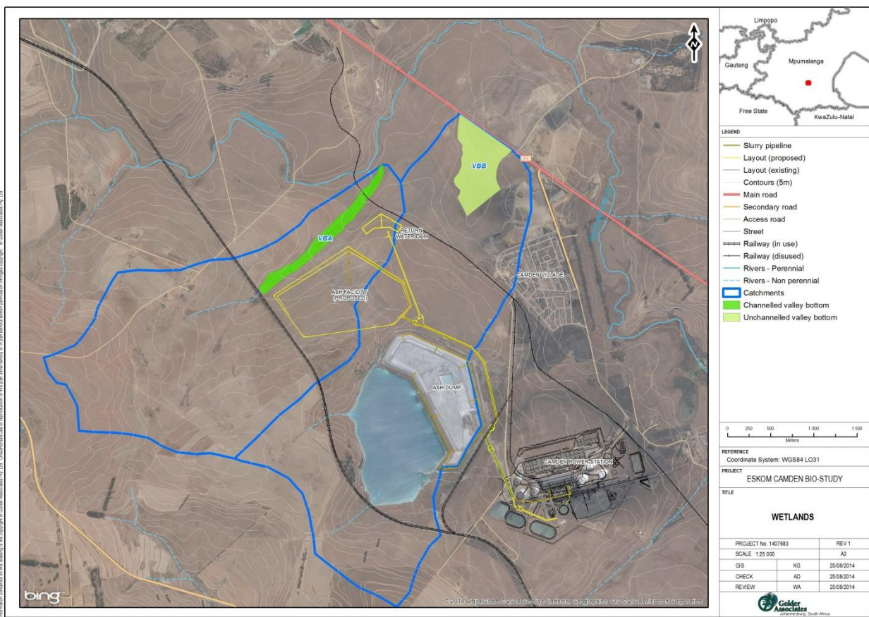
Figure 1: Location of infrastructure in Preferred Site 1 – the Study Area for wetland and aquatic assessment
