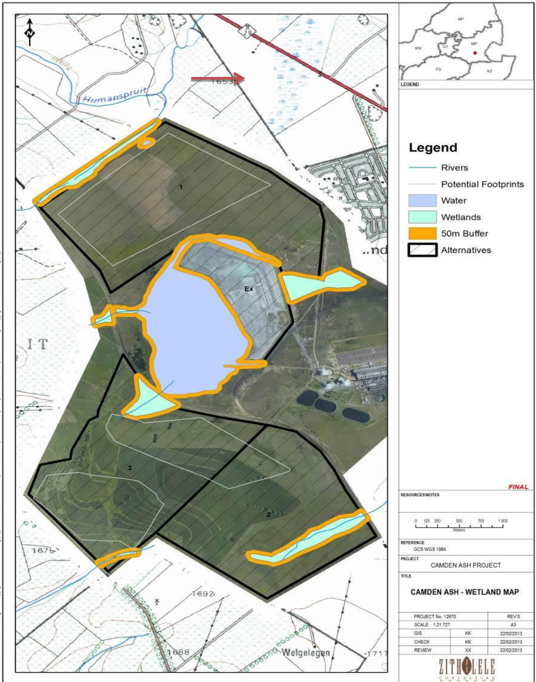
Figure 2: Previously mapped wetlands (Zitholele, 2013)
