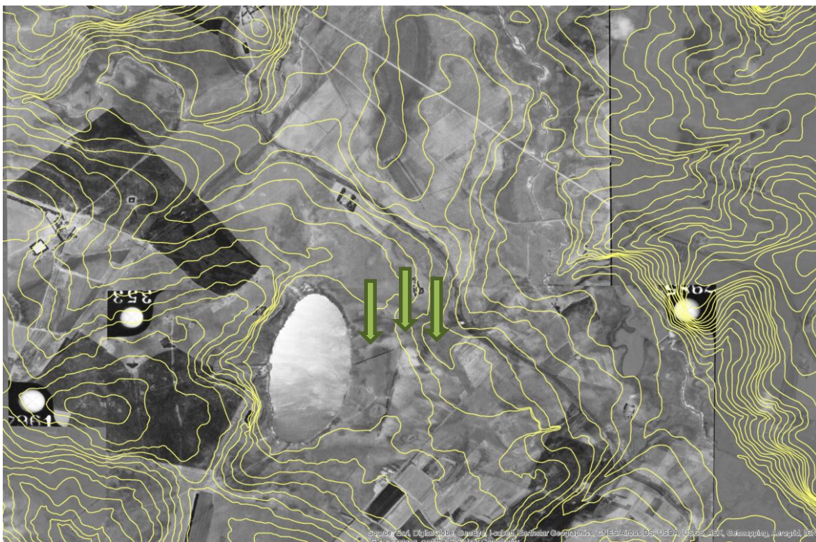
Figure 3: Historical imagery (1955 predating construction of the power station, indicating De Jagers Pan and wetland areas to the East in proximity to the current ash facility)
