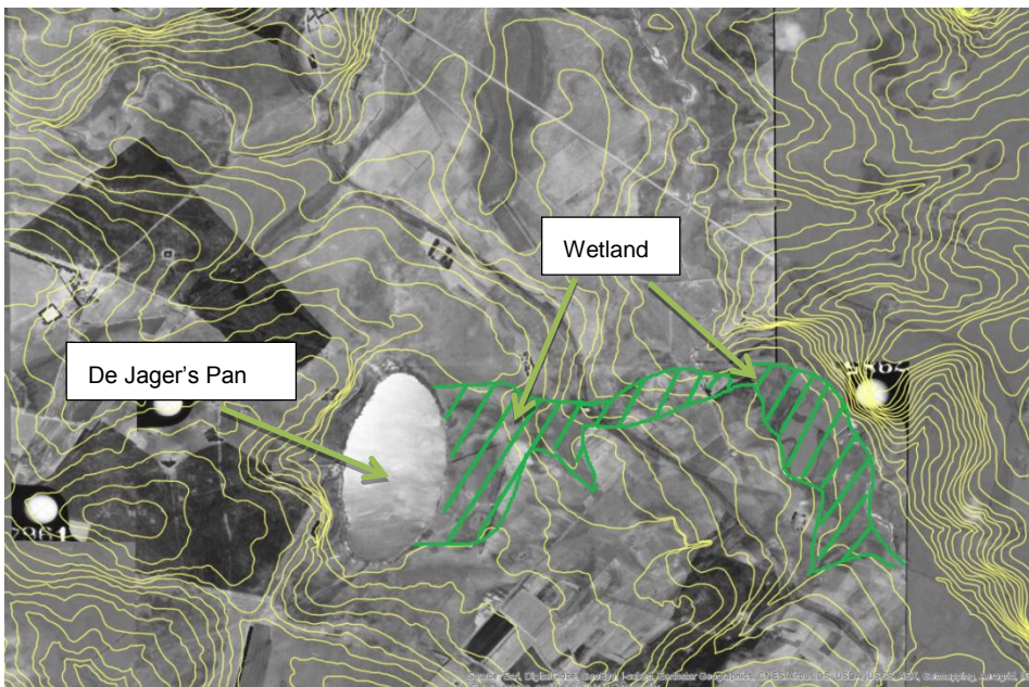
A. Historic aerial imagery showing wetland area east of De Jager's pan prior to construction of power plant and ash facility
