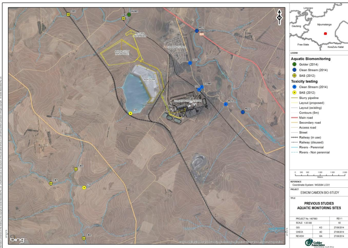
Figure 4: Aquatic sampling sites sampled in January 2012, March 2014 and July 2014
