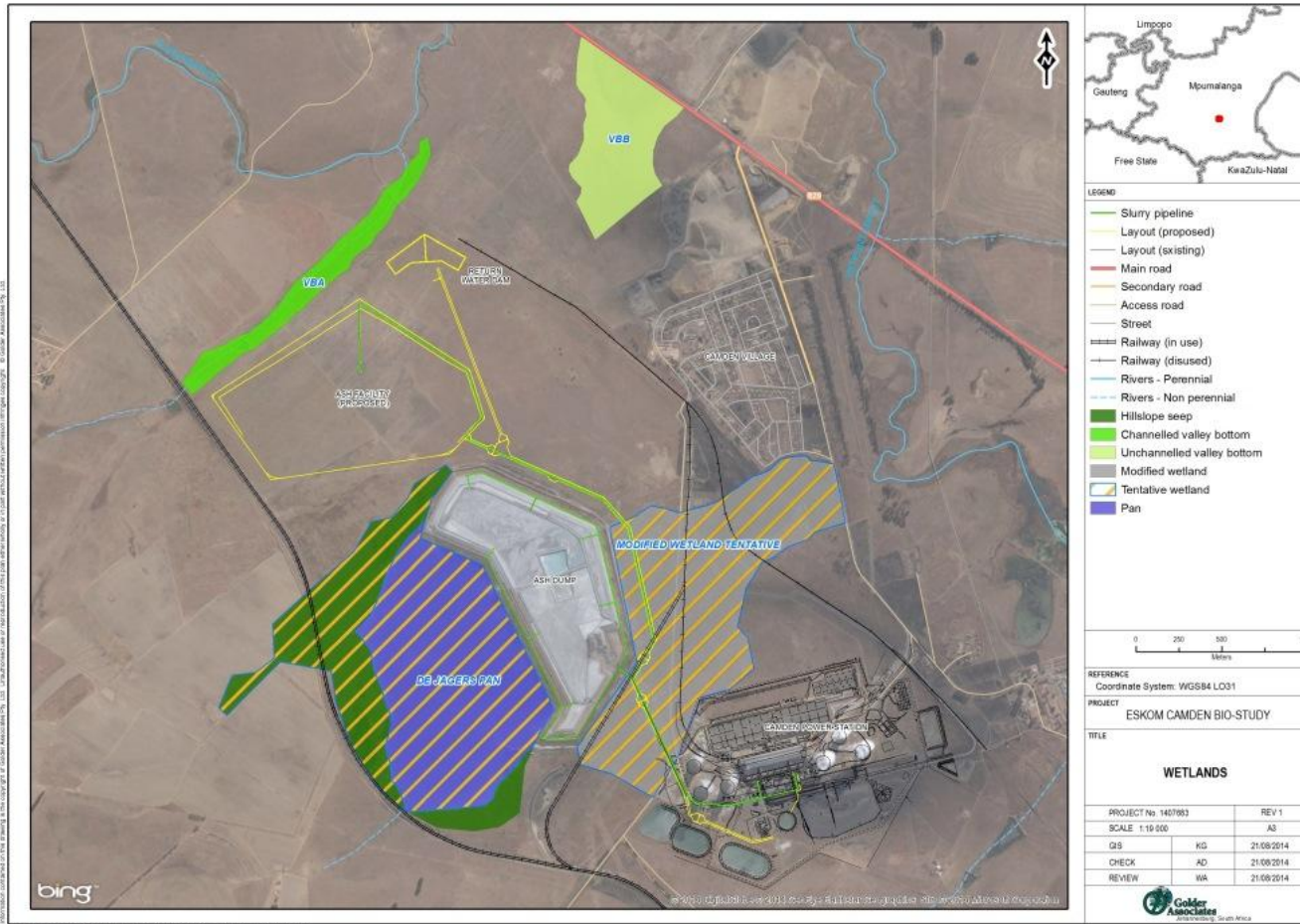
Figure 9: Wetlands in relation to preferred Site 1 ash disposal facility footprint
