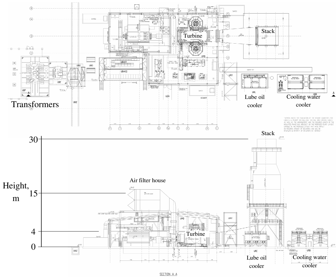
FIGURE 3 Example of two OCGT power generation units
