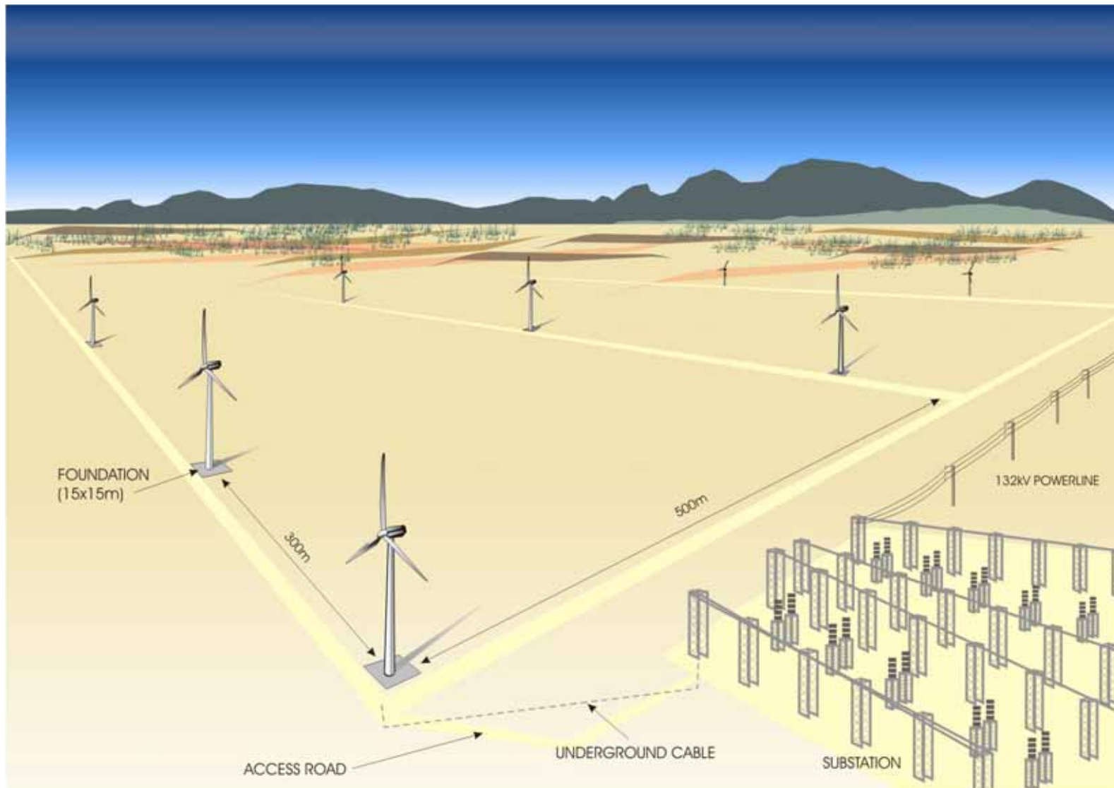
Figure 7.8: Artists impression of a portion of a wind energy facility, illustrating the various components and associated infrastructure
