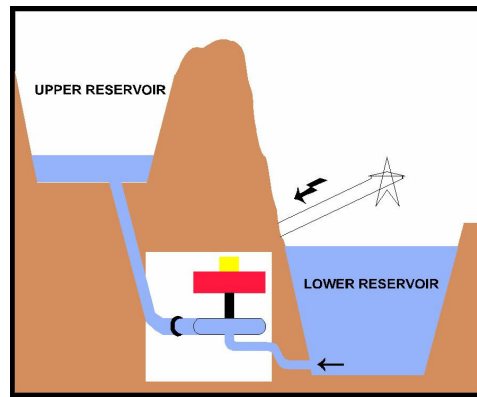
PUMPING CYCLE
