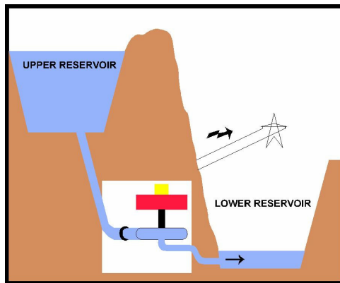
GENERATION CYCLE
