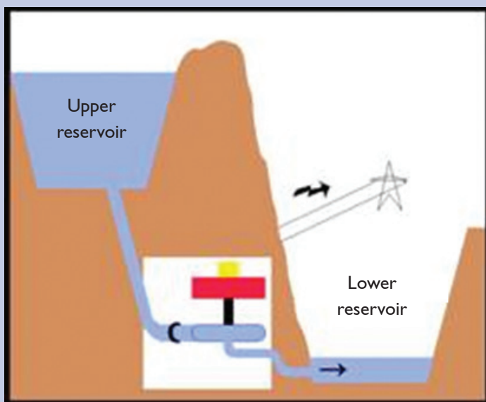
Generation cycle
