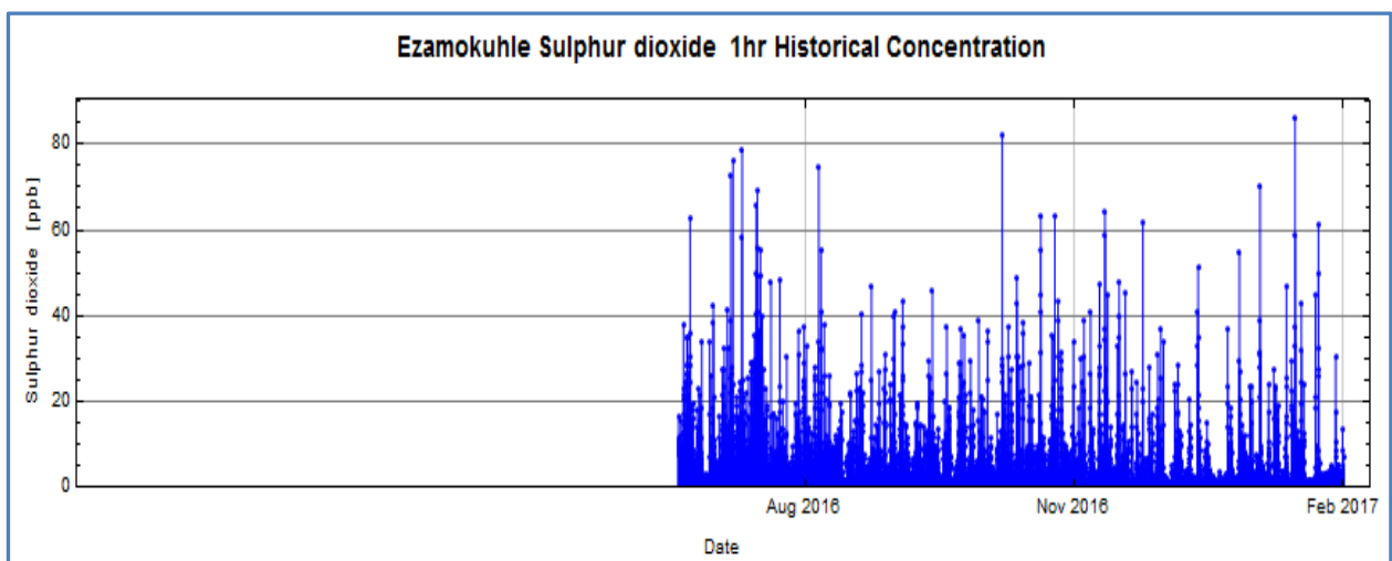
Figure 15: Time series graph for SO 2 hourly data from July 2016 to February 2017
