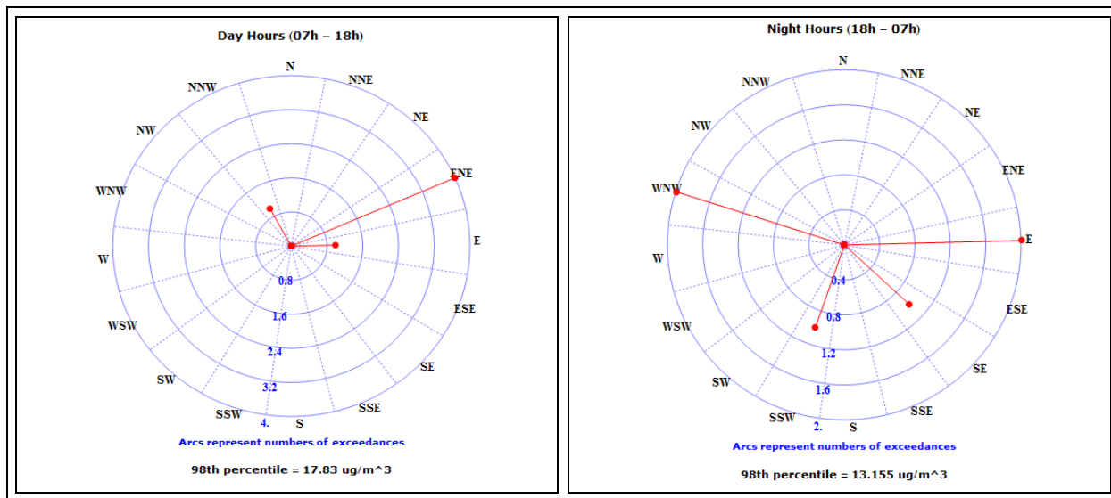
Figure 4: PM 10 hourly mean 98 th percentile event roses during day and night times
