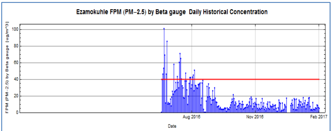
Figure 18: Time series graph for PM 2.5 daily data from July 2016 to February 2017
