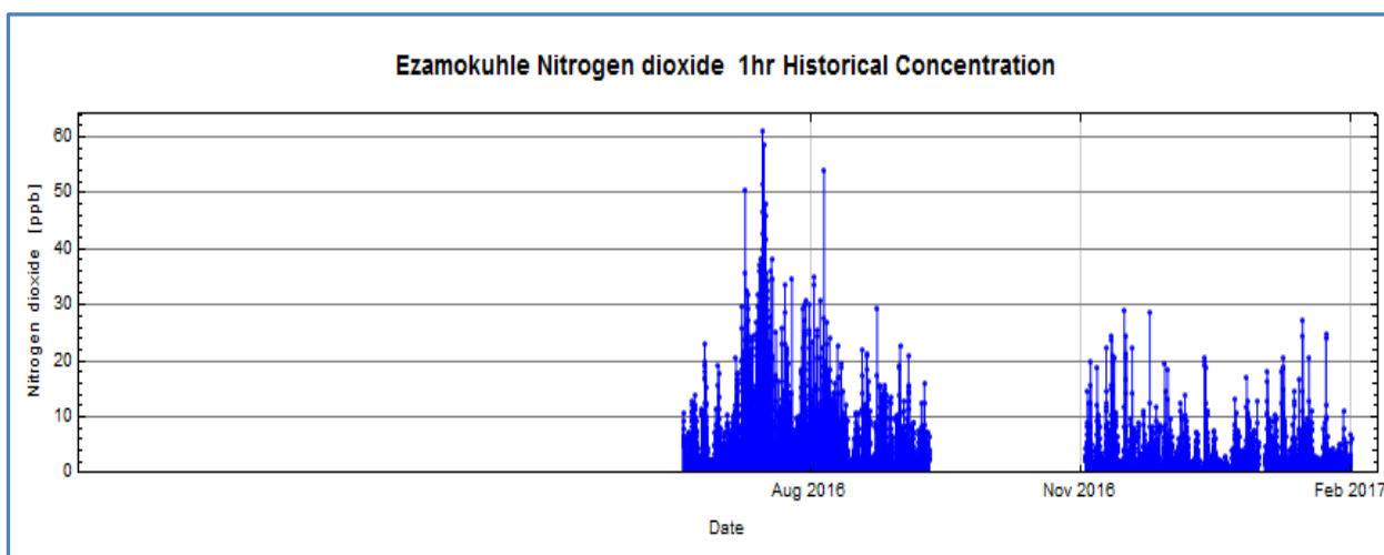
Figure 19: Time series graph for NO 2 hourly data from July 2016 to February 2017
