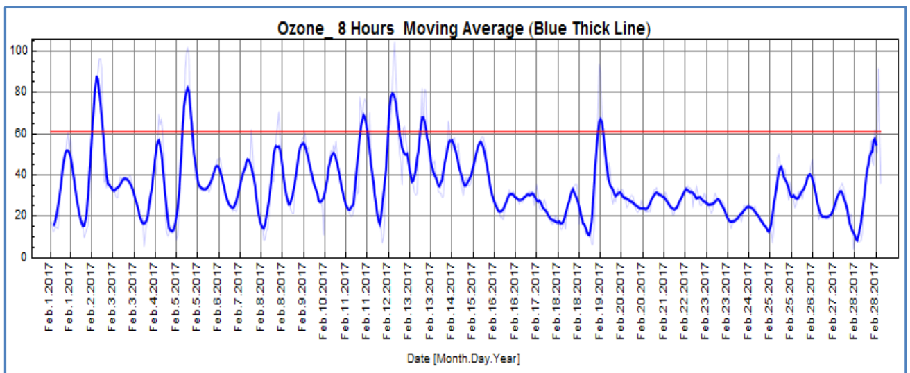
Figure 13: O 3 8 Hours Moving Average (Blue Thick Line)
