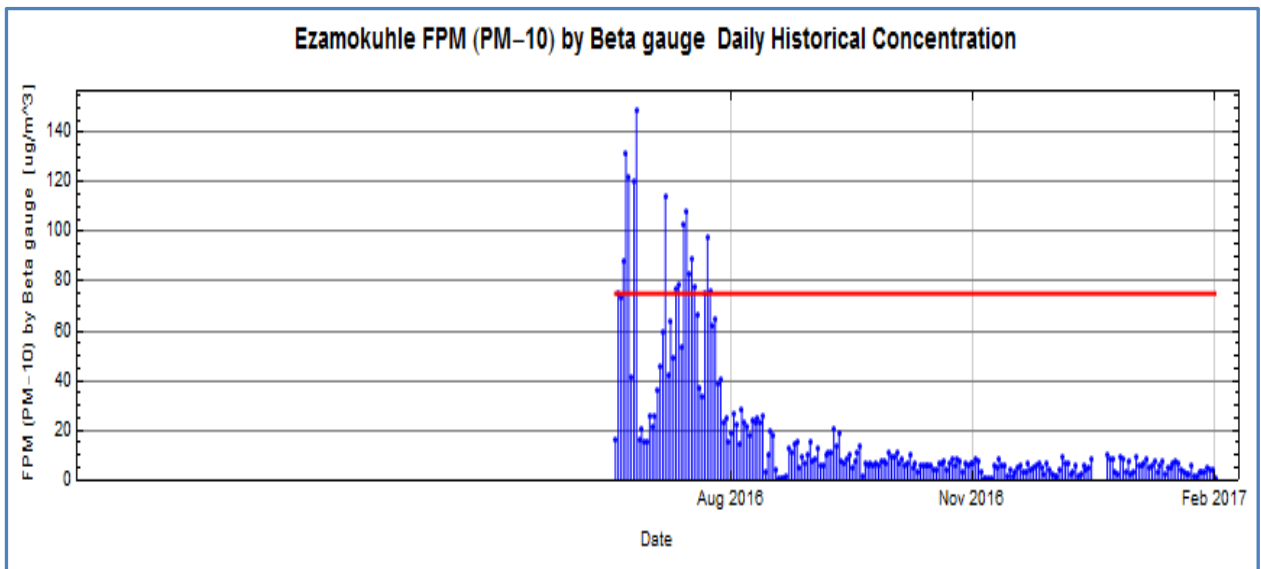
Figure 17: Time series graph for PM 10 daily data from July 2016 to February 2017
