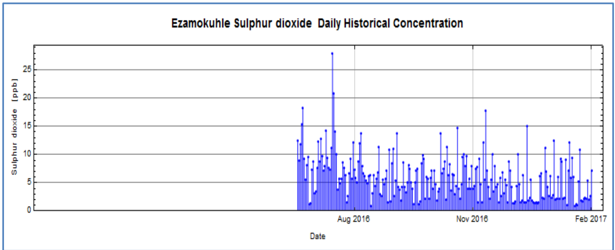
Figure 16: Time series graph for SO 2 daily data from July 2016 to February 2017
