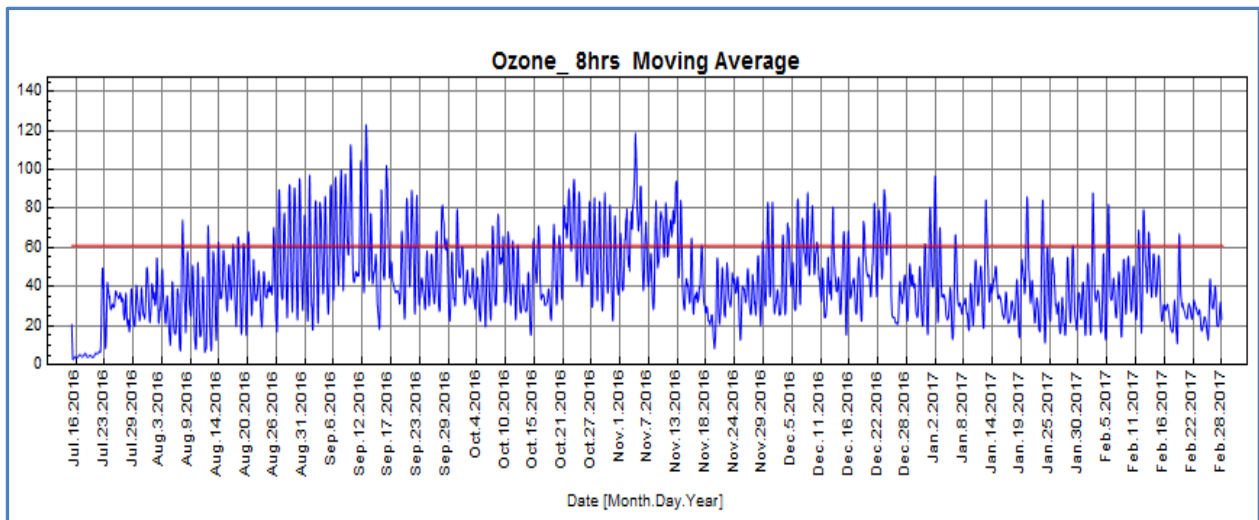
Figure 14: Historical ozone 8 hours moving average from July 2016 to February 2017
