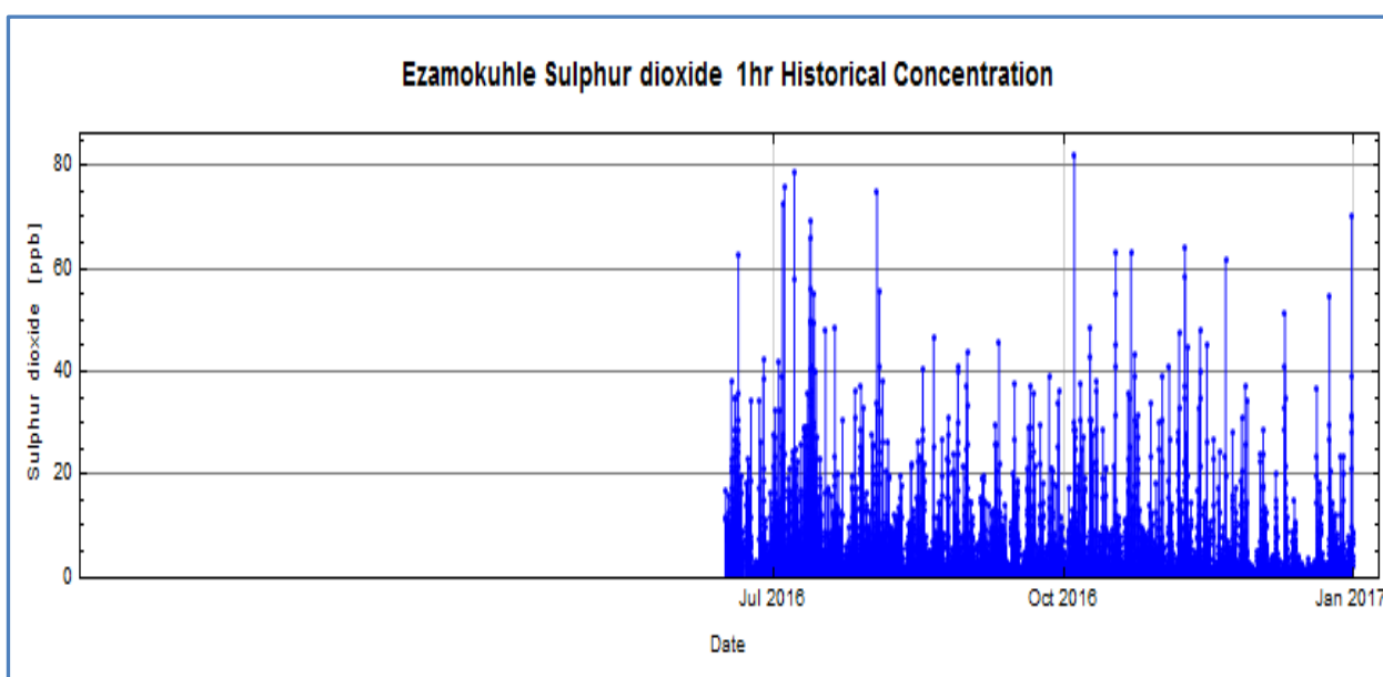
Figure 15: Time series graph for SO 2 hourly data from July 2016 to January 2017
