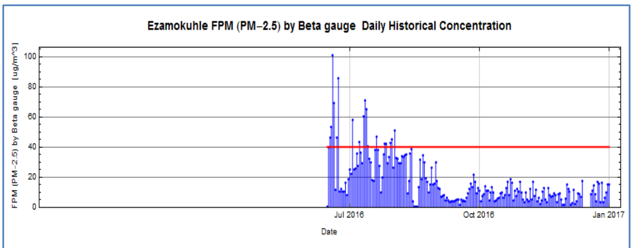
Figure 18: Time series graph for PM 2.5 daily data from July 2016 to January 2017
