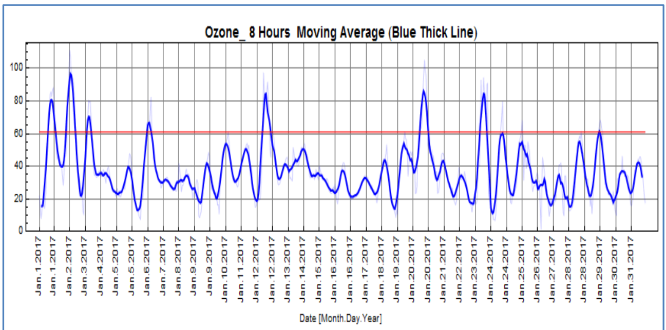
Figure 13: O 3 8 Hours Moving Average (Blue Thick Line)
