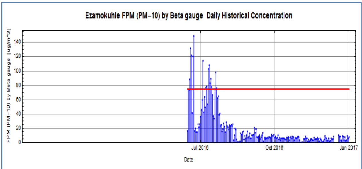
Figure 17: Time series graph for PM 10 daily data from July 2016 to January 2017
