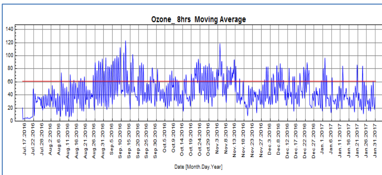
Figure 14: Historical ozone 8 hours moving average from July 2016 to January 2017
