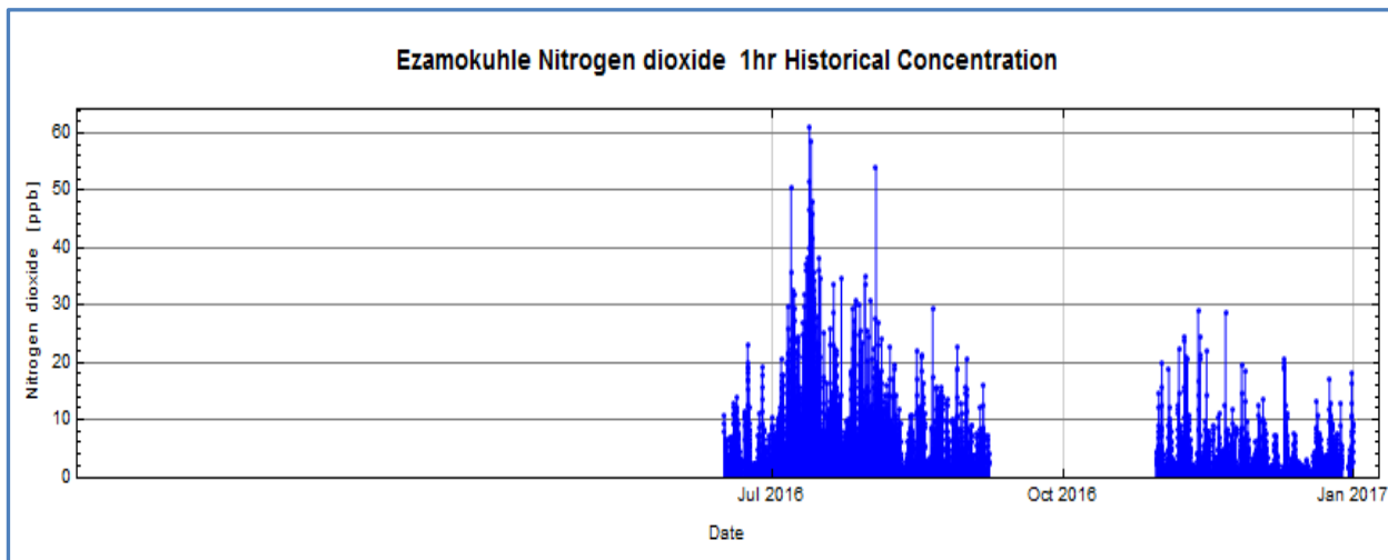
Figure 19: Time series graph for NO 2 hourly data from July 2016 to January 2017
