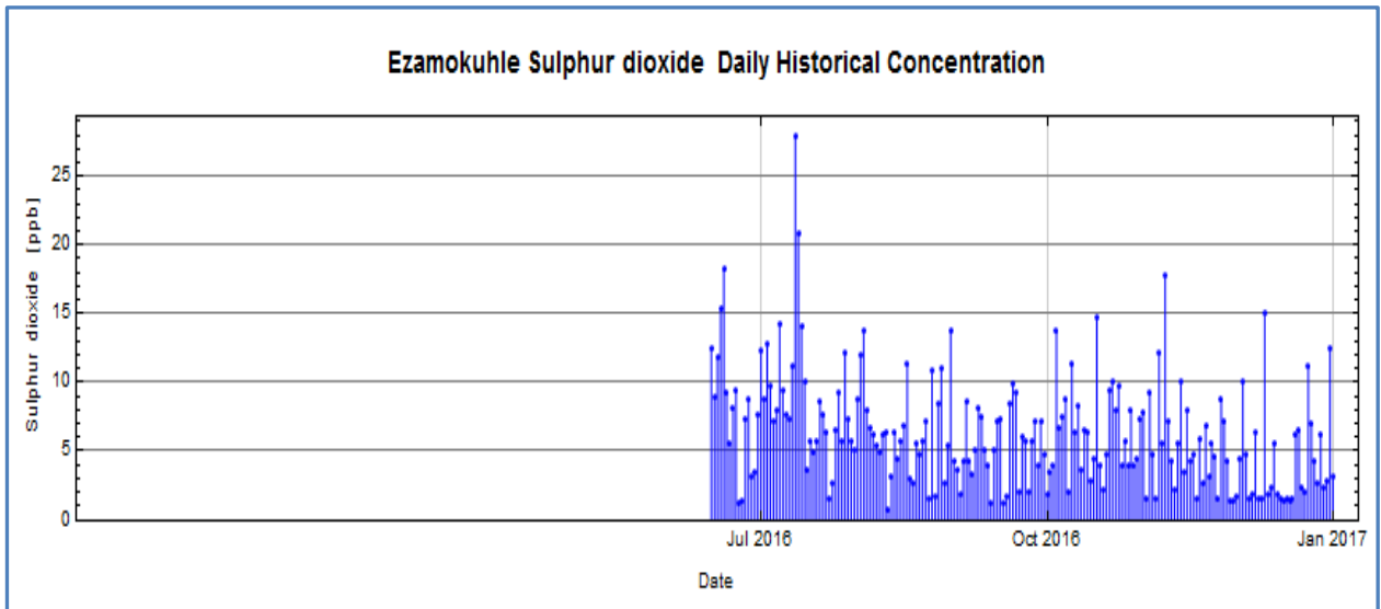
Figure 16: Time series graph for SO 2 daily data from July 2016 to January 2017
