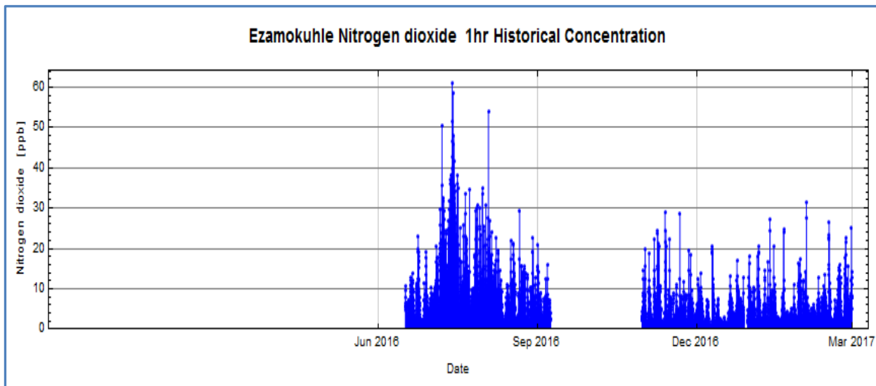
Figure 19: Time series graph for NO 2 hourly data from July 2016 to March 2017
