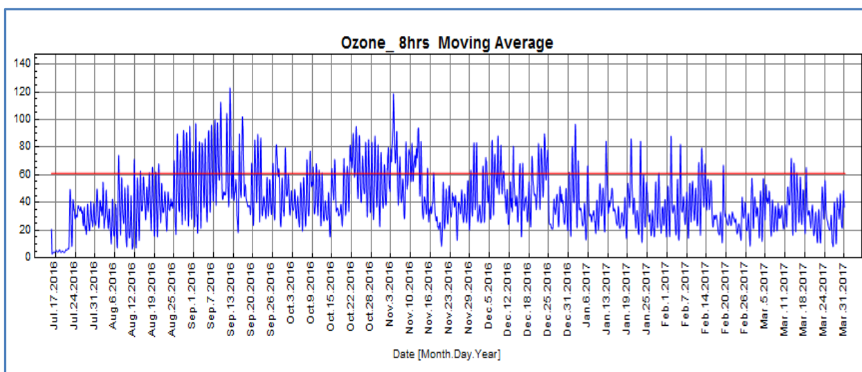
Figure 14: Historical ozone 8 hours moving average from July 2016 to March 2017
