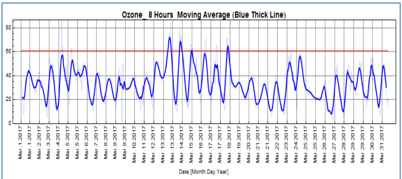
Figure 13: O 3 8 Hours Moving Average (Blue Thick Line)
