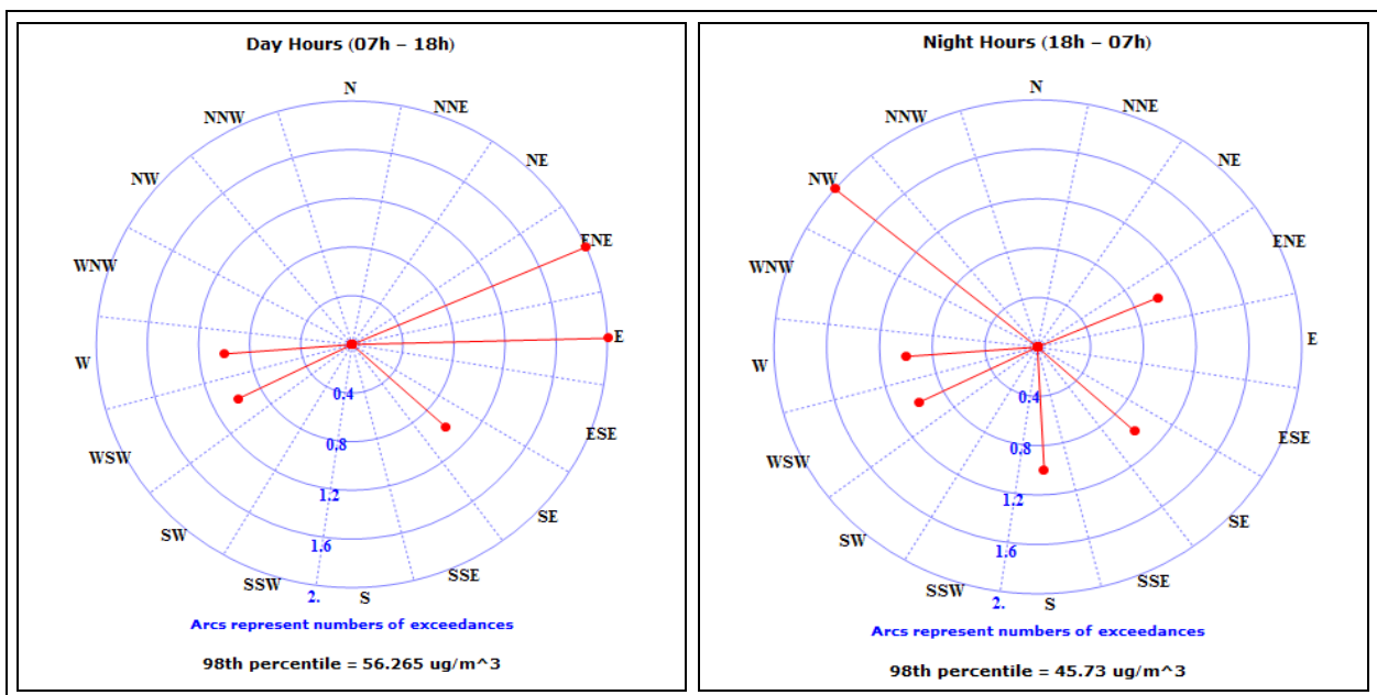
Figure 6: PM 2.5 hourly mean 98 th percentile event roses during day and night times
