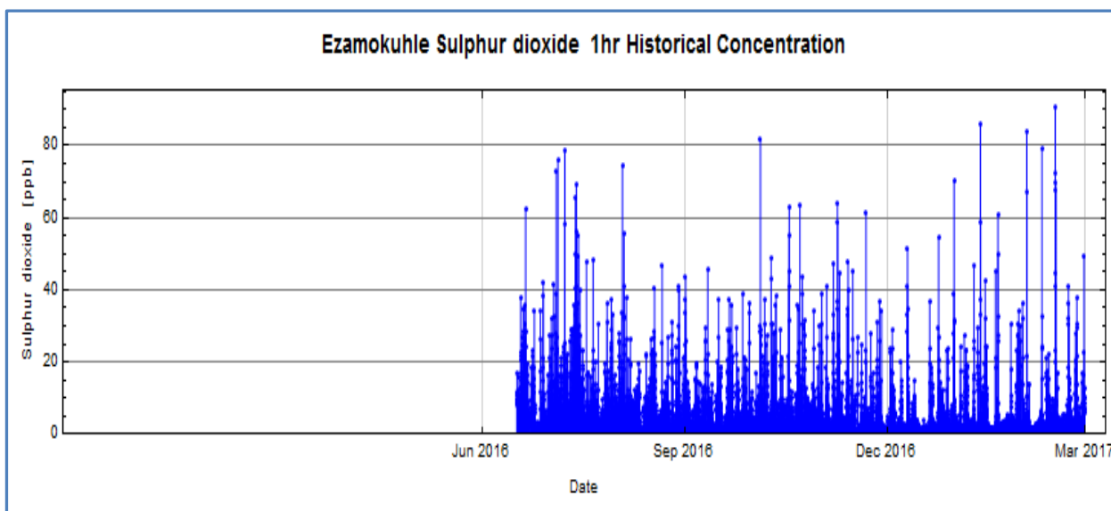
Figure 15: Time series graph for SO 2 hourly data from July 2016 to March 2017
