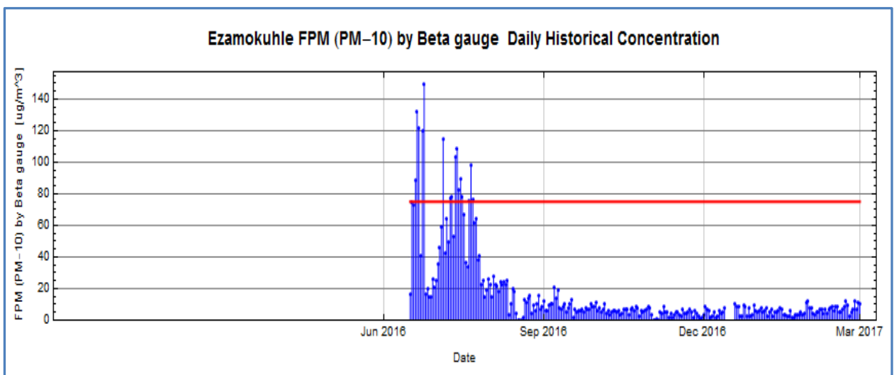
Figure 17: Time series graph for PM 10 daily data from July 2016 to March 2017
