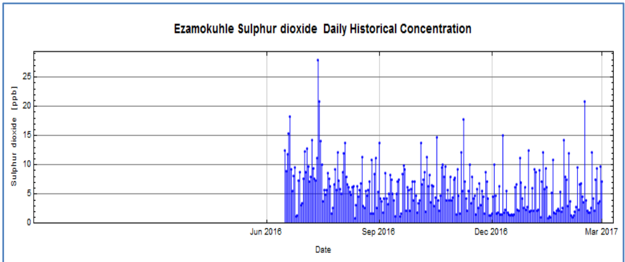
Figure 16: Time series graph for SO 2 daily data from July 2016 to March 2017
