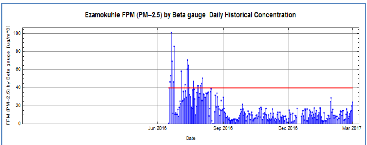
Figure 18: Time series graph for PM 2.5 daily data from July 2016 to March 2017
