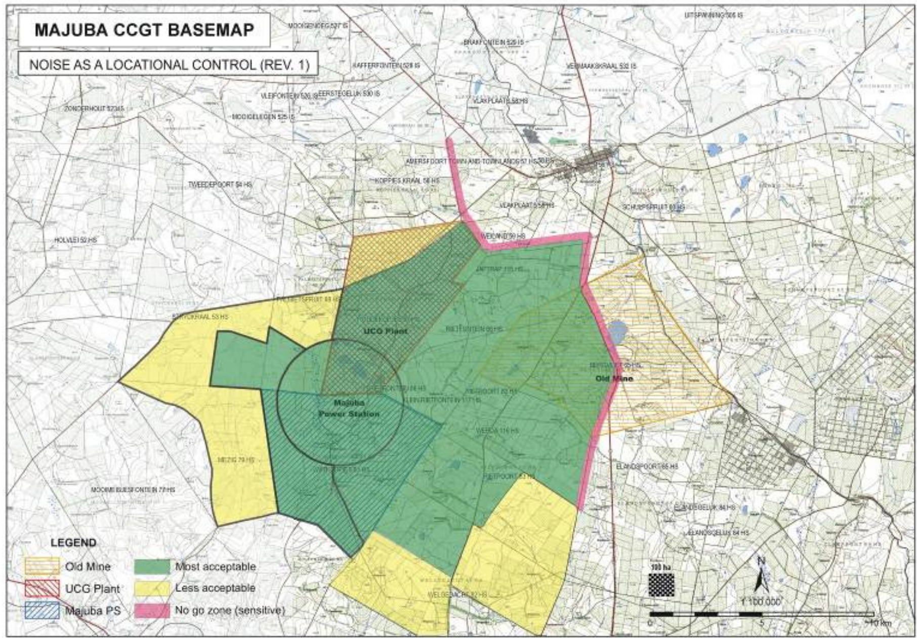
Figure 5 Sensitivity map showing areas that are ideal, acceptable and sensitive in terms of noise impacts.
