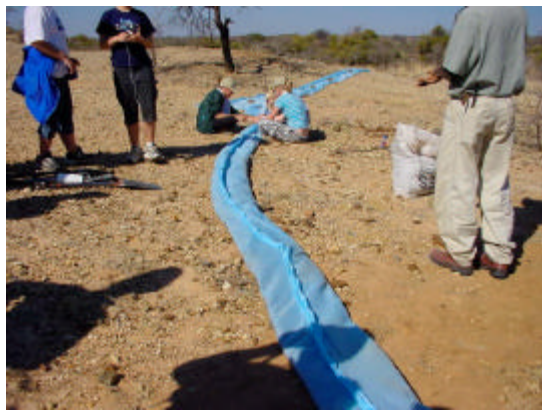
Figure 8. The photo's show the mixing of the soil, the manure seed and silicate mineral before placing it in the geotextile bags.
