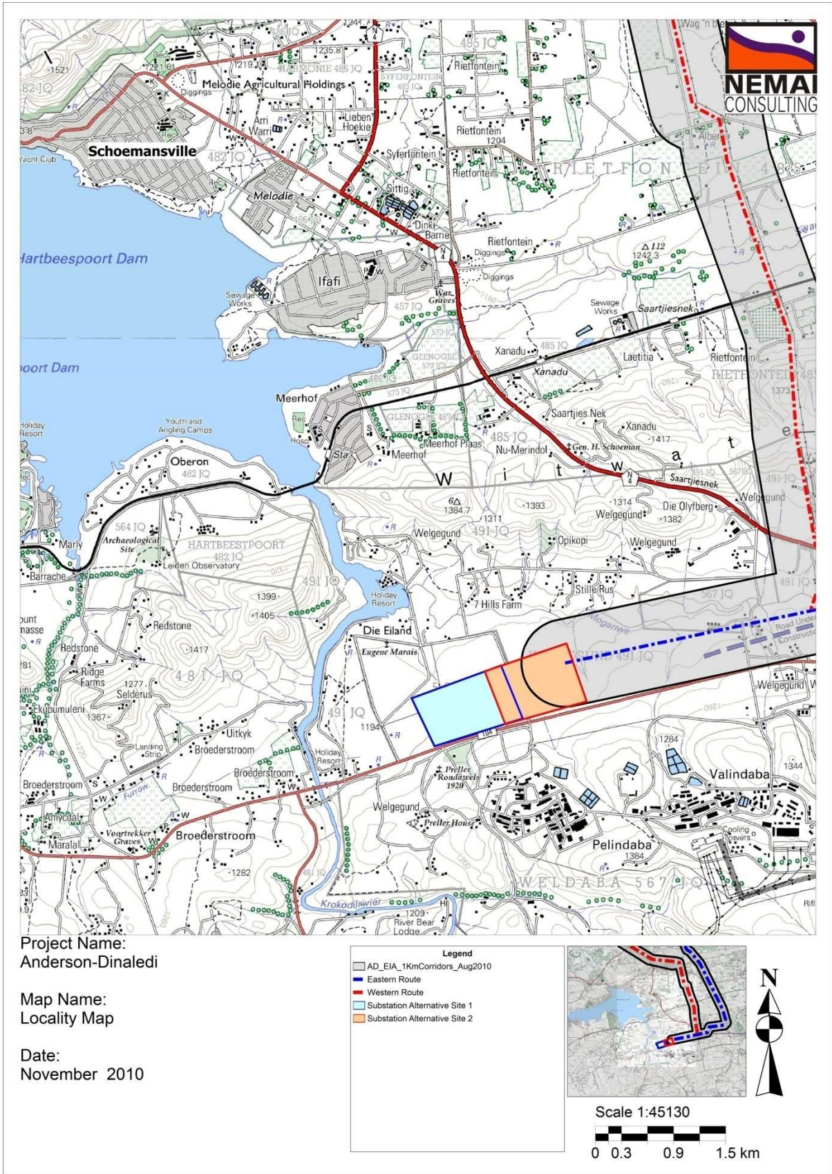
Figure 3: Substation Alternative Sites
