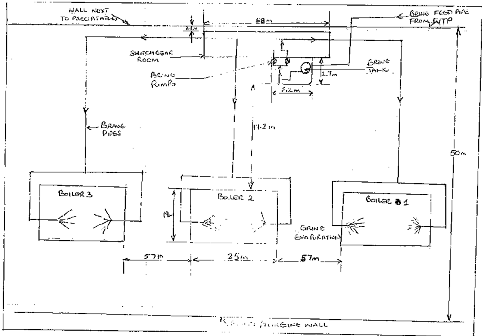
Figure 1.2 Location of existing infrastructure for evaporation in boilers 1 - 3
