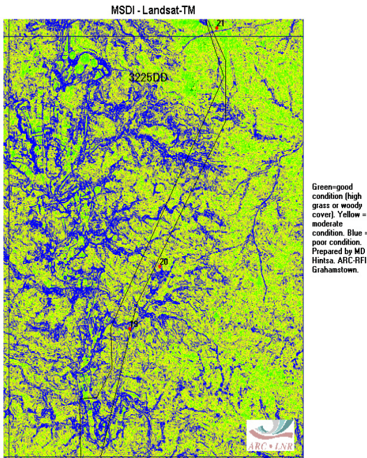
Plate 10. Landsat TM MSDI for 1:50 000 Topo Series Sheet 3225DD, showing the existing and proposed transmission lines and field sampling sites.
