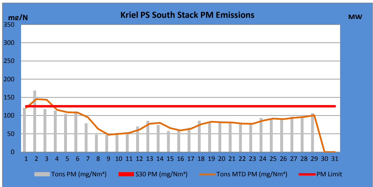
Figure 2: PM emissions (daily averages) for the month of April 2018 against emission limit for the South Stack
