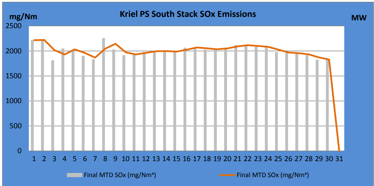
Figure 5. SO 2 emissions (daily averages) for the month of April 2018 against emission limit for the South Stack. SO x permitted maximum release rate is 3 500mg/Nm 3
