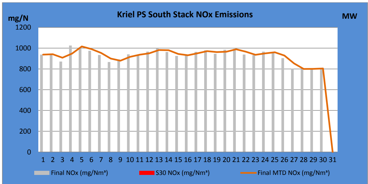
Figure 6. NO 2 emissions (daily averages) for the month of April 2018 against emission limit for the South Stack. NO x permitted maximum release rate is 1 600mg/Nm 3
