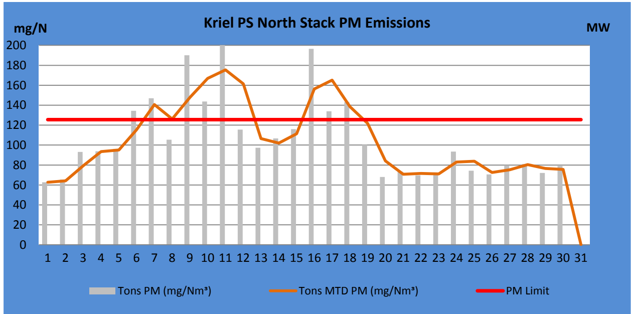
Figure 1: PM emissions (daily averages) for the month of April 2018 against emission limit for the North Stack
