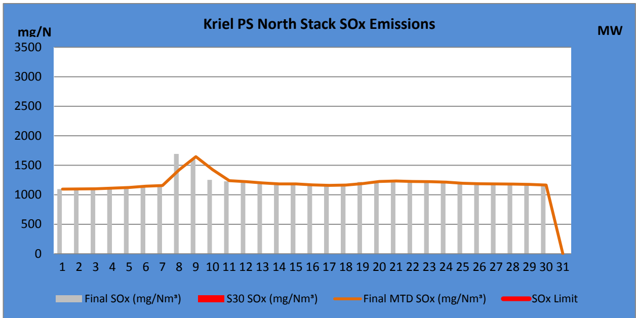
Figure 3. SO 2 emissions (daily averages) for the month of April 2018 against emission limit for the North Stack. SO x permitted maximum release rate is 3 500mg/Nm 3
