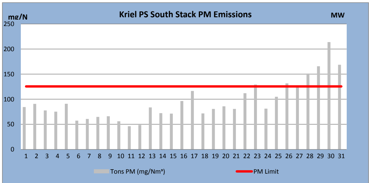
Figure 2: PM emissions (daily averages) for the month of August 2018 against emission limit for the South Stack
