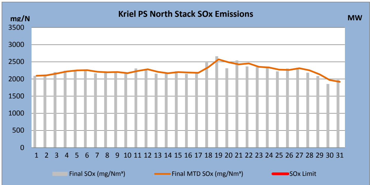
Figure 3. SO 2 emissions (daily averages) for the month of August 2018 against emission limit for the North Stack. SO x permitted maximum release rate is 3 500mg/Nm 3
