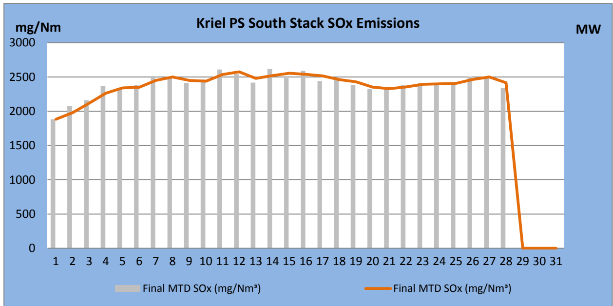
Figure 5. SO 2 emissions (daily averages) for the month of February 2018 against emission limit for the South Stack. SO x permitted maximum release rate is 3 500mg/Nm 3 .
