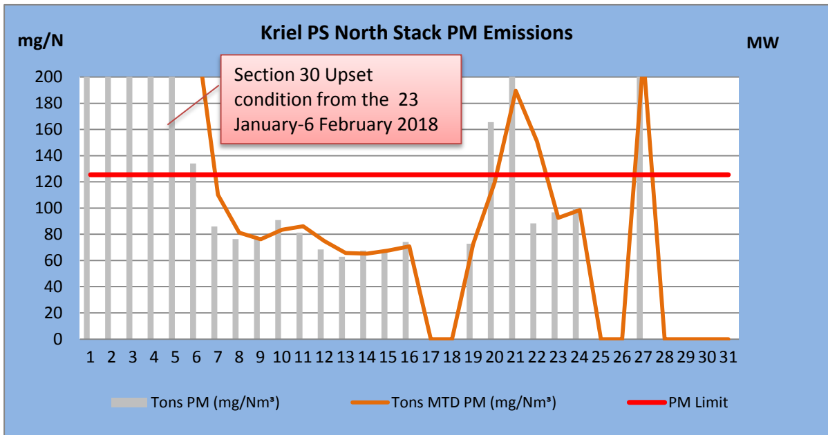
Figure 1: PM emissions (daily averages) for the month of February 2018 against emission limit for the North Stack
