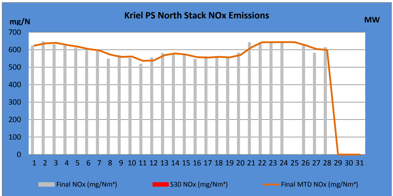
4. NO 2 emissions (daily averages) for the month of February 2018 against emission limit for the North Stack. NO x permitted maximum release rate is 1 600mg/Nm 3
