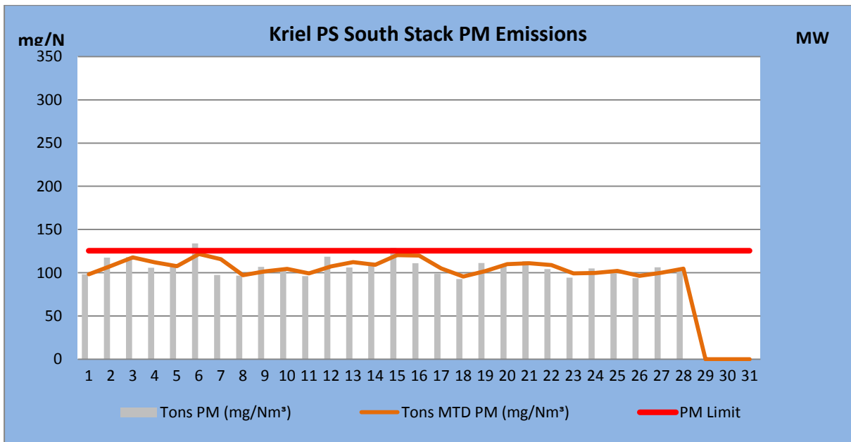
Figure 2: PM emissions (daily averages) for the month of February 2018 against emission limit for the South Stack
