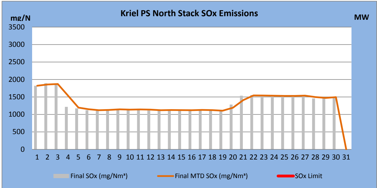
Figure 3. SO 2 emissions (daily averages) for the month of June 2018 against emission limit for the North Stack. SO x permitted maximum release rate is 3 500mg/Nm 3
