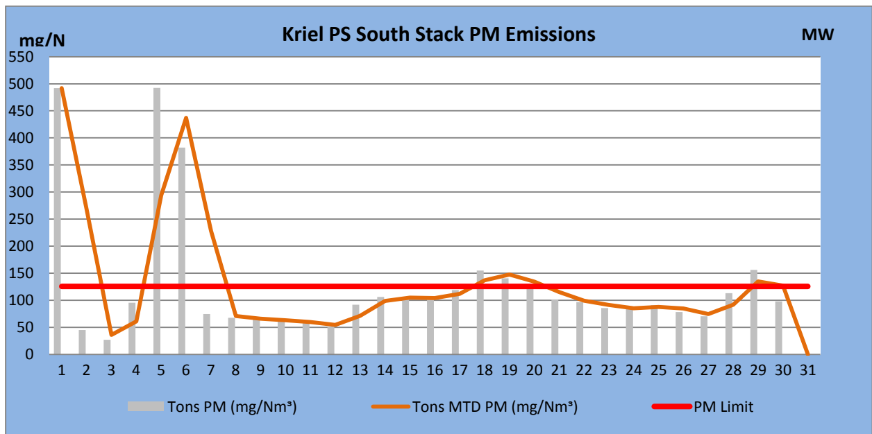
Figure 2: PM emissions (daily averages) for the month of June 2018 against emission limit for the South Stack
