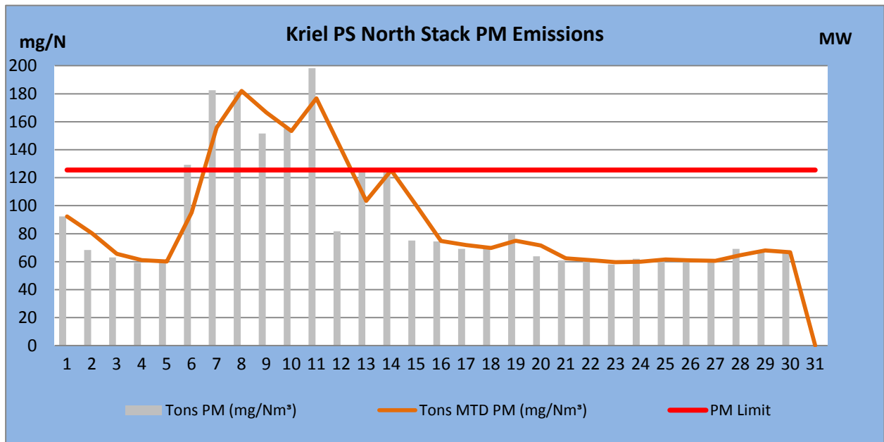
Figure 1: PM emissions (daily averages) for the month of June 2018 against emission limit for the North Stack
