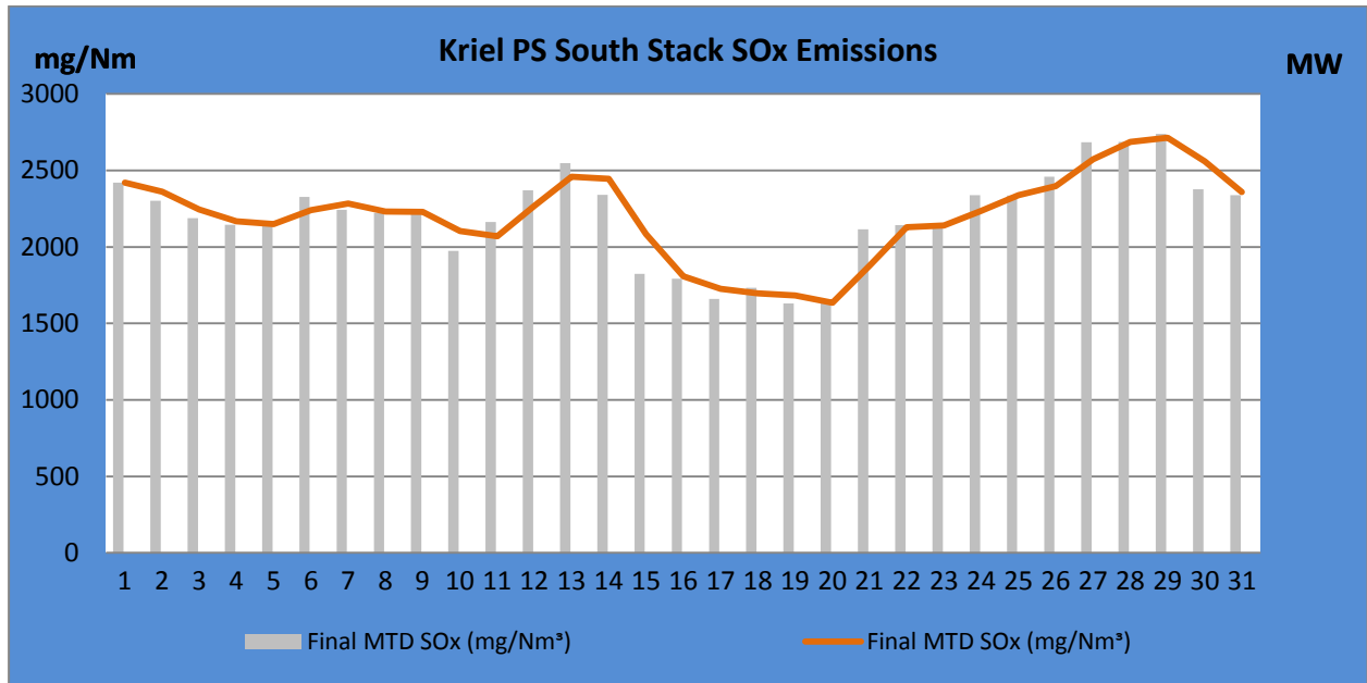
Figure 5. SO 2 emissions (daily averages) for the month of March 2018 against emission limit for the South Stack. . SO x permitted maximum release rate is 3 500mg/Nm 3
