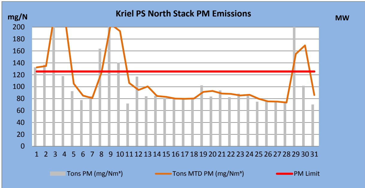
Figure 1: PM emissions (daily averages) for the month of March 2018 against emission limit for the North Stack
