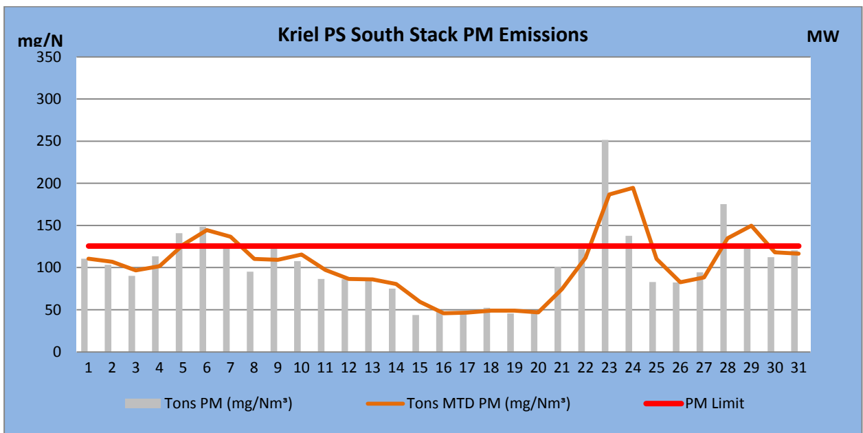
Figure 2: PM emissions (daily averages) for the month of March 2018 against emission limit for the South Stack
