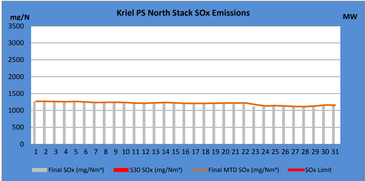
Figure 3. SO 2 emissions (daily averages) for the month of March 2018 against emission limit for the North Stack. SO x permitted maximum release rate is 3 500mg/Nm 3
