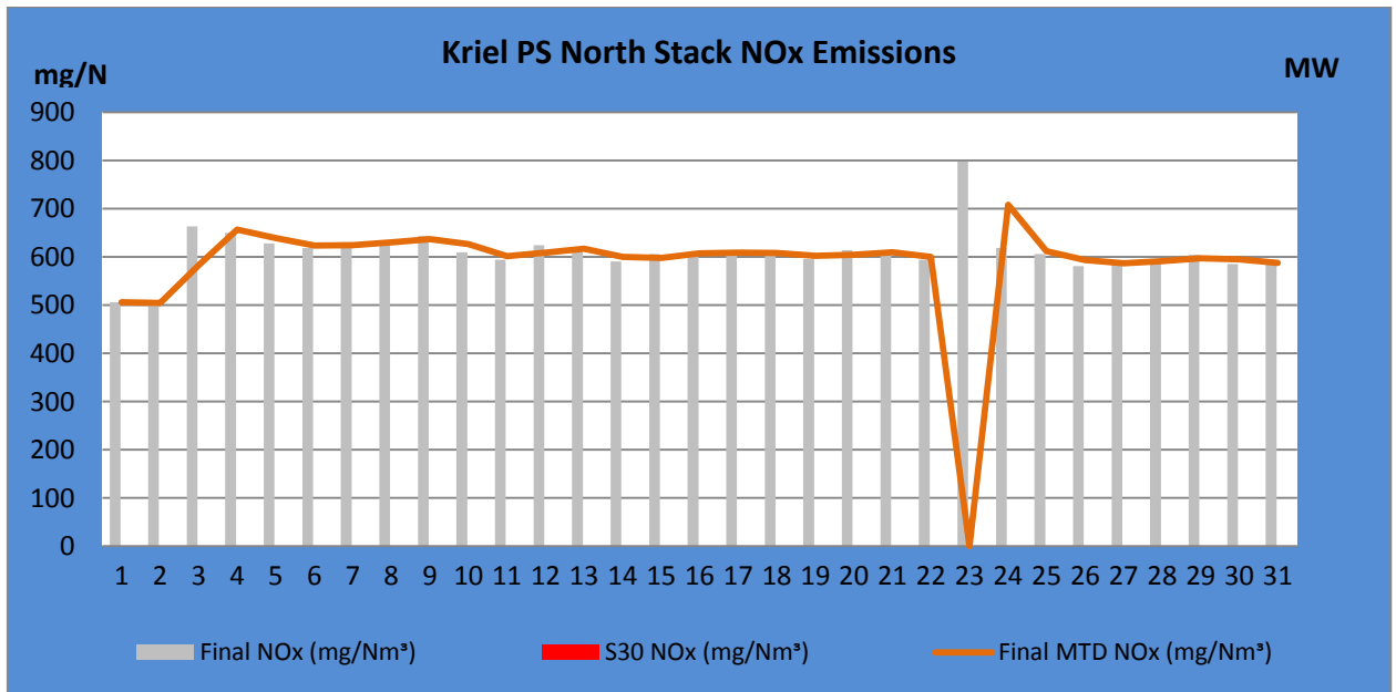
4. NO 2 emissions (daily averages) for the month of March 2018 against emission limit for the North Stack. NO x permitted maximum release rate is 1 600mg/Nm 3
