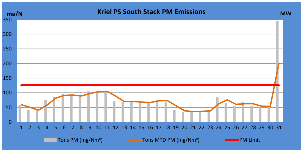
Figure 2: PM emissions (daily averages) for the month of May 2018 against emission limit for the South Stack
