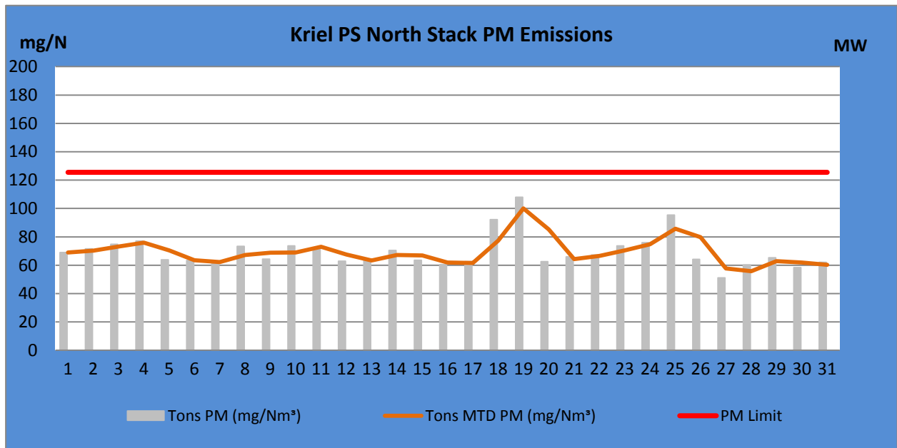
Figure 1: PM emissions (daily averages) for the month of May 2018 against emission limit for the North Stack
