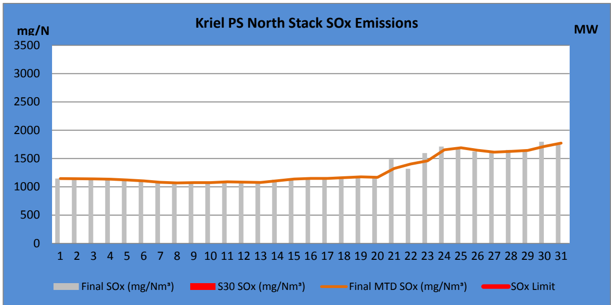
Figure 3. SO 2 emissions (daily averages) for the month of May 2018 against emission limit for the North Stack. SO x permitted maximum release rate is 3 500mg/Nm 3
