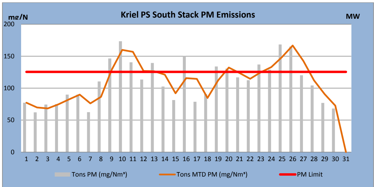
Figure 2: PM emissions (daily averages) for the month of November 2018 against emission limit for the South Stack
