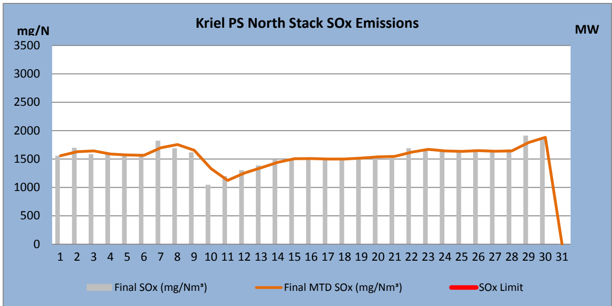
Figure 3. SO 2 emissions (daily averages) for the month of November 2018 against emission limit for the North Stack. SO x permitted maximum release rate is 3 500mg/Nm 3
