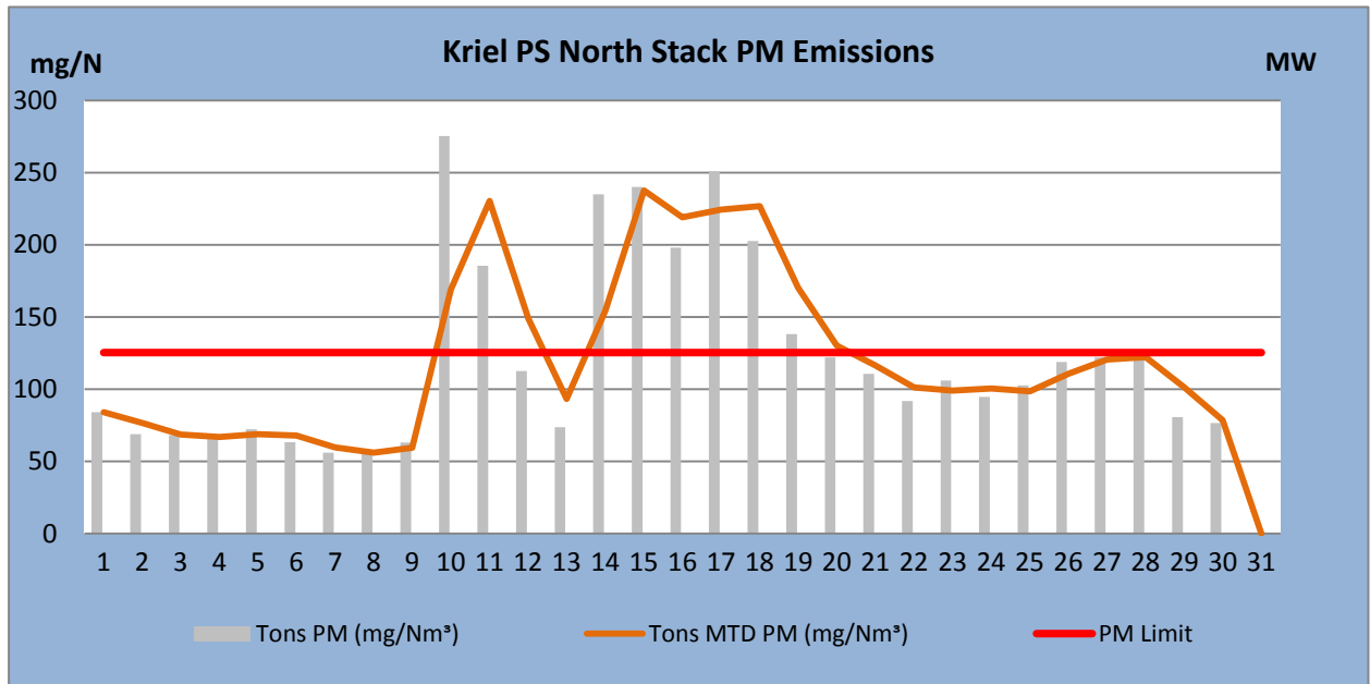
Figure 1: PM emissions (daily averages) for the month of November 2018 against emission limit for the North Stack
