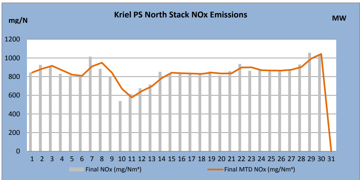
4. NO 2 emissions (daily averages) for the month of November 2018 against emission limit for the North Stack. NO x permitted maximum release rate is 1 600mg/Nm 3
