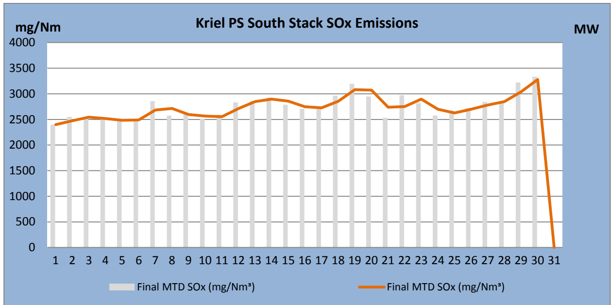
Figure 5. SO 2 emissions (daily averages) for the month of November 2018 against emission limit for the South Stack. SO x permitted maximum release rate is 3 500mg/Nm 3
