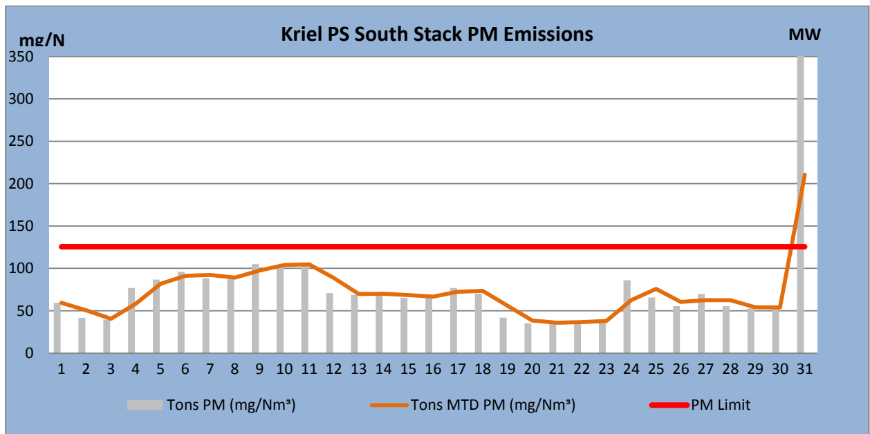
Figure 2: PM emissions (daily averages) for the month of October 2018 against emission limit for the South Stack
