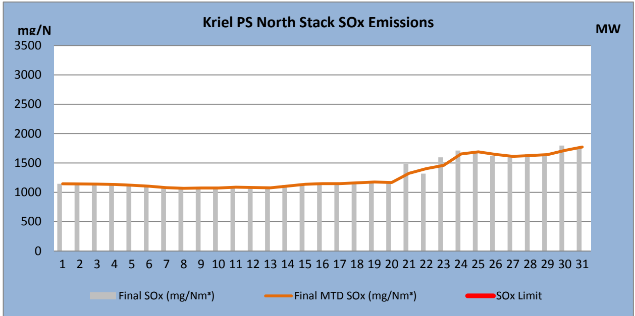
Figure 3. SO 2 emissions (daily averages) for the month of October 2018 against emission limit for the North Stack. SO x permitted maximum release rate is 3 500mg/Nm 3
