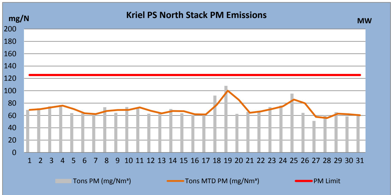
Figure 1: PM emissions (daily averages) for the month of October 2018 against emission limit for the North Stack
