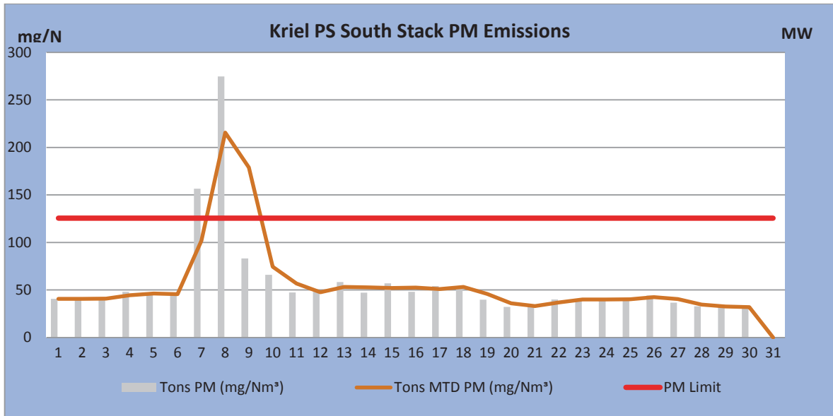
Figure 2: PM emissions (daily averages) for the month of April 2019 against emission limit for the South Stack
