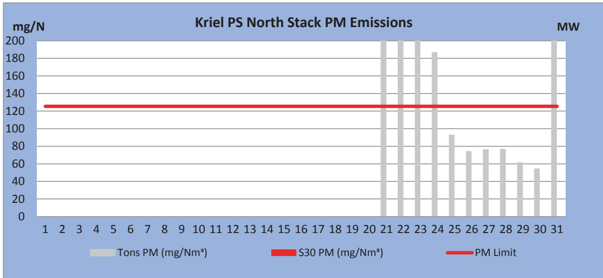
Figure 1: PM emissions (daily averages) for the month of January 2019 against emission limit for the North Stack
