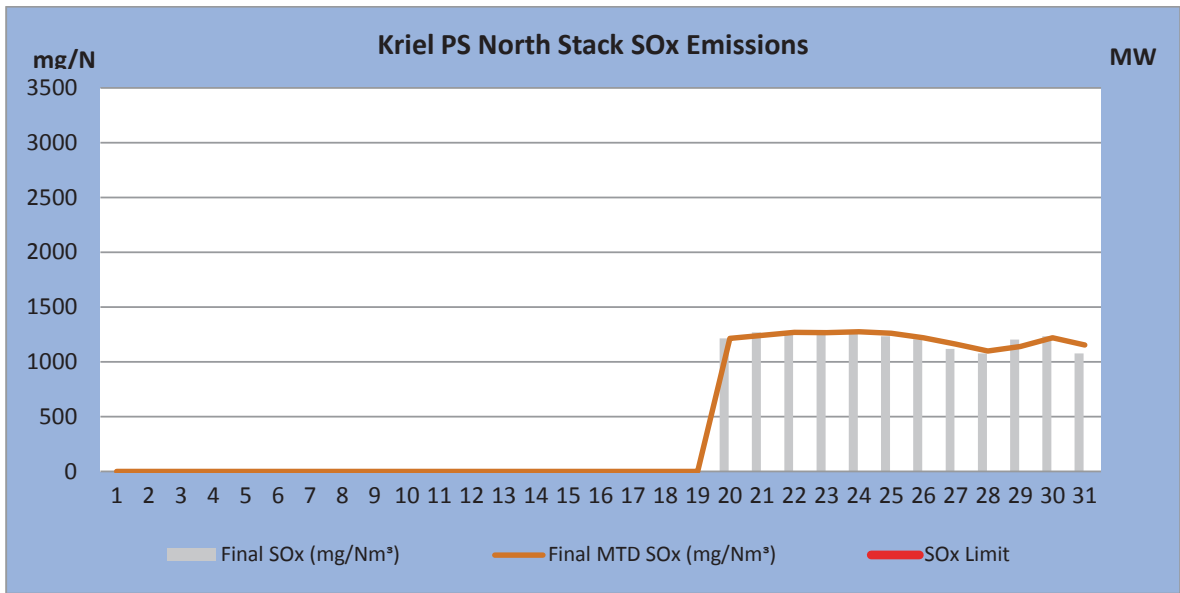
Figure 3. SO 2 emissions (daily averages) for the month of January 2019 against emission limit for the North Stack. SO x permitted maximum release rate is 3 500mg/Nm 3
