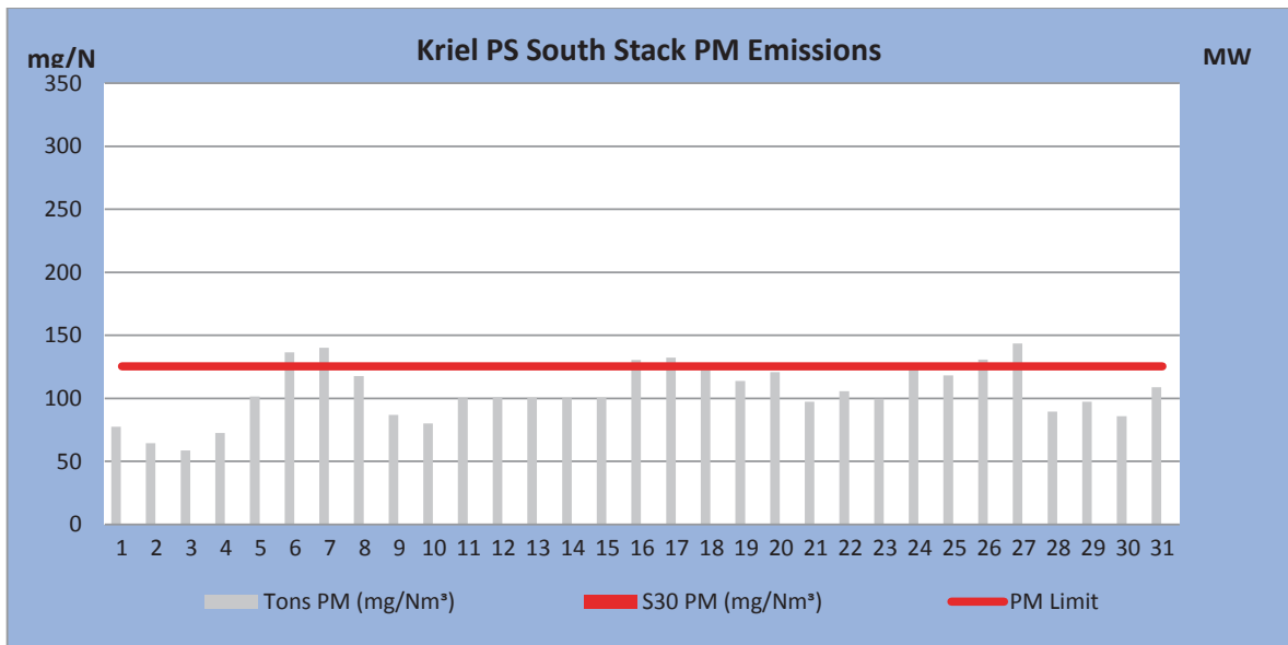
Figure 2: PM emissions (daily averages) for the month of January 2019 against emission limit for the South Stack
