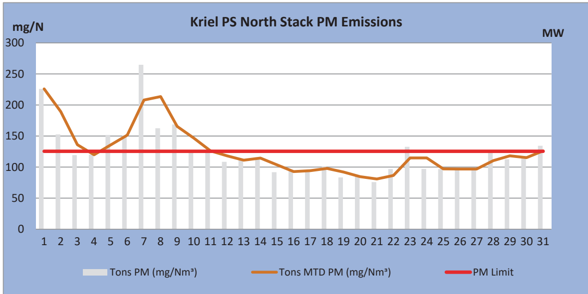
Figure 1: PM emissions (daily averages) for the month of July 2019 against emission limit for the North Stack
