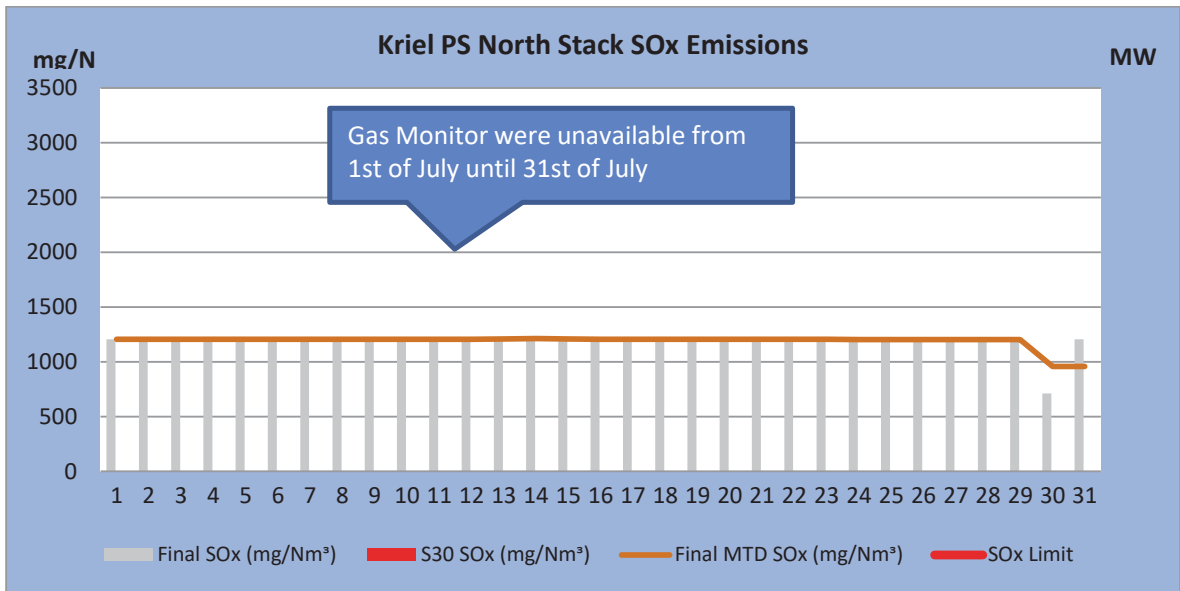
Figure 3. SO 2 emissions (daily averages) for the month of July 2019 against emission limit for the North Stack. SO x permitted maximum release rate is 3 500mg/Nm 3
