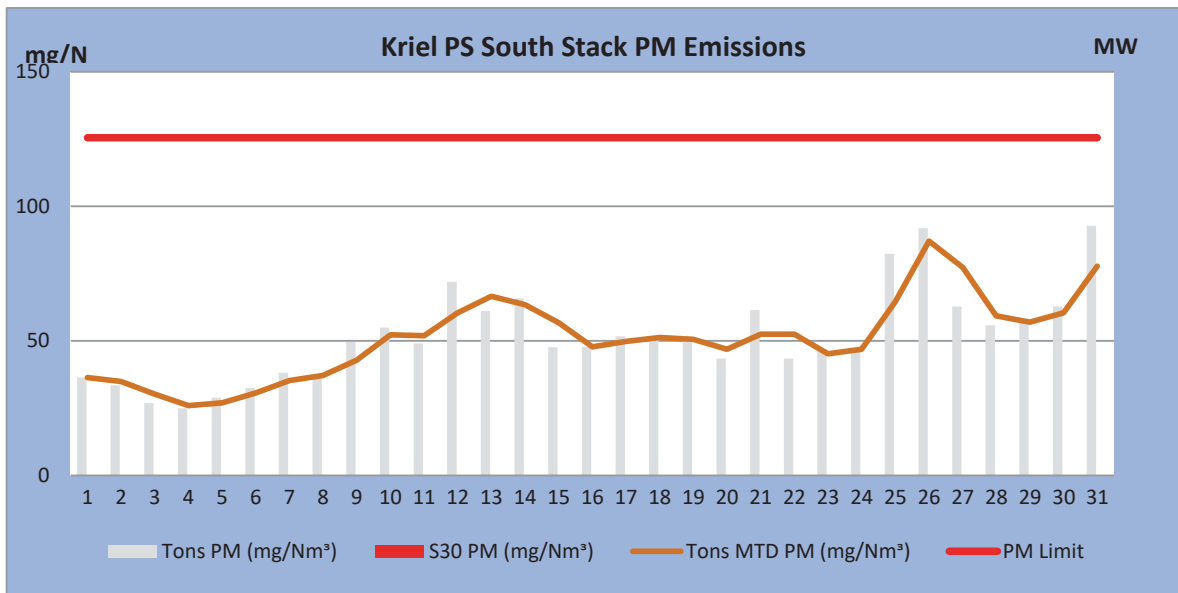
Figure 2: PM emissions (daily averages) for the month of July 2019 against emission limit for the South Stack
