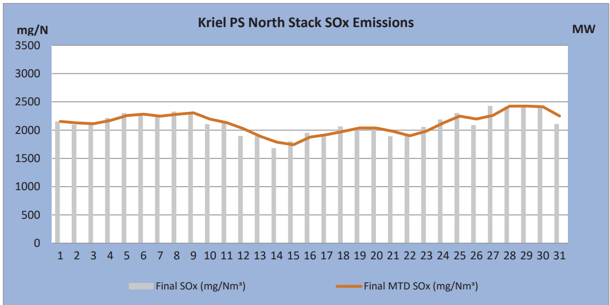
Figure 3. SO 2 emissions (daily averages) for the month of March 2019 against emission limit for the North Stack. SO x permitted maximum release rate is 3 500mg/Nm 3
