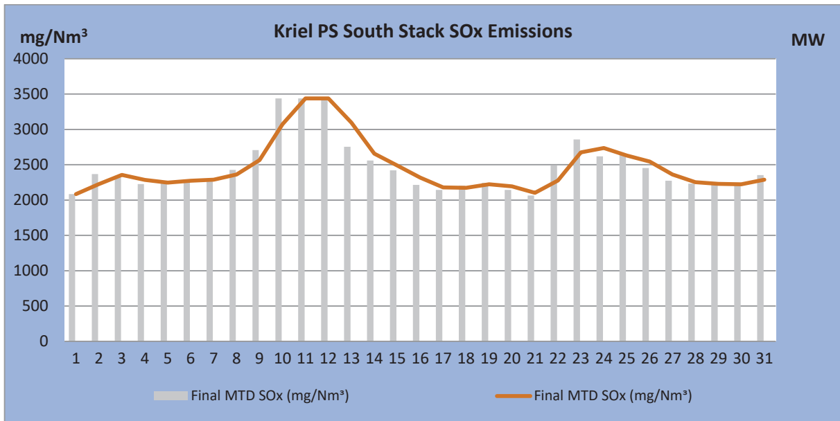
Figure 5. SO 2 emissions (daily averages) for the month of March 2019 against emission limit for the South Stack. SO x permitted maximum release rate is 3 500mg/Nm 3
