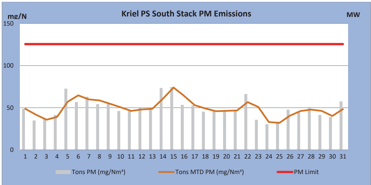
Figure 2: PM emissions (daily averages) for the month of March 2019 against emission limit for the South Stack
