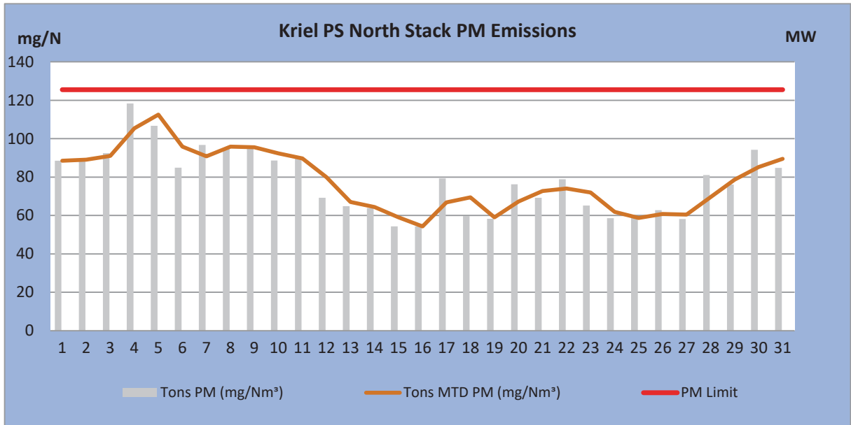
Figure 1: PM emissions (daily averages) for the month of March 2019 against emission limit for the North Stack
