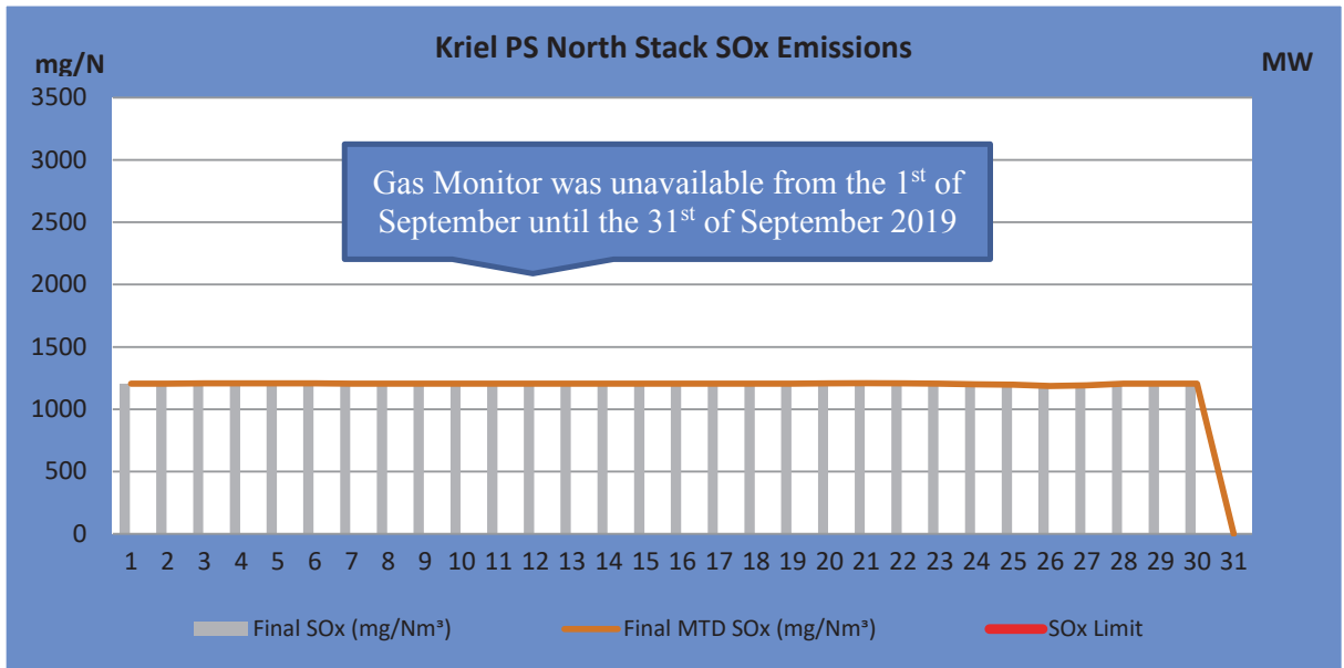
Figure 3. SO 2 emissions (daily averages) for the month of September 2019 against emission limit for the North Stack. SO x permitted maximum release rate is 3 500mg/Nm 3
