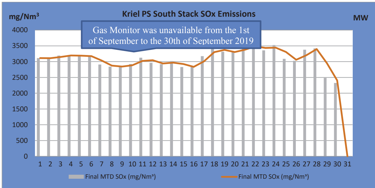
Figure 5. SO 2 emissions (daily averages) for the month of September 2019 against emission limit for the South Stack. SO x permitted maximum release rate is 3 500mg/Nm 3
