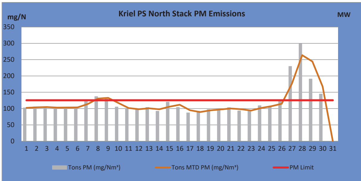
Figure 1: PM emissions (daily averages) for the month of September 2019 against emission limit for the North Stack
