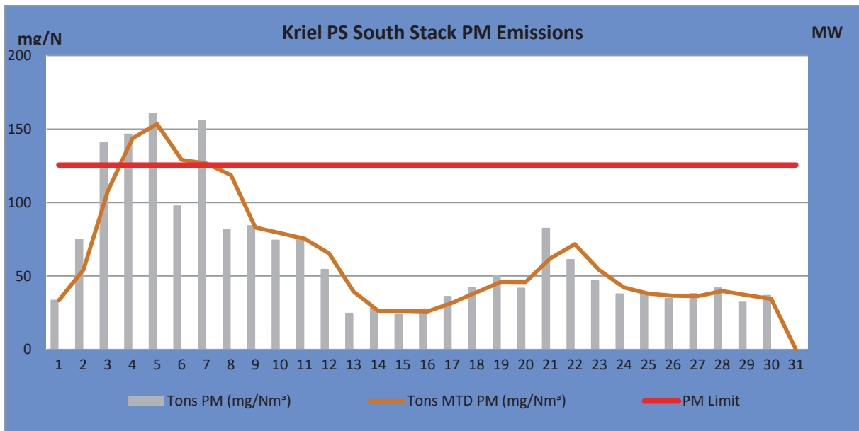
Figure 2: PM emissions (daily averages) for the month of September 2019 against emission limit for the South Stack
