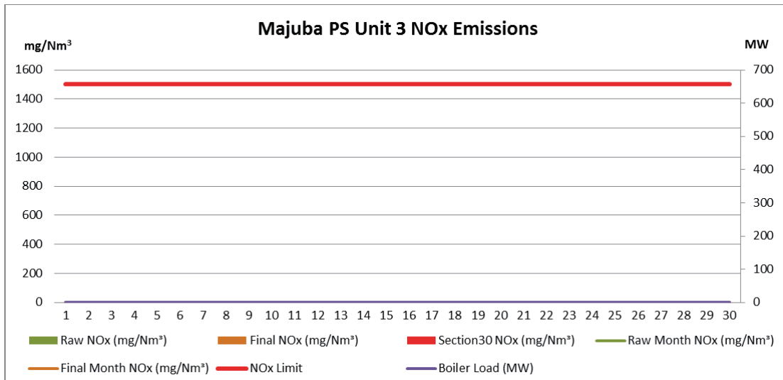
Figure 15. NOx emissions (daily averages) for the month of April 2019 against emission limit for Unit 3 (Unit on outage).
