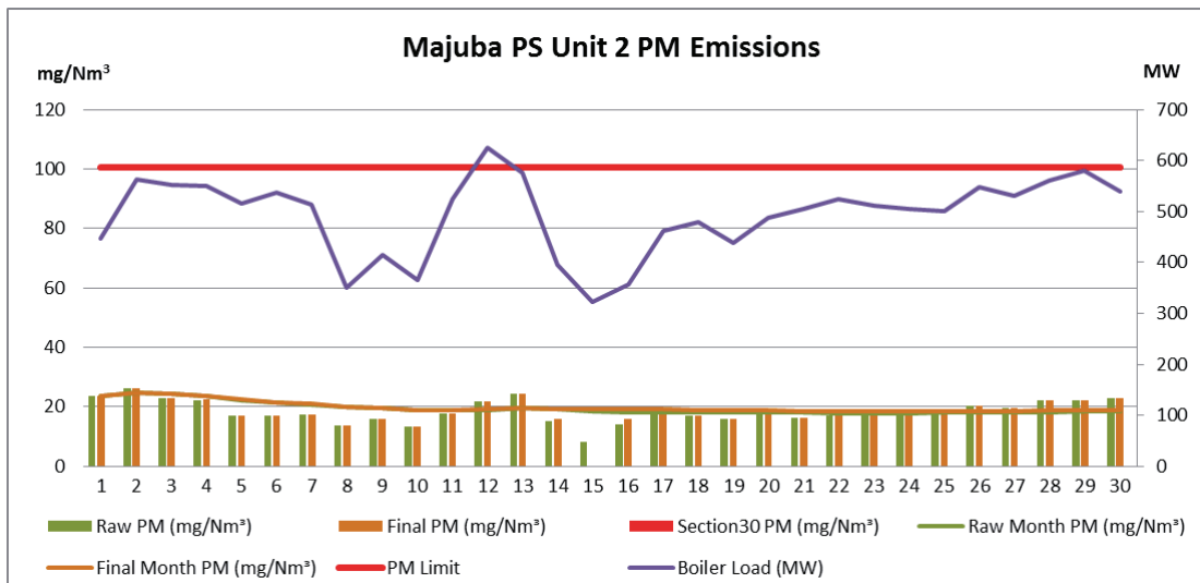
Figure 2. Particulate Matter emissions (daily averages) for the month of April 2019 against emission limit for Unit 2
