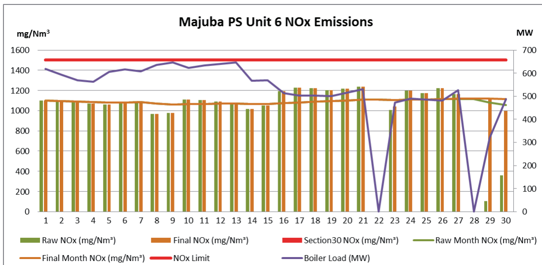
Figure 18. NOx emissions (daily averages) for the month April 2019 against emission limit for Unit 6
