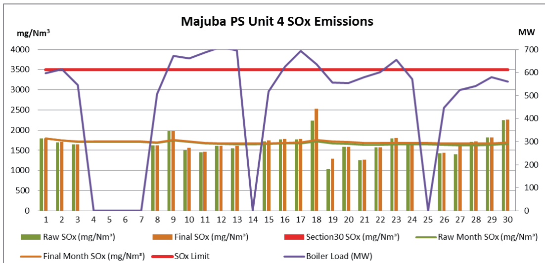
Figure 10. Sox emissions (daily averages) for the month of April 2019 against emission limit for Unit 4
