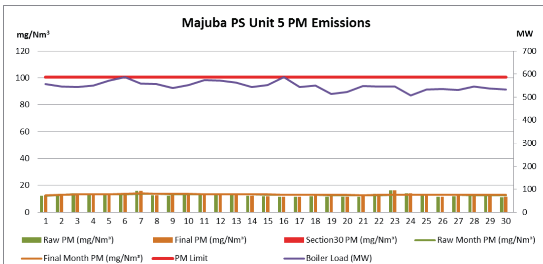
Figure 5. Particulate Matter emissions (daily averages) for the month of April 2019 against emission limit for Unit 5
