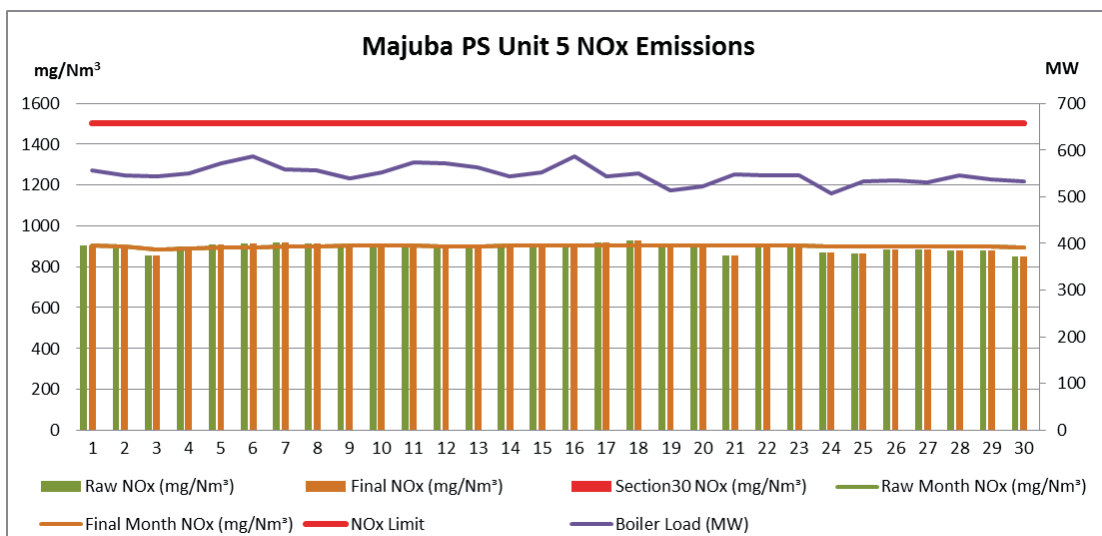
Figure 17. NOx emissions (daily averages) for the month of April 2019 against emission limit for Unit 5
