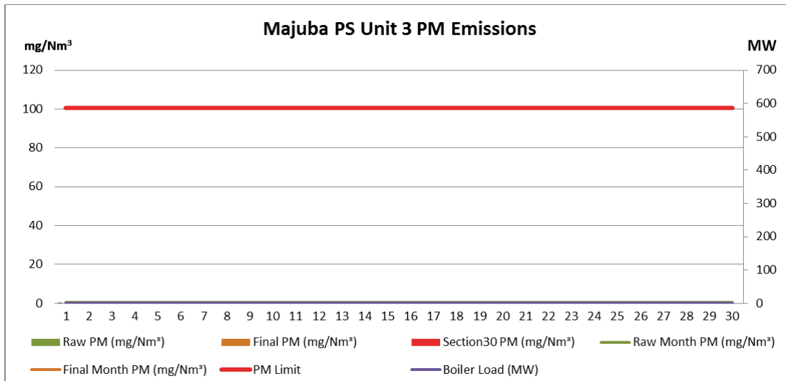
Figure 3. Particulate Matter emissions (daily averages) for the month of April 2019 against emission limit for Unit 3 (Unit on outage).
