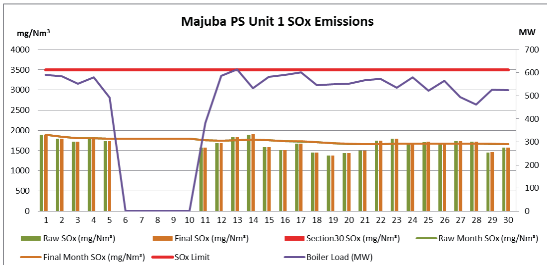
Figure 7. SOx emissions (daily averages) for the month of April 2019 against emission limit for Unit 1
