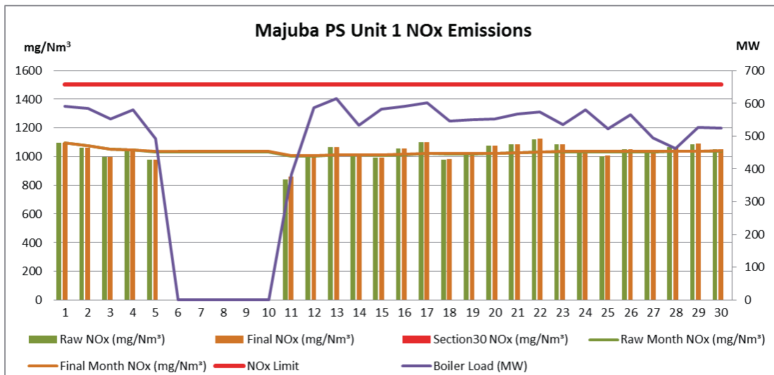
Figure 13. NOx emissions (daily averages) for the month of April 2019 against emission limit for Unit 1
