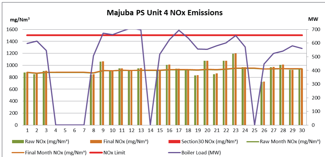
Figure 16. NOx emissions (daily averages) for the month of April 2019 against emission limit for Unit 4
