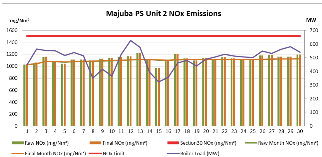
Figure 14. NOx emissions (daily averages) for the month of April 2019 against emission limit for Unit 2
