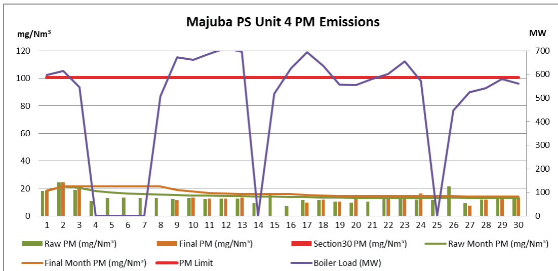
Figure 4. Particulate Matter emissions (daily averages) for the month of April 2019 against emission limit for Unit 4
