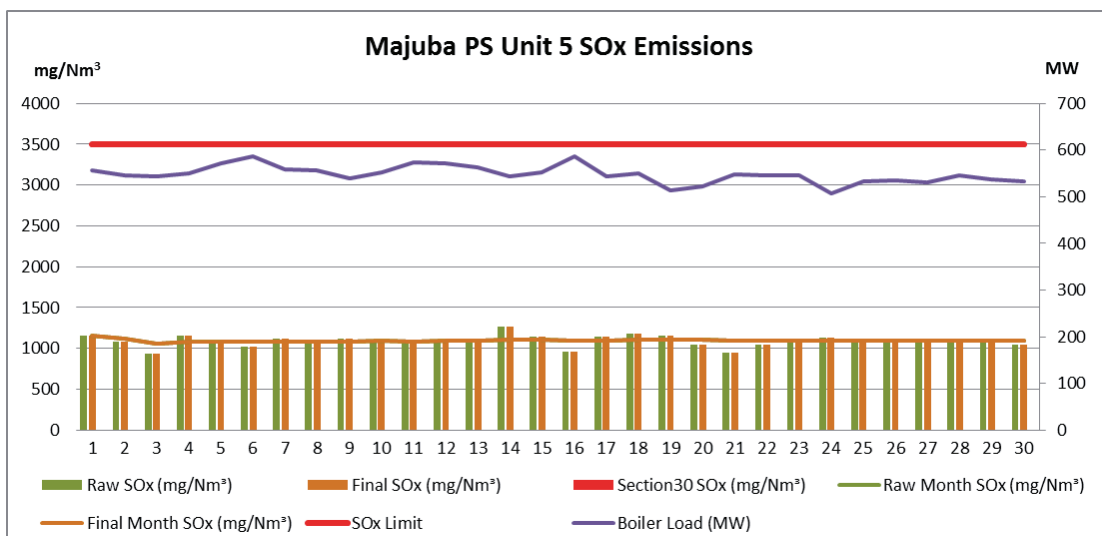
Figure 11. SOx emissions (daily averages) for the month of April 2019 against emission limit for Unit 5
