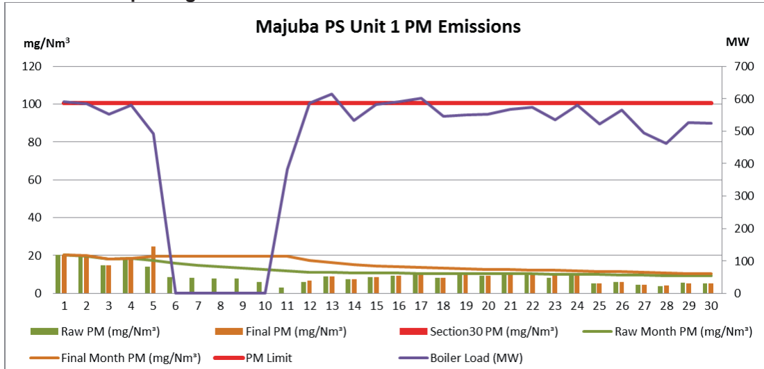
Figure 1. Particulate Matter emissions (daily averages) for the month of April 2019 against emission limit for Unit 1
