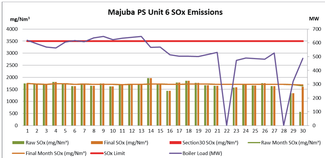
Figure 12. SOx emissions (daily averages) for the month of April 2019 against emission limit for Unit 6
