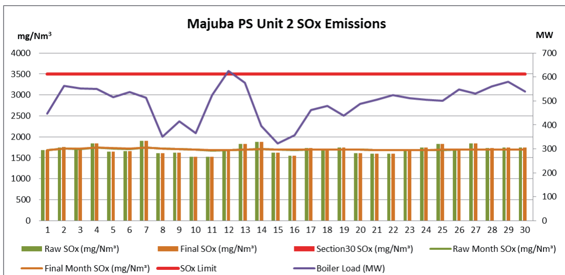
Figure 8. SOx emissions (daily averages) for the month of April 2019 against emission limit for Unit 2
