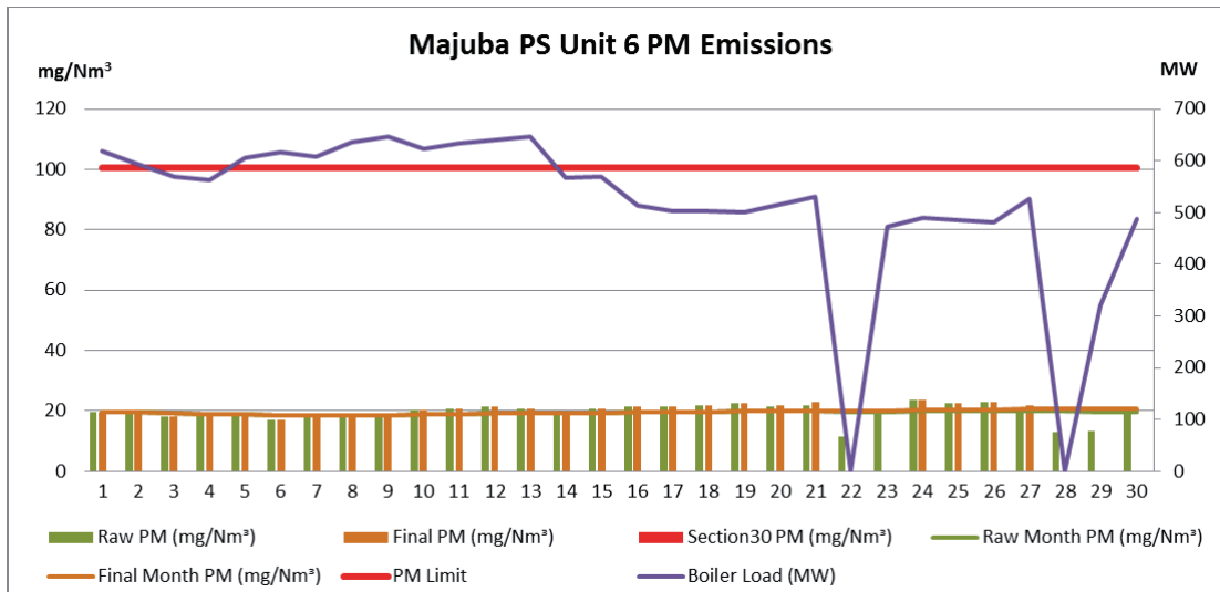
Figure 6. Particulate Matter emissions (daily averages) for the month of April 2019 against emission limit for Unit 6
