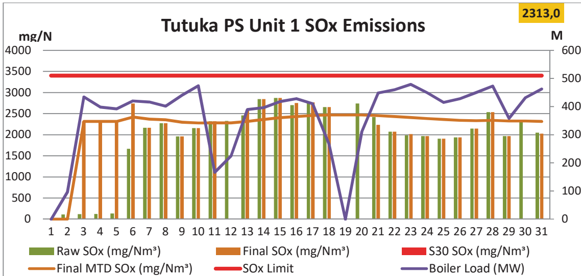
Figure 7: Unit 1 Daily Average SOx Emissions for the month of May 2019 (against the emissions limit and load generated)
