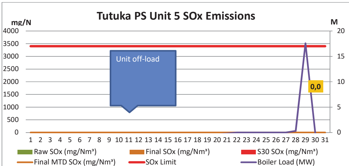
Figure 11: Unit 5 Daily Average SOx Emissions for the month of May 2019 (against the emissions limit and load generated)
