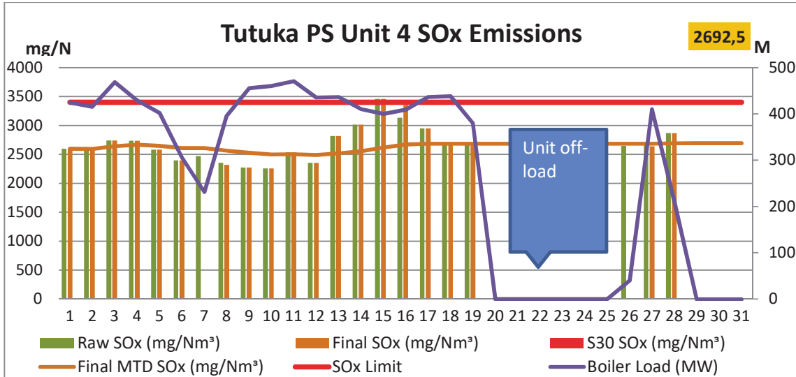
Figure 10: Unit 4 Daily Average SOx emissions for the month of May 2019 (against the emission limits and load generated)
