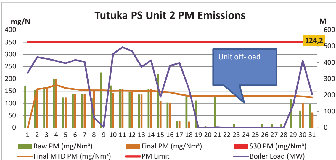
Figure 2: Unit 2 Daily Average emissions for the month of May 2019 (against the emission limits and load generated)
