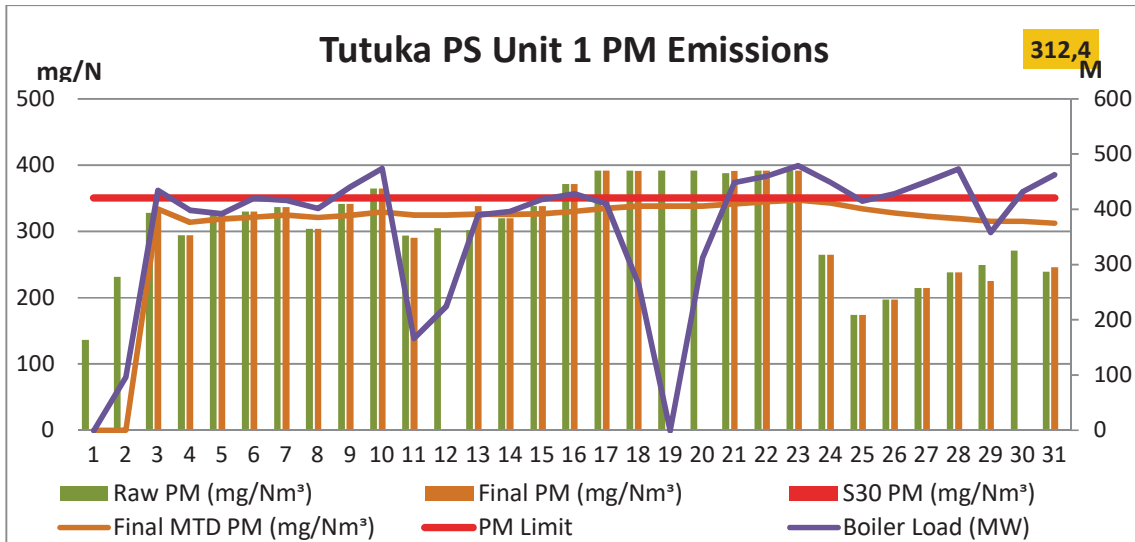
Figure 1: Unit 1 Daily Average Particulate Matter Emissions for the month of May 2019 (against the emissions limit and load generated)
