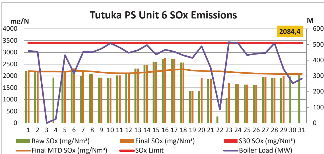
Figure 12: Unit 6 Daily SOx emissions for the month of May 2019 (against the emission limits and load generated)
