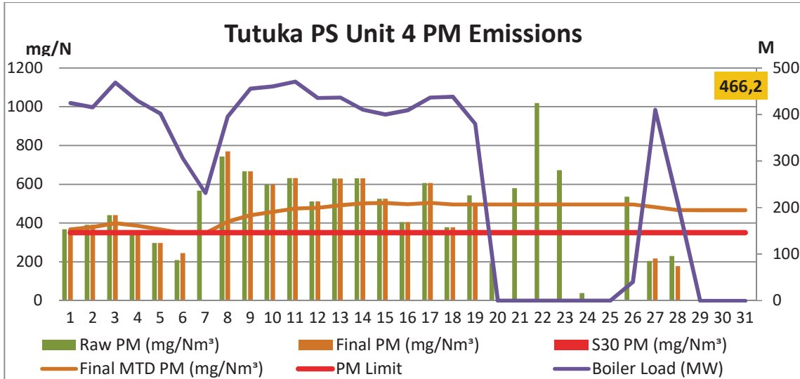
Figure 4: Unit 4 Daily Average PM emissions for the month of May 2019 (against the emission limits and load generated)
