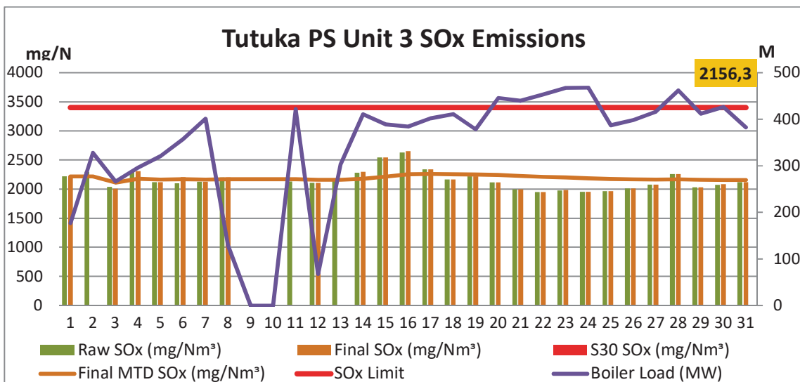
Figure 9: Unit 3 Daily Average SOx emissions for the month of May 2019 (against the emission limits and load generated)
