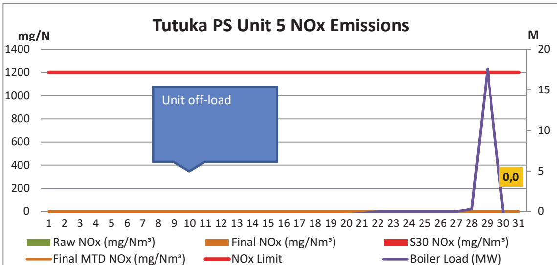
Figure 17: Unit 5 Daily Average NOx emissions for the month of May 2019 (against the emission limits and load generated)
