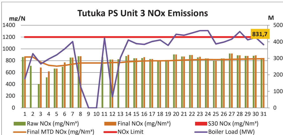
Figure 15: Unit 3 Daily Average NOx emissions for the month of May 2019 (against the emission limits and load generated)
