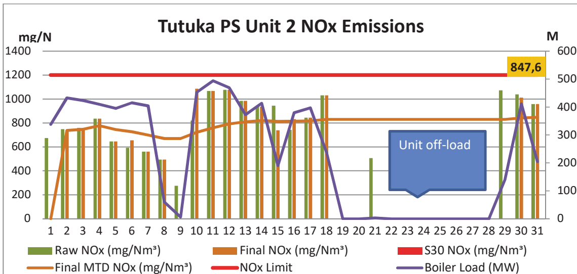
Figure 14: Unit 2 Daily Average NOx emissions for the month of May 2019 (against the emission limits and load generated)
