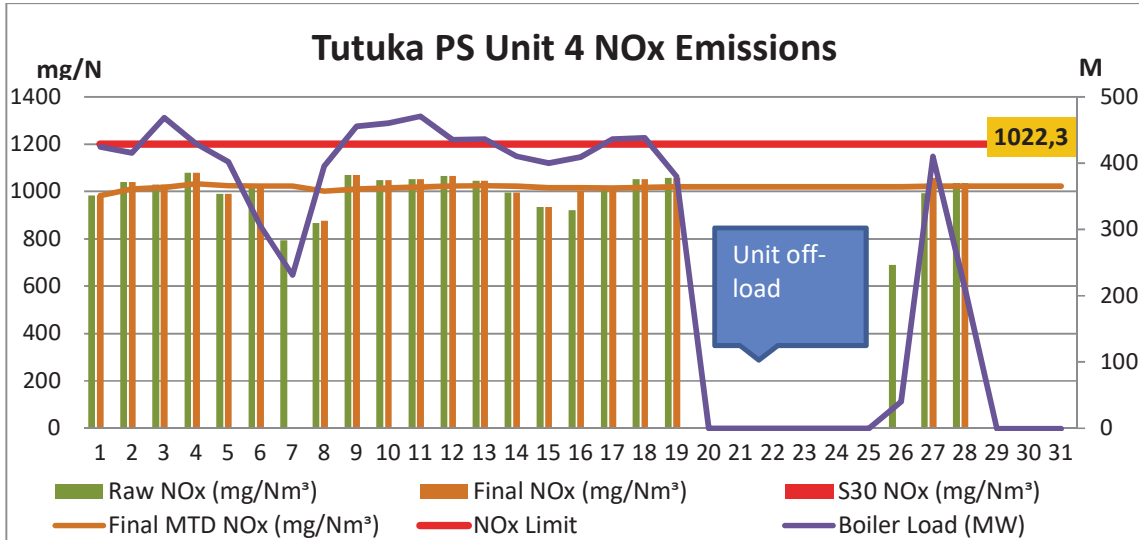
Figure 16: Unit 4 Daily Average NOx emissions for the month of May 2019 (against the emission limits and load generated)
