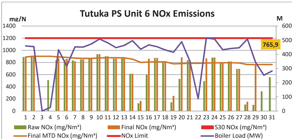
Figure 18: Unit 6 Daily Average NOx emissions for the month of May 2019 (against the emission limits and load generated)
