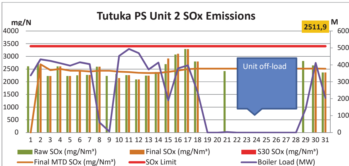
Figure 8: Unit 2 Daily Average SOx emissions for the month of May 2019 (against the emission limits and load generated)
