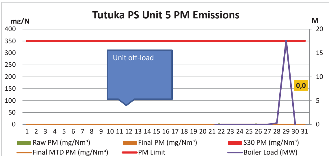
Figure 5: Unit 5 Daily Average Particulate Matter Emissions for the month of May 2019 (against the emissions limit and load generated)
