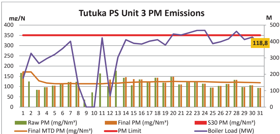
Figure 3: Unit 3 Daily Average Particulate Matter Emissions for the month of May 2019 (against the emissions limit and load generated)
