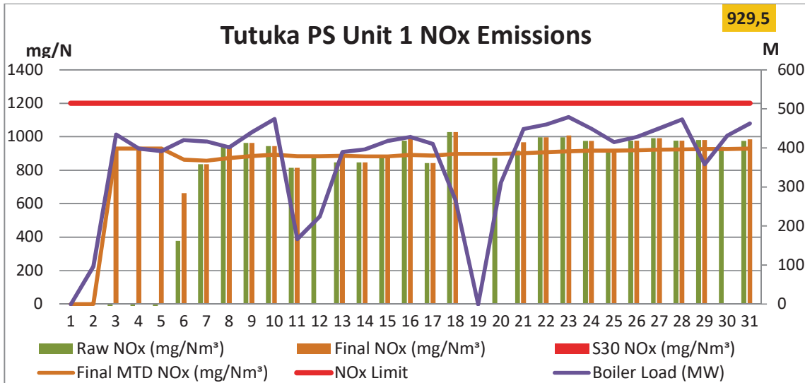
Figure 13: Unit 1 Daily Average NOx Emissions for the month of May 2019 (against the emissions limit and load generated)
