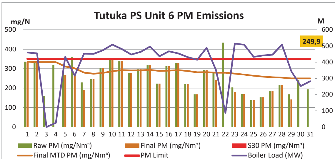
Figure 6: Unit 6 Daily Average PM emissions for the month of May 2019 (against the emission limits and load generated)
