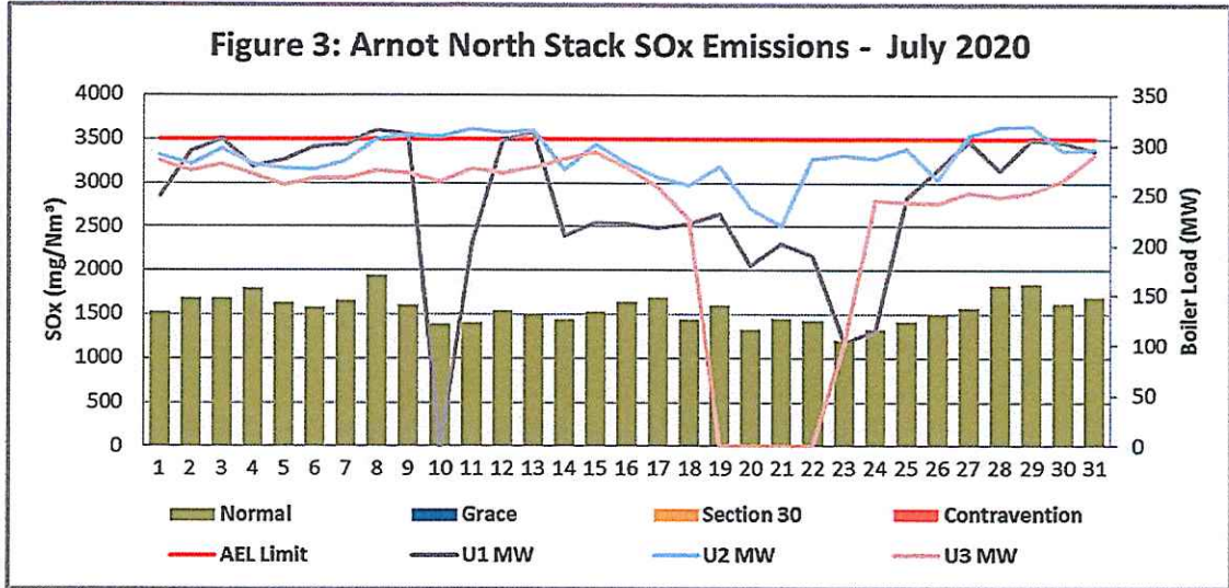
Figure 3: SO 2 emissions (daily averages) for the month of July 2020 against emission limit for the North Stack
