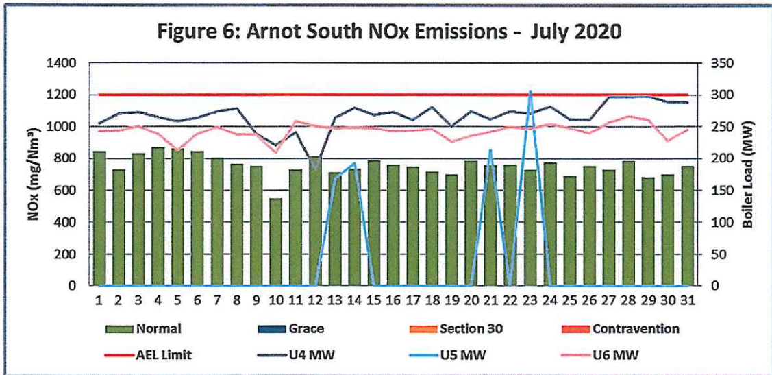
Figure 6: NO 2 emissions (daily averages) for the month of July -2020 against emission limit for the South Stack
