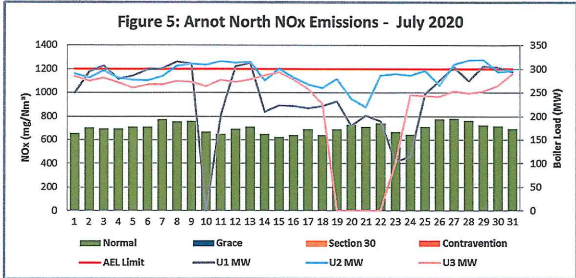
Figure 5: NO 2 emissions (daily averages) for the month of July-2020 against emission limit for the North Stack
