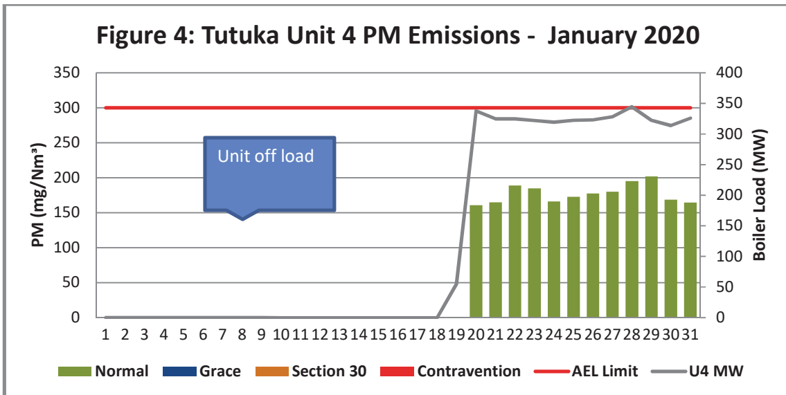
Figure 4: Unit 4 Daily Average PM emissions for the month of January 2020 (against the emission limits and load generated)
