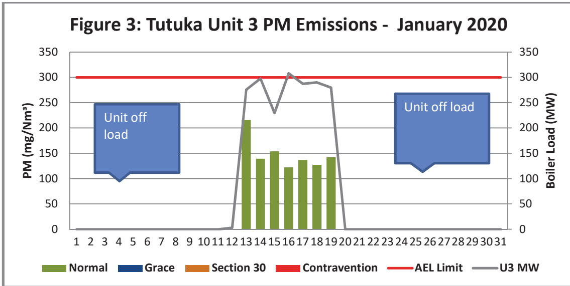
Figure 3: Unit 3 Daily Average Particulate Matter Emissions for the month of January 2020 (against the emissions limit and load generated)
