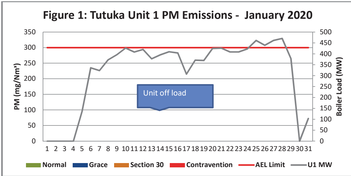
Figure 1: Unit 1 Daily Average Particulate Matter Emissions for the month of January 2020 (against the emissions limit and load generated)
