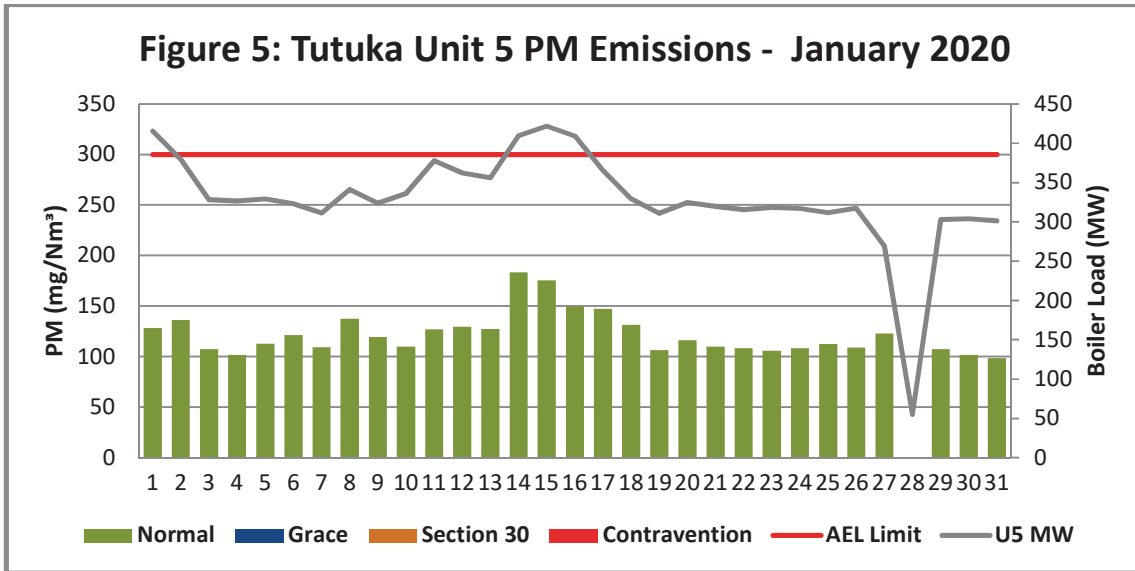
Figure 5: Unit 5 Daily Average Particulate Matter Emissions for the month of January 2020 (against the emissions limit and load generated)
