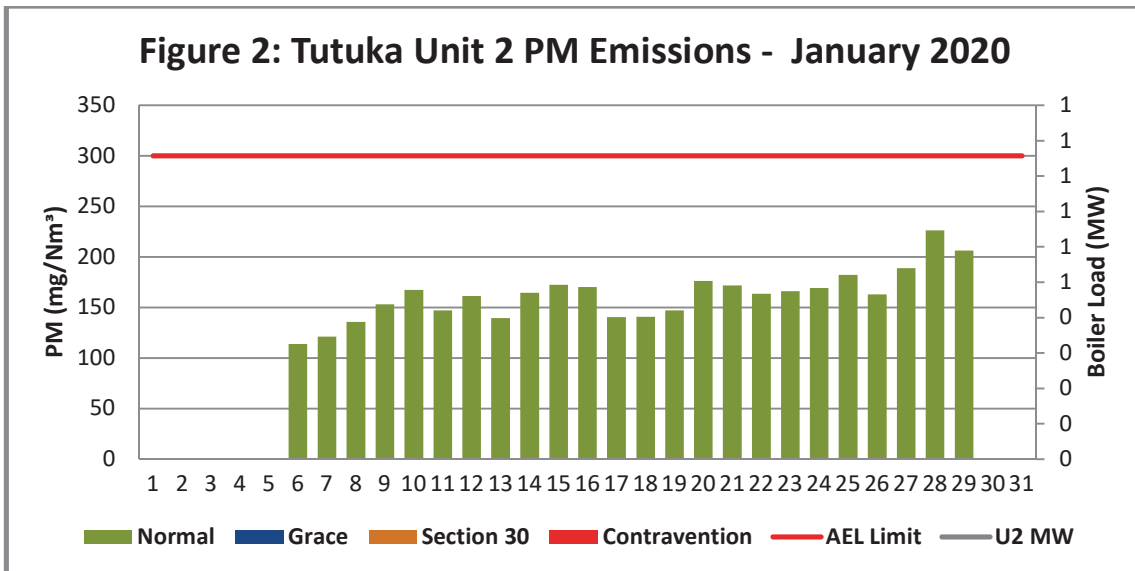
Figure 2: Unit 2 Daily Average emissions for the month of January 2020 (against the emission limits and load generated)
