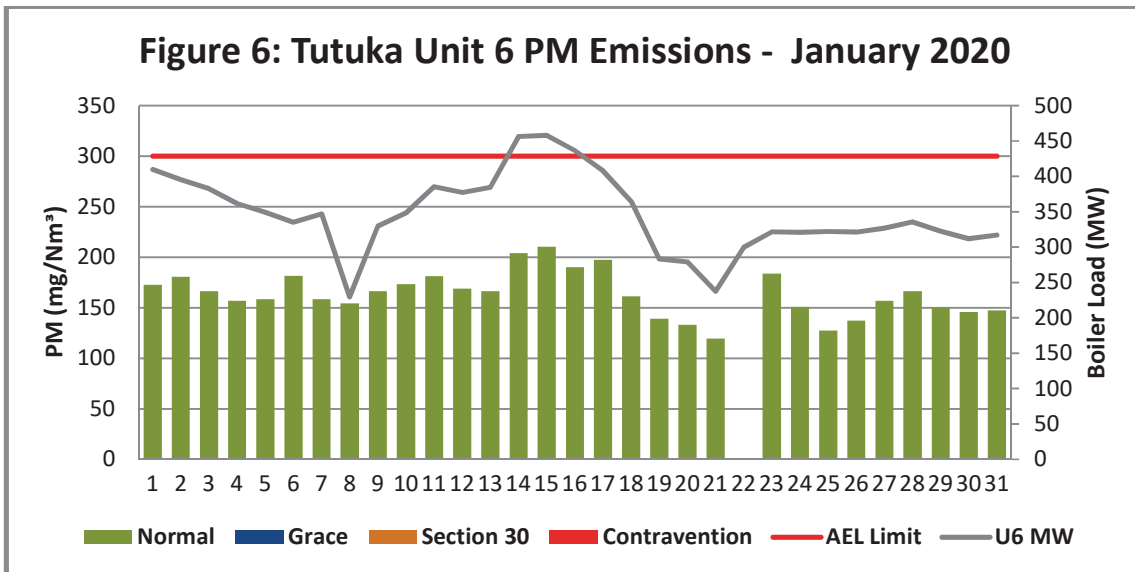
Figure 6: Unit 6 Daily Average PM emissions for the month of January 2020 (against the emission limits and load generated)
