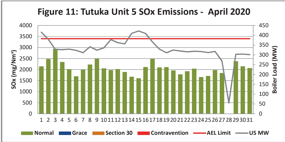
Figure 11: Unit 5 Daily Average SOx Emissions for the month of January 2020 (against the emissions limit and load generated)
