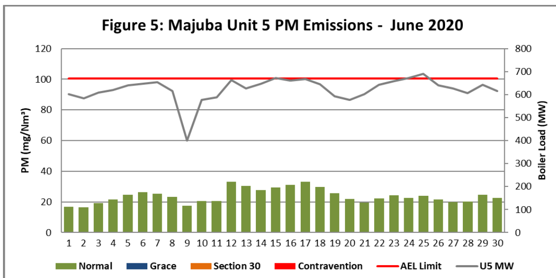
Figure 5. Particulate Matter emissions (daily averages) for the month of June 2020 against emission limit for Unit 5
