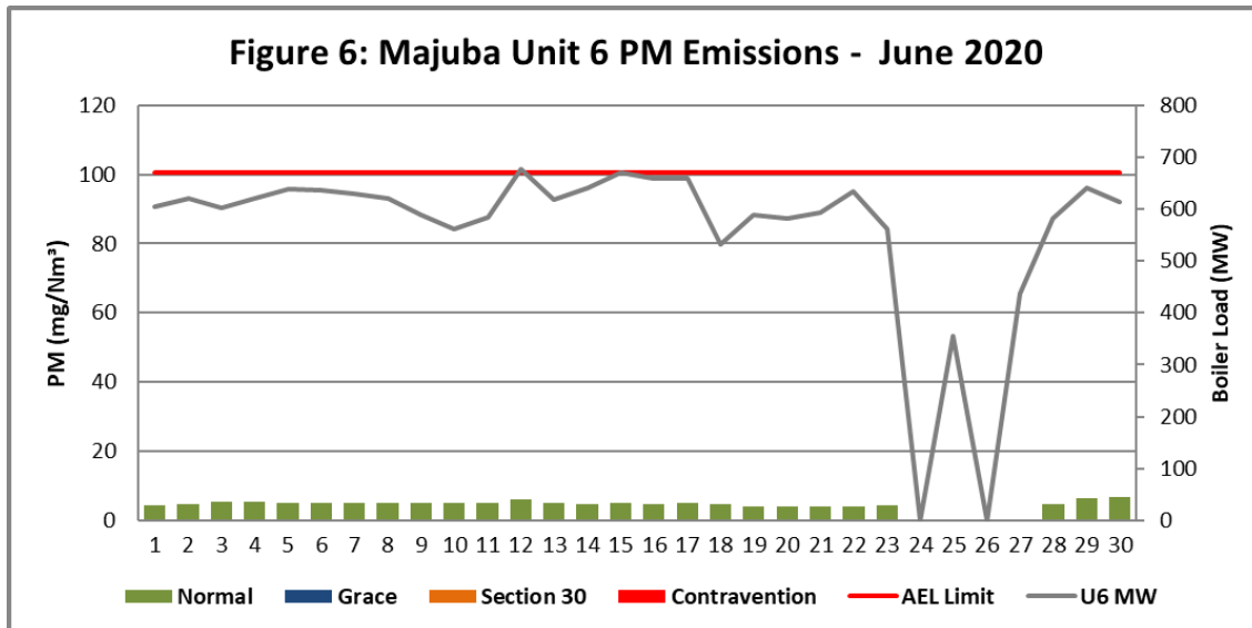
Figure 6. Particulate Matter emissions (daily averages) for the month of June 2020 against emission limit for Unit 6. *Both servers failed on Unit 6 resulting in dataloss between 05 and 11 June 2020. An average was calculated for those days.
