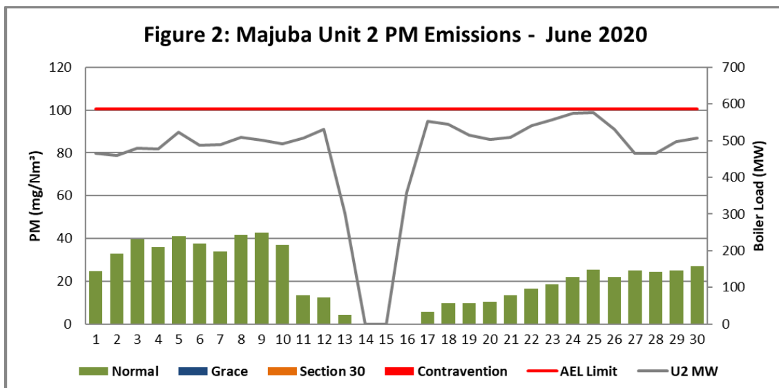
Figure 2. Particulate Matter emissions (daily averages) for the month of June 2020 against emission limit for Unit 2
