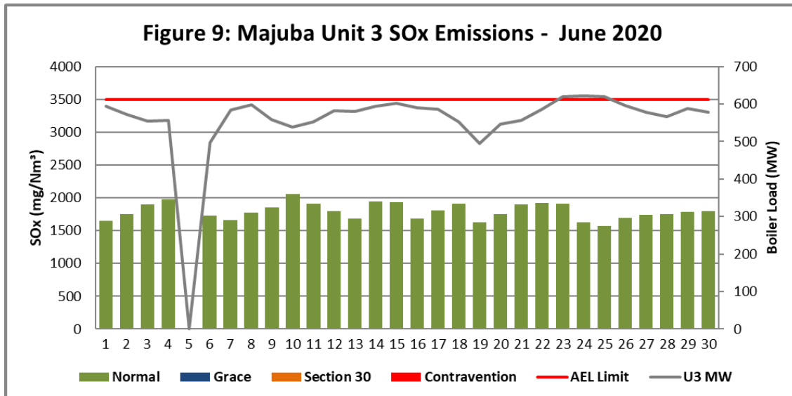
Figure 9. SOx emissions (daily averages) for the month of June 2020 against emission limit for Unit 3.
