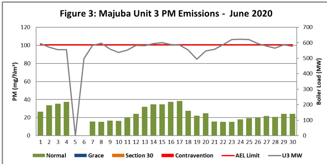
Figure 3. Particulate Matter emissions (daily averages) for the month of June 2020 against emission limit for Unit 3.
