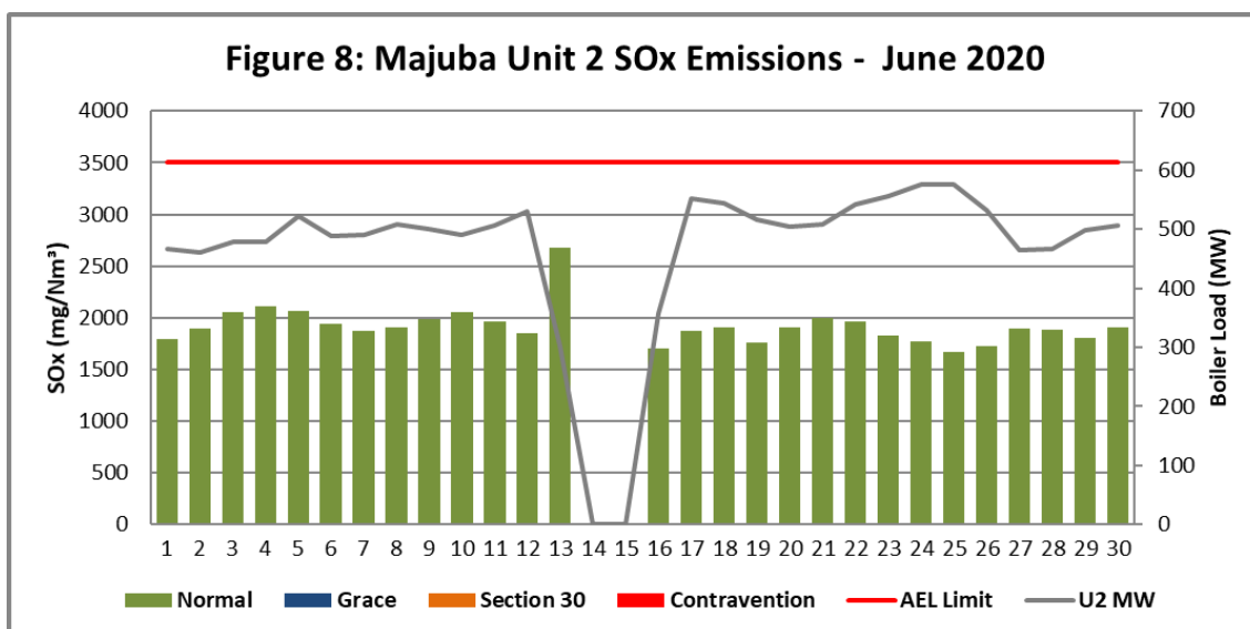
Figure 8. SOx emissions (daily averages) for the month of June 2020 against emission limit for Unit 2
