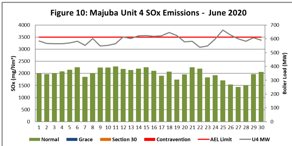
Figure 10. SOx emissions (daily averages) for the month of June 2020 against emission limit for Unit 4
