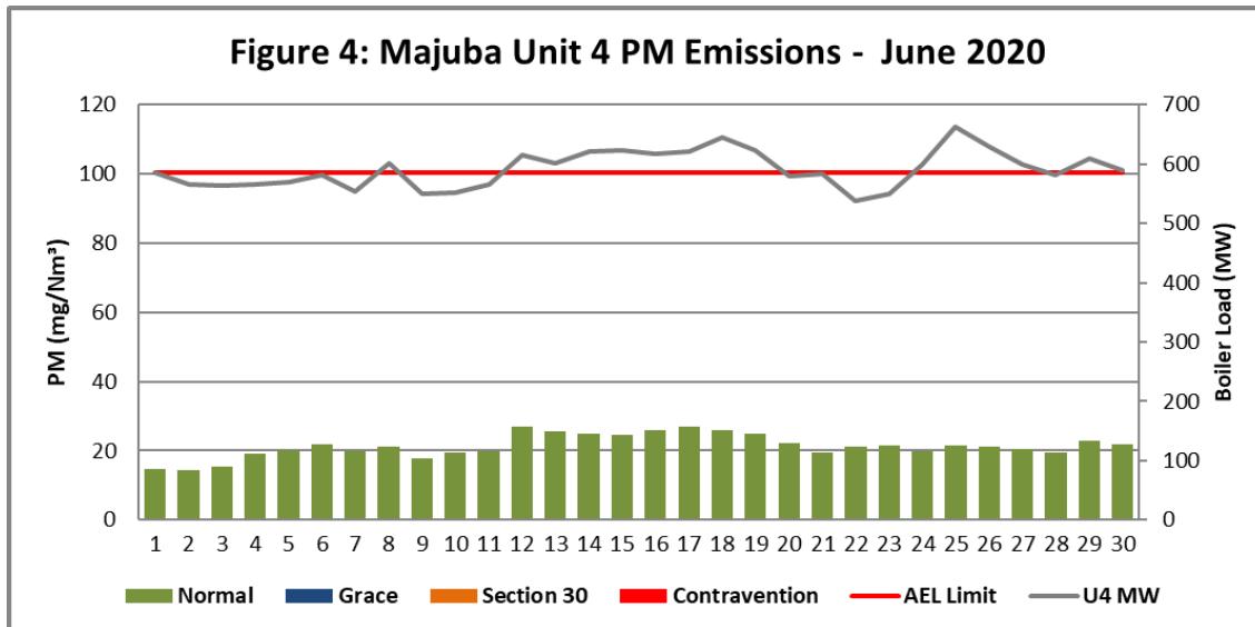
Figure 4. Particulate Matter emissions (daily averages) for the month of June 2020 against emission limit for Unit 4
