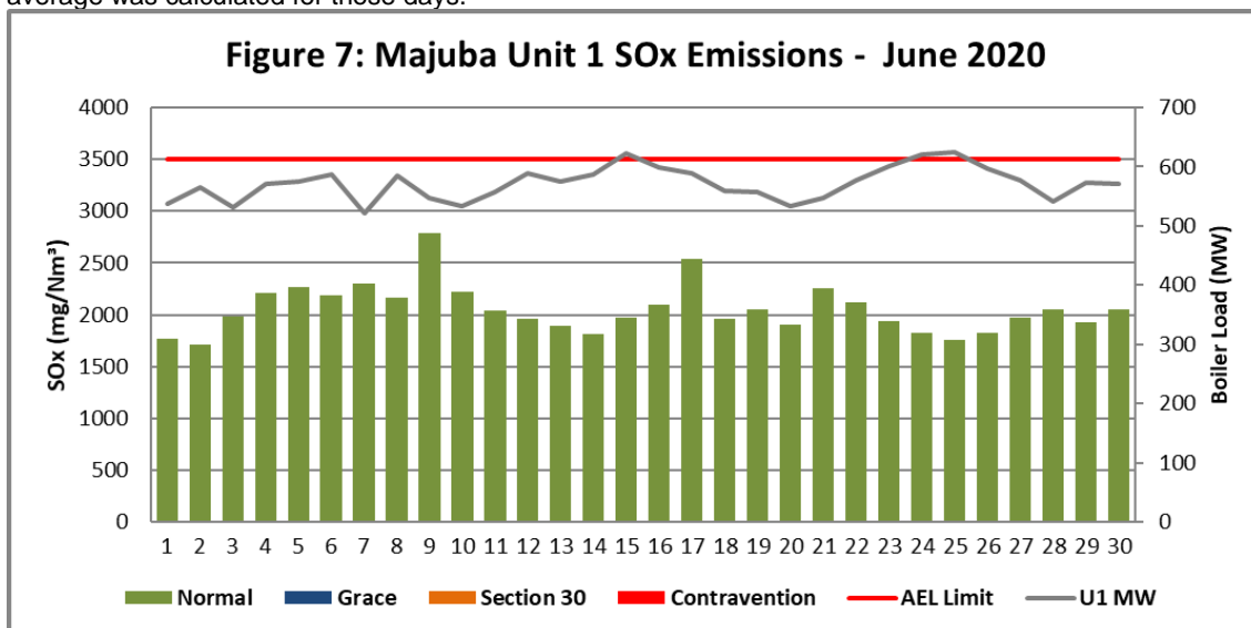
Figure 7. SOx emissions (daily averages) for the month of June 2020 against emission limit for Unit 1.
