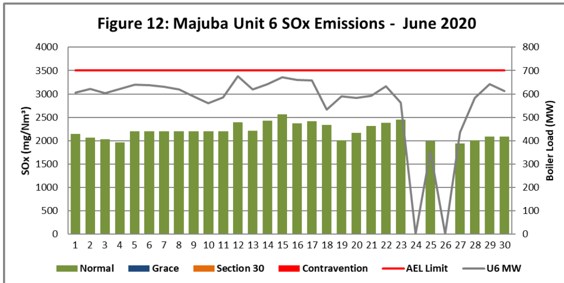
Figure 12. SOx emissions (daily averages) for the month of June 2020 against emission limit for Unit 6. *Both servers failed on Unit 6 resulting in dataloss between 05 and 11 June 2020. An average was calculated for those days.
