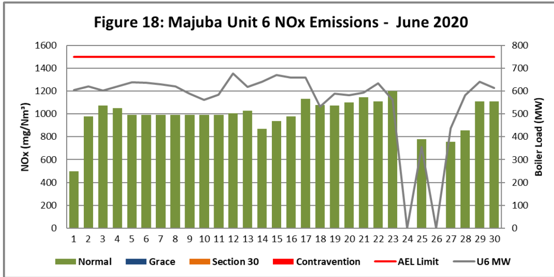
Figure 18. NO x emissions (daily averages) for the month June 2020 against emission limit for Unit 6 *Both servers failed on Unit 6 resulting in dataloss between 05 and 11 June 2020. An average was calculated for those days.
