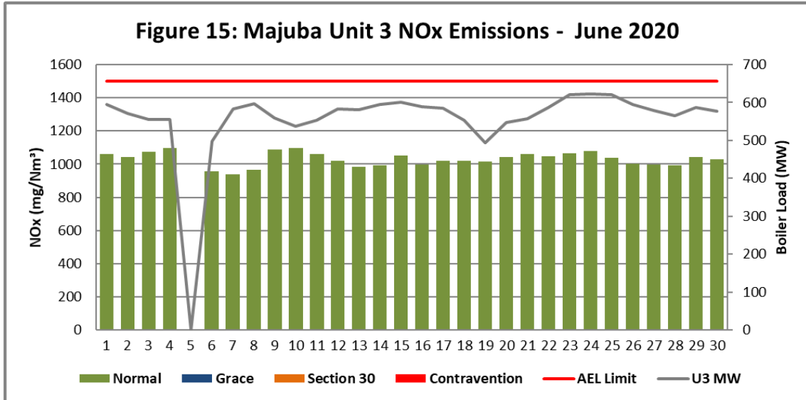
Figure 15. NOx emissions (daily averages) for the month of June 2020 against emission limit for Unit 3.
