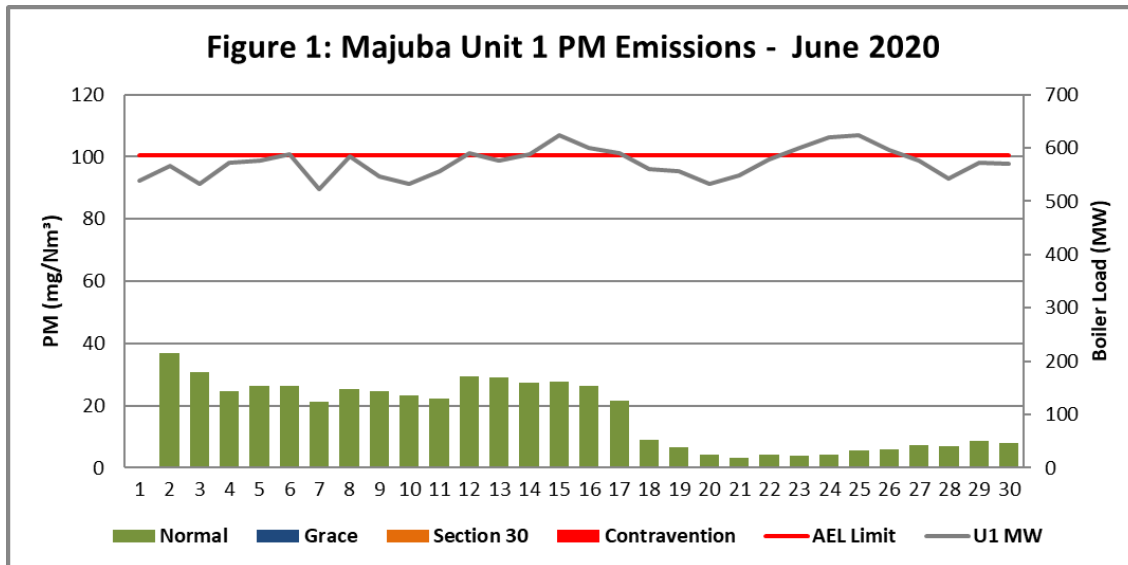
Figure 1. Particulate Matter emissions (daily averages) for the month of June 2020 against emission limit for Unit 1.
