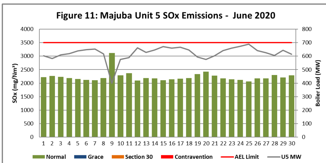
Figure 11. SOx emissions (daily averages) for the month of June 2020 against emission limit for Unit 5
