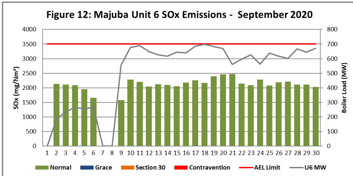
Figure 12. SOx emissions (daily averages) for the month of September 2020 against emission limit for Unit 6
