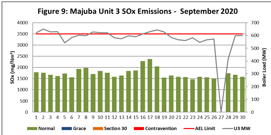
Figure 9. SOx emissions (daily averages) for the month of September 2020 against emission limit for Unit 3.
