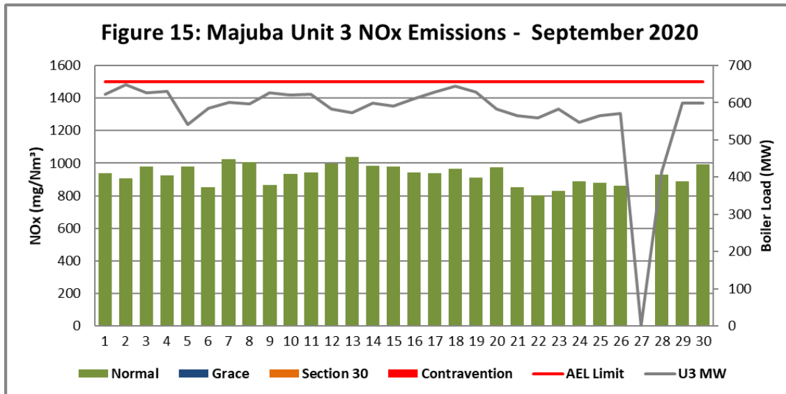
Figure 15. NOx emissions (daily averages) for the month of September 2020 against emission limit for Unit 3.
