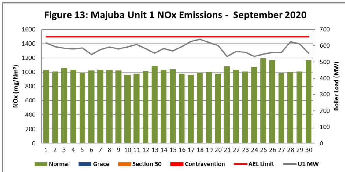
Figure 13. NOx emissions (daily averages) for the month of September 2020 against emission limit for Unit 1.
