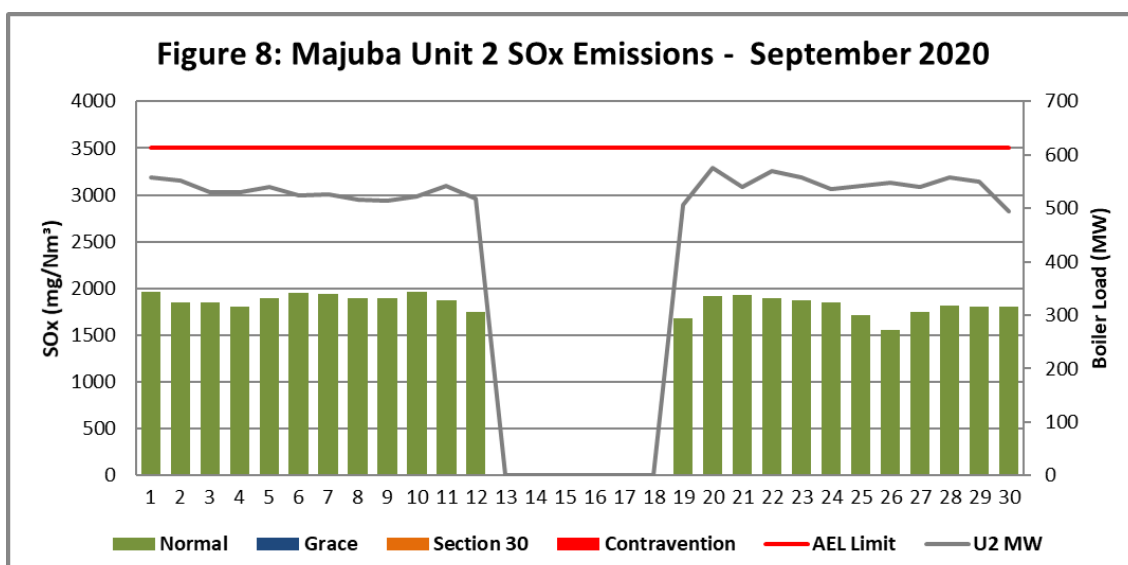
Figure 8. SOx emissions (daily averages) for the month of September 2020 against emission limit for Unit 2
