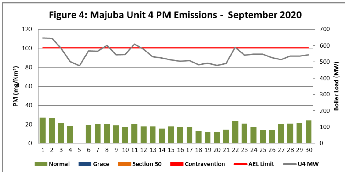
Figure 4. Particulate Matter emissions (daily averages) for the month of September 2020 against emission limit for Unit 4
