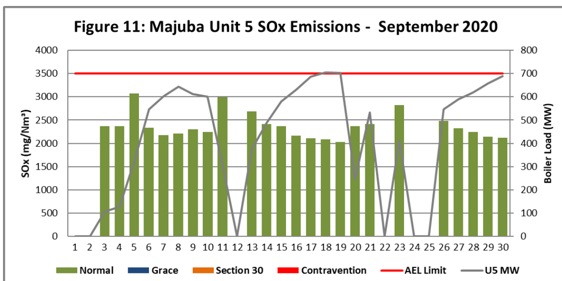
Figure 11. SOx emissions (daily averages) for the month of September 2020 against emission limit for Unit 5
