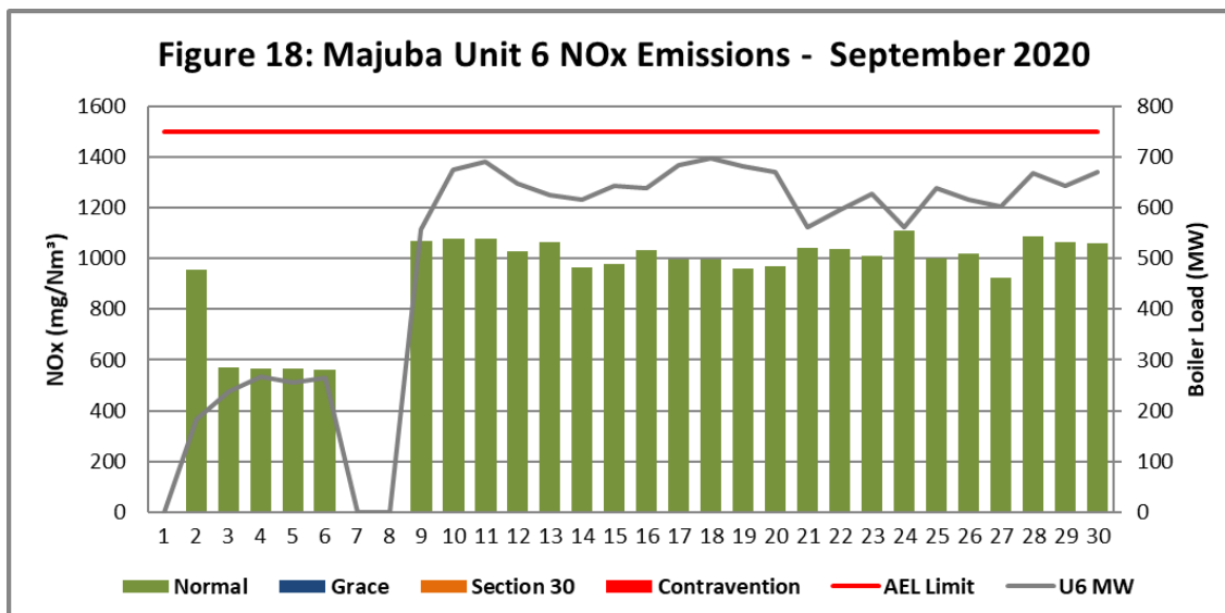
Figure 18. NOx emissions (daily averages) for the month September 2020 against emission limit for Unit 6
