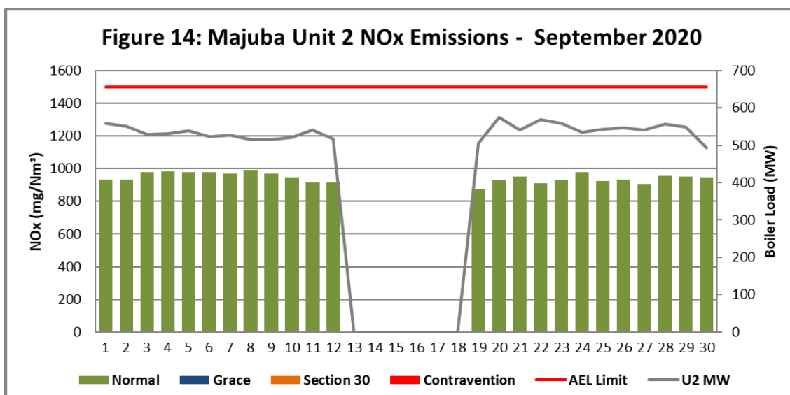
Figure 14. NOx emissions (daily averages) for the month of September 2020 against emission limit for Unit 2
