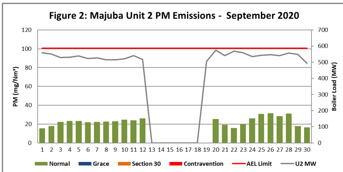
Figure 2. Particulate Matter emissions (daily averages) for the month of September 2020 against emission limit for Unit 2
