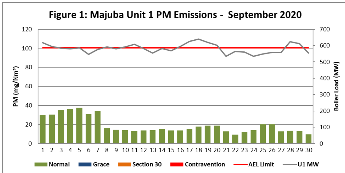
Figure 1. Particulate Matter emissions (daily averages) for the month of September 2020 against emission limit for Unit 1.
