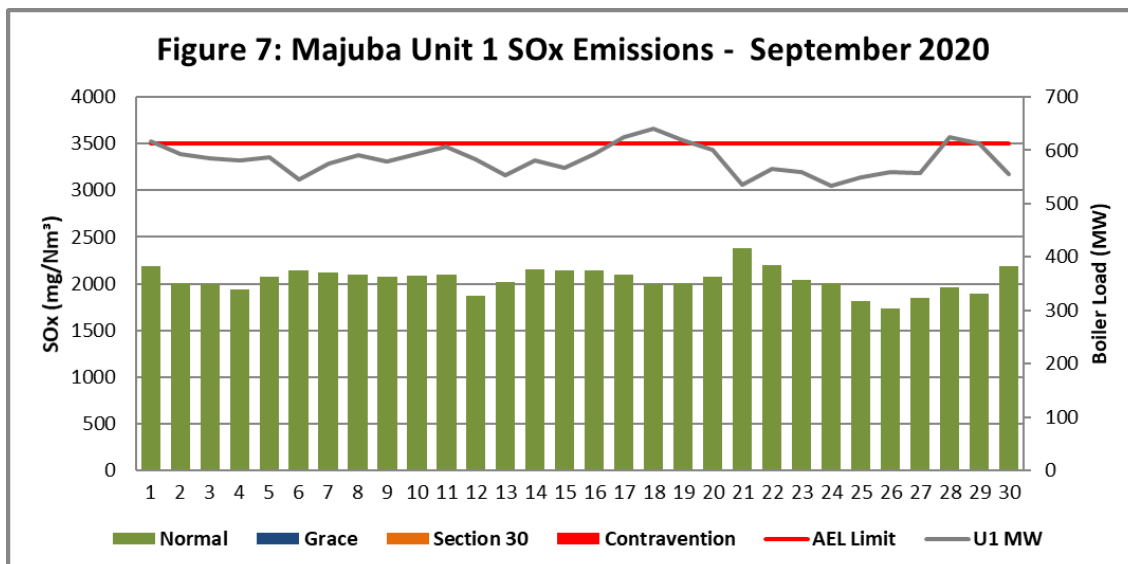
Figure 7. SOx emissions (daily averages) for the month of September 2020 against emission limit for Unit 1.
