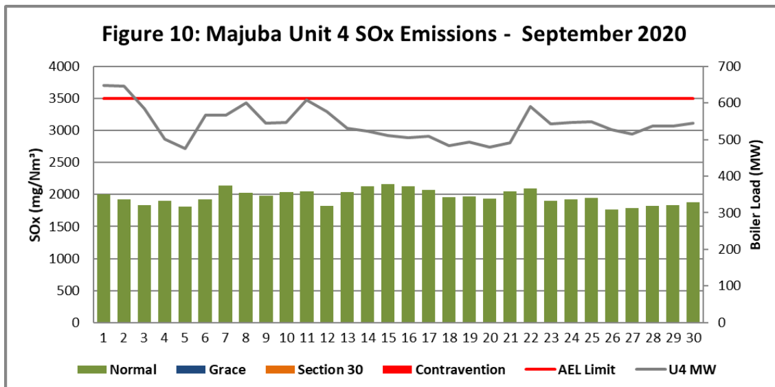
Figure 10. SOx emissions (daily averages) for the month of September 2020 against emission limit for Unit 4
