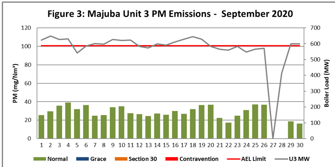
Figure 3. Particulate Matter emissions (daily averages) for the month of September 2020 against emission limit for Unit 3.
