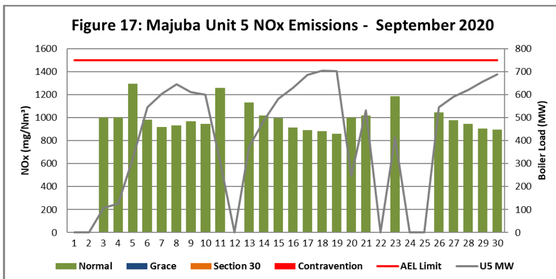
Figure 17. NOx emissions (daily averages) for the month of September 2020 against emission limit for Unit 5
