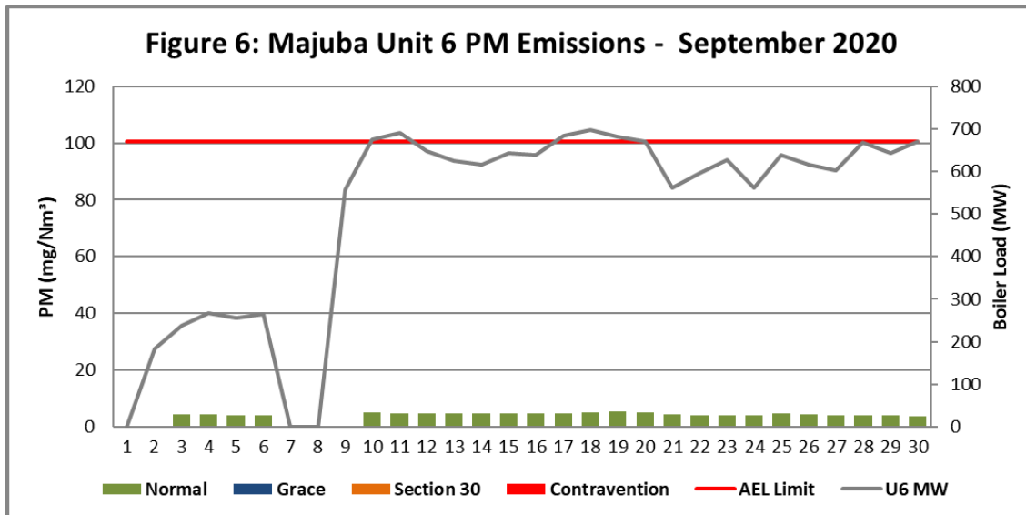
Figure 6. Particulate Matter emissions (daily averages) for the month of September 2020 against emission limit for Unit 6
