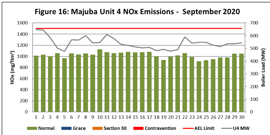
Figure 16. NOx emissions (daily averages) for the month of September 2020 against emission limit for Unit 4
