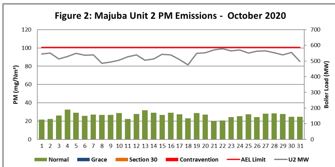
Figure 2. Particulate Matter emissions (daily averages) for the month of October 2020 against emission limit for Unit 2
