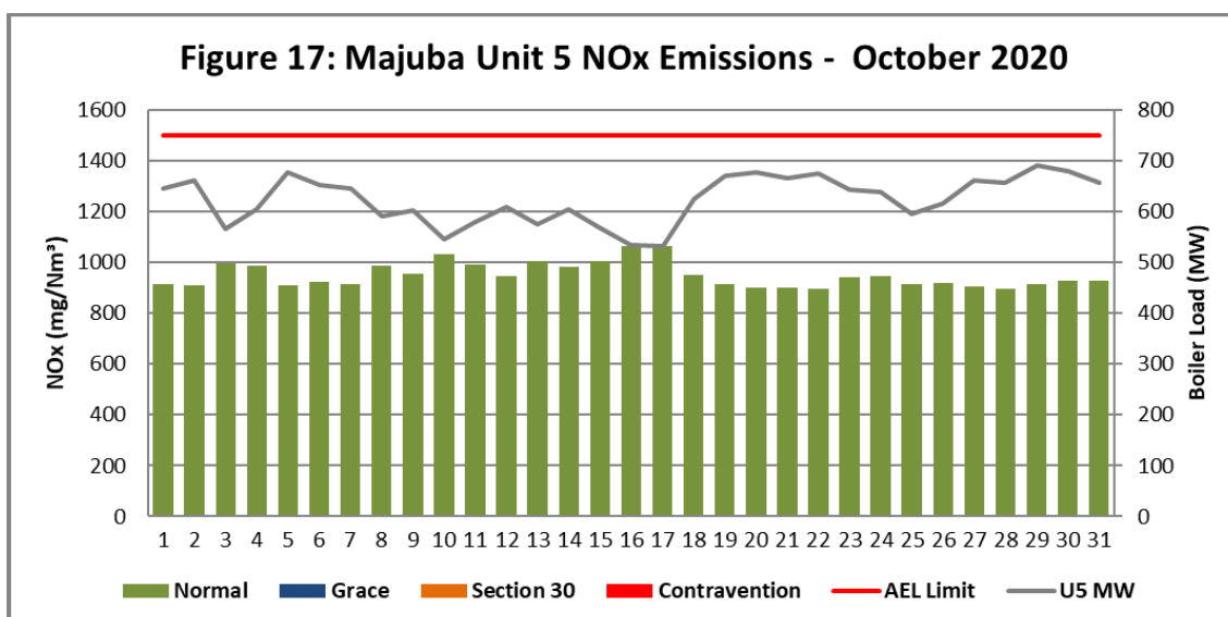
Figure 17. NOx emissions (daily averages) for the month of October 2020 against emission limit for Unit 5
