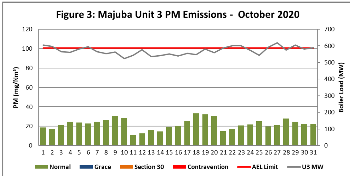
Figure 3. Particulate Matter emissions (daily averages) for the month of October 2020 against emission limit for Unit 3.
