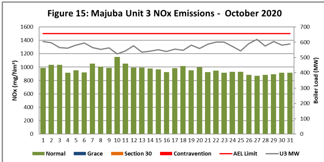
Figure 15. NOx emissions (daily averages) for the month of October 2020 against emission limit for Unit 3.
