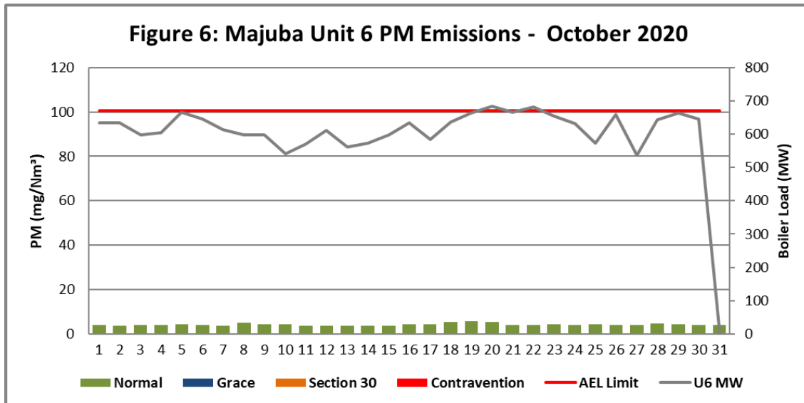
Figure 6. Particulate Matter emissions (daily averages) for the month of October 2020 against emission limit for Unit 6
