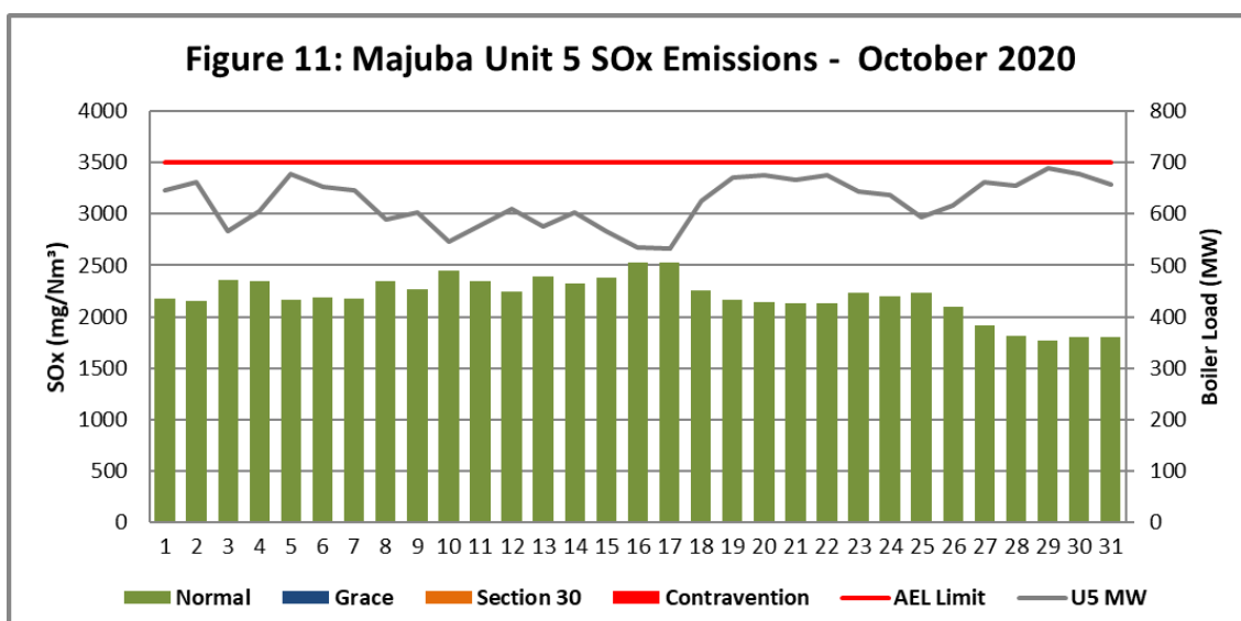
Figure 11. SOx emissions (daily averages) for the month of October 2020 against emission limit for Unit 5
