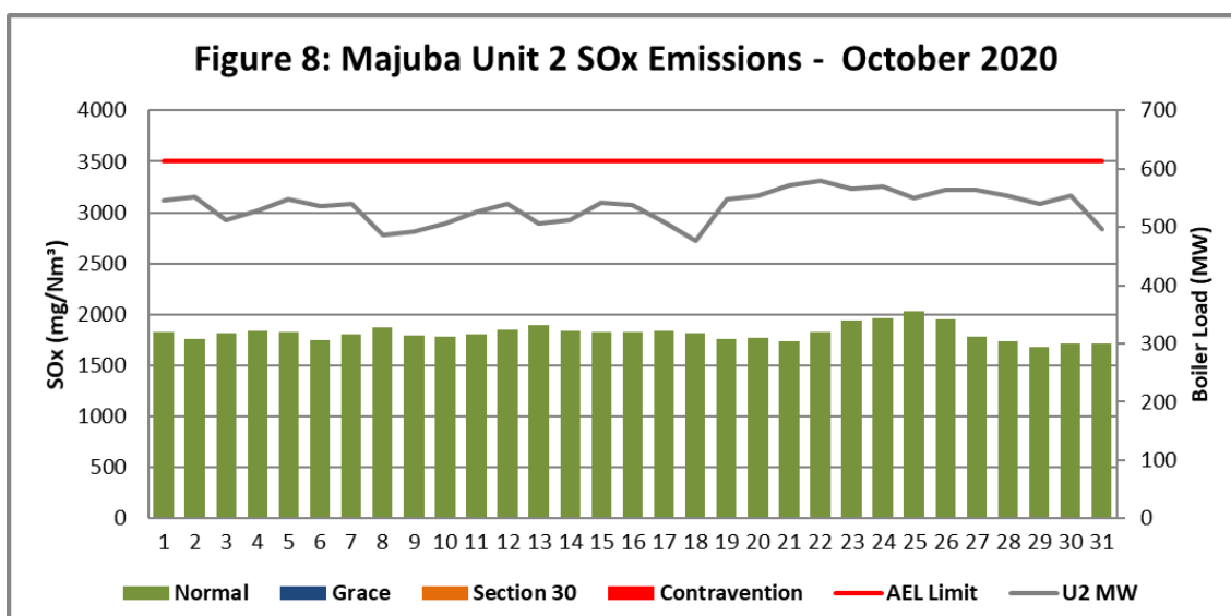
Figure 8. SOx emissions (daily averages) for the month of October 2020 against emission limit for Unit 2
