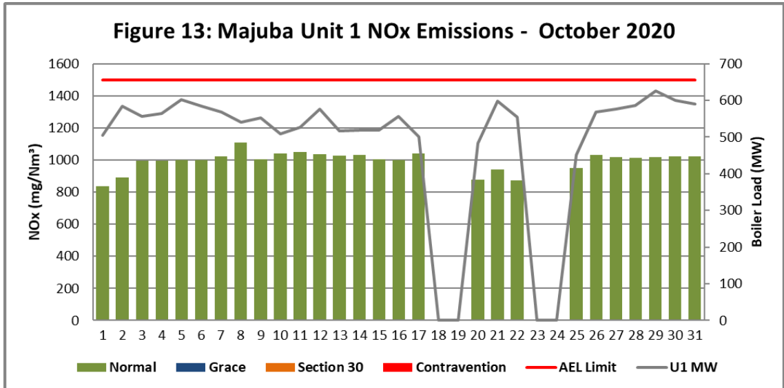
Figure 13. NOx emissions (daily averages) for the month of October 2020 against emission limit for Unit 1.
