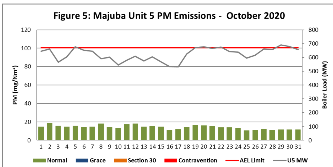
Figure 5. Particulate Matter emissions (daily averages) for the month of October 2020 against emission limit for Unit 5
