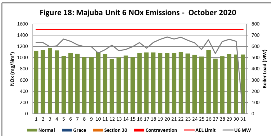
Figure 18. NOx emissions (daily averages) for the month October 2020 against emission limit for Unit 6
