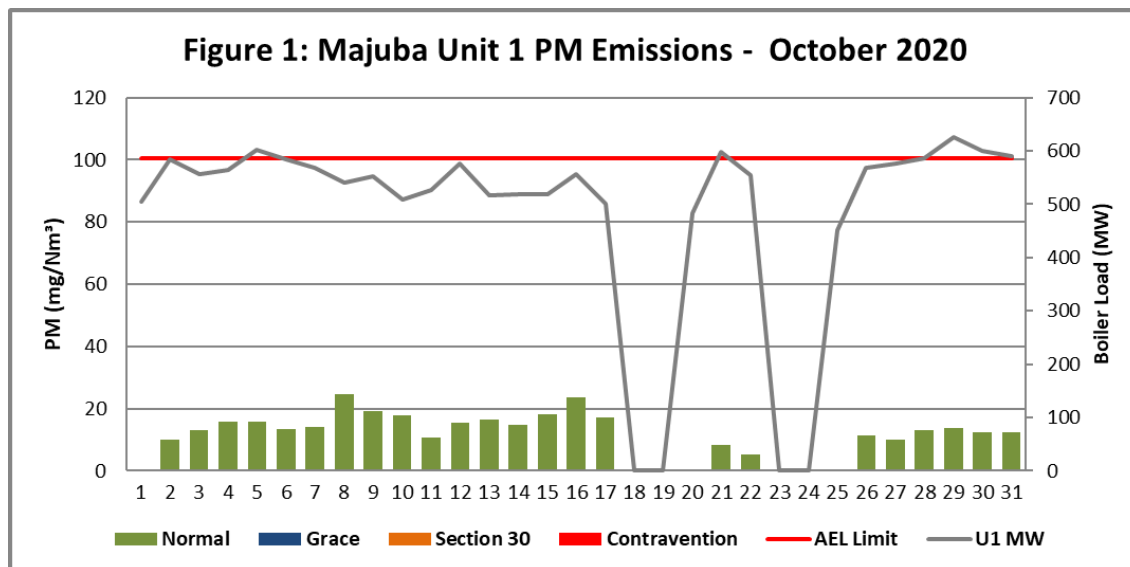
Figure 1. Particulate Matter emissions (daily averages) for the month of October 2020 against emission limit for Unit 1.
