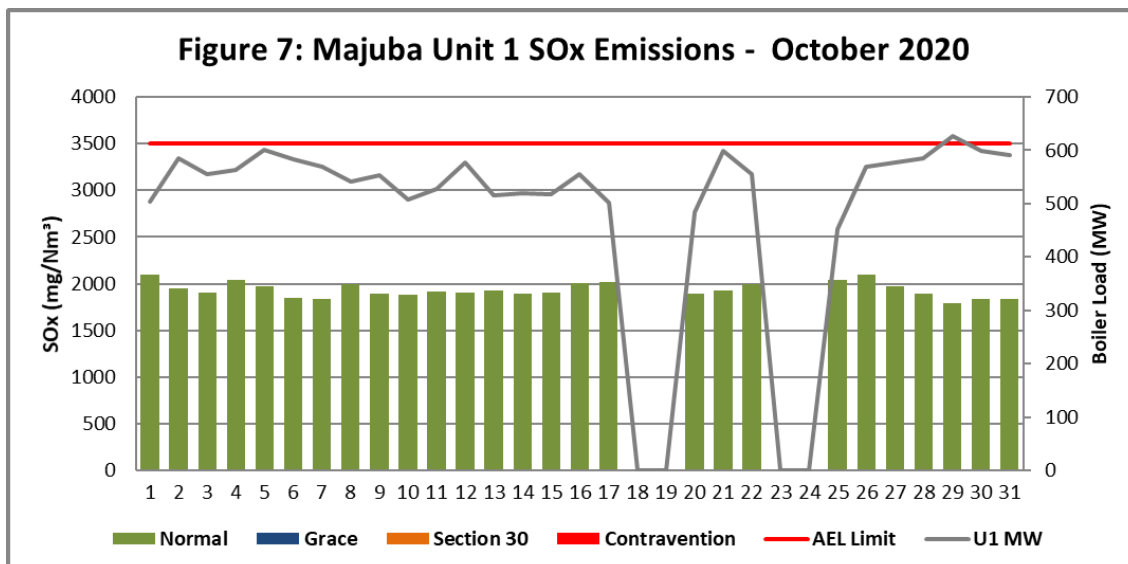
Figure 7. SOx emissions (daily averages) for the month of October 2020 against emission limit for Unit 1.
