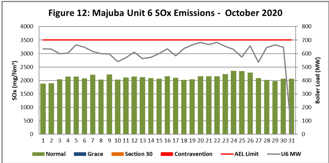
Figure 12. SOx emissions (daily averages) for the month of October 2020 against emission limit for Unit 6
