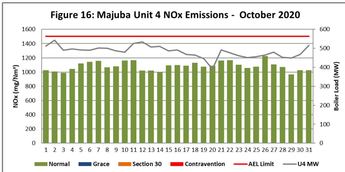
Figure 16. NOx emissions (daily averages) for the month of October 2020 against emission limit for Unit 4
