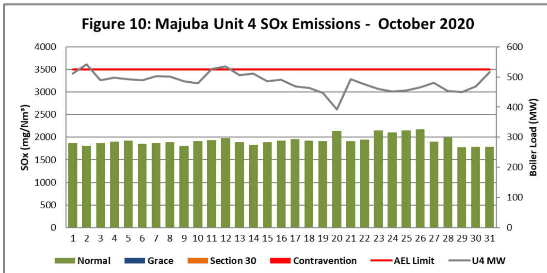
Figure 10. SOx emissions (daily averages) for the month of October 2020 against emission limit for Unit 4
