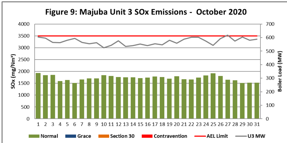
Figure 9. SOx emissions (daily averages) for the month of October 2020 against emission limit for Unit 3.
