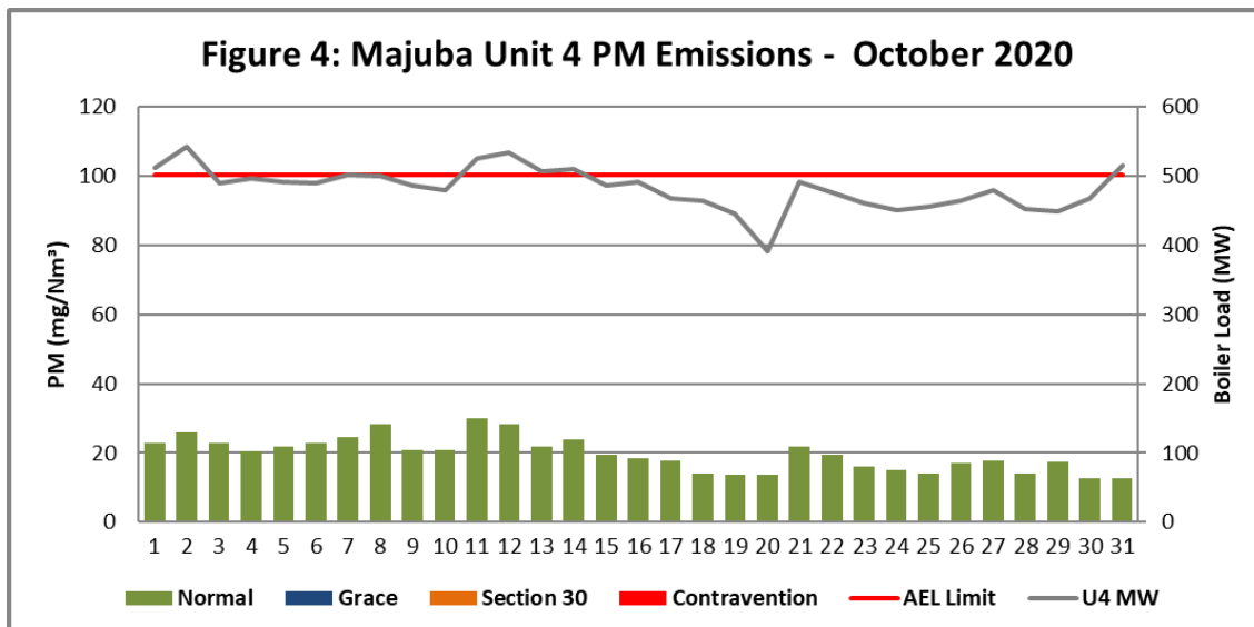
Figure 4. Particulate Matter emissions (daily averages) for the month of October 2020 against emission limit for Unit 4
