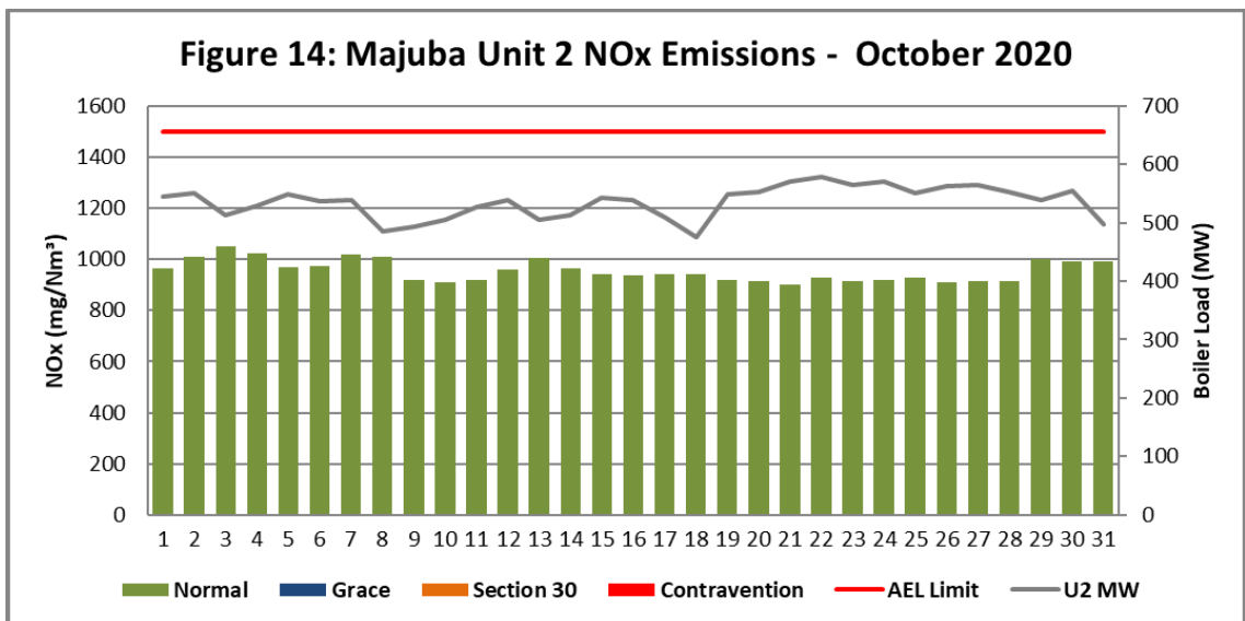
Figure 14. NOx emissions (daily averages) for the month of October 2020 against emission limit for Unit 2
