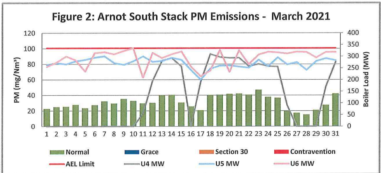
Figure 2: PM emissions (daily averages) for the month of March 2021 against emission limit for the South Stack
