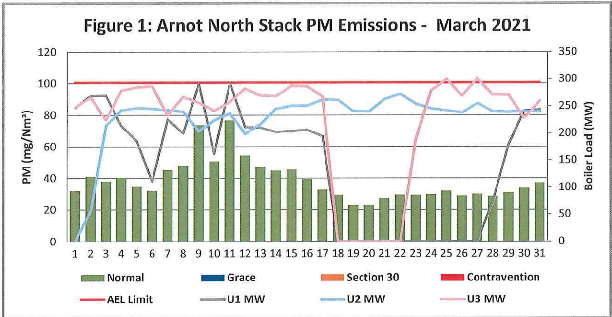
Figure 1: PM emissions (daily averages) for the month of March 2021 against emission limit for the North Stack
