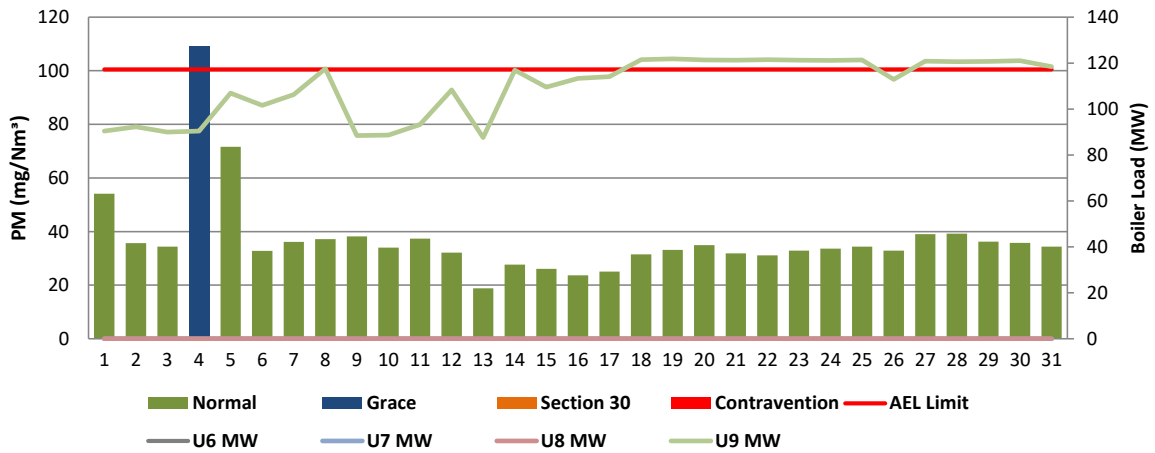
Figure 2: Komati West Stack PM Emissions - June 2020
