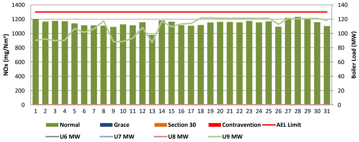
Figure 6: Komati West Stack NOx Emissions - June 2020
