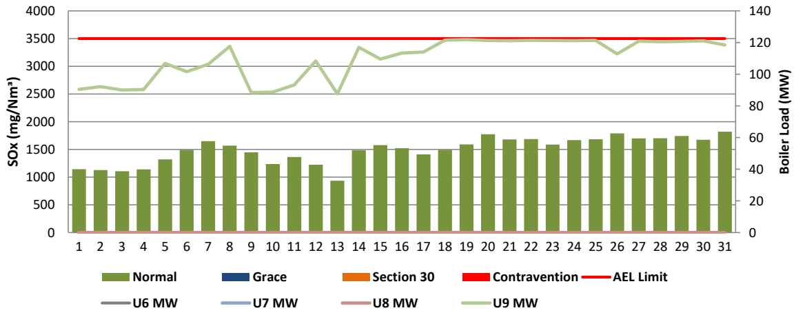
Figure 4: Komati West Stack SOx Emissions - June 2020
