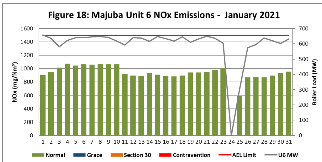
Figure 18. NOx emissions (daily averages) for the month January 2021 against emission limit for Unit 6
