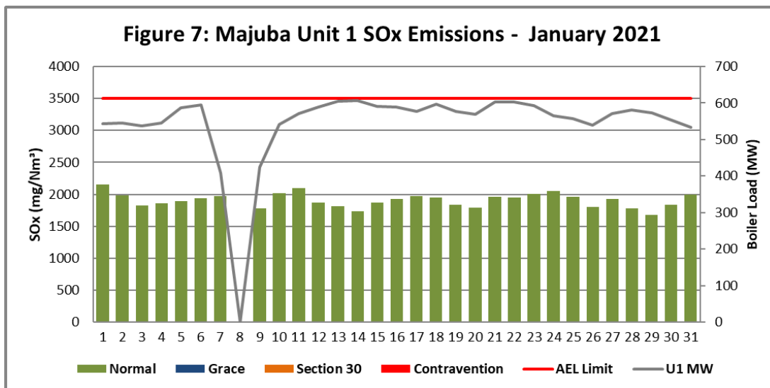
Figure 7. SOx emissions (daily averages) for the month of January 2021 against emission limit for Unit 1.
