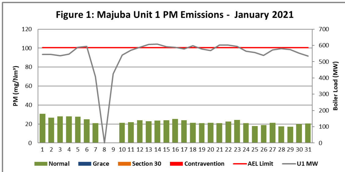
Figure 1. Particulate Matter emissions (daily averages) for the month of January 2021 against emission limit for Unit 1.
