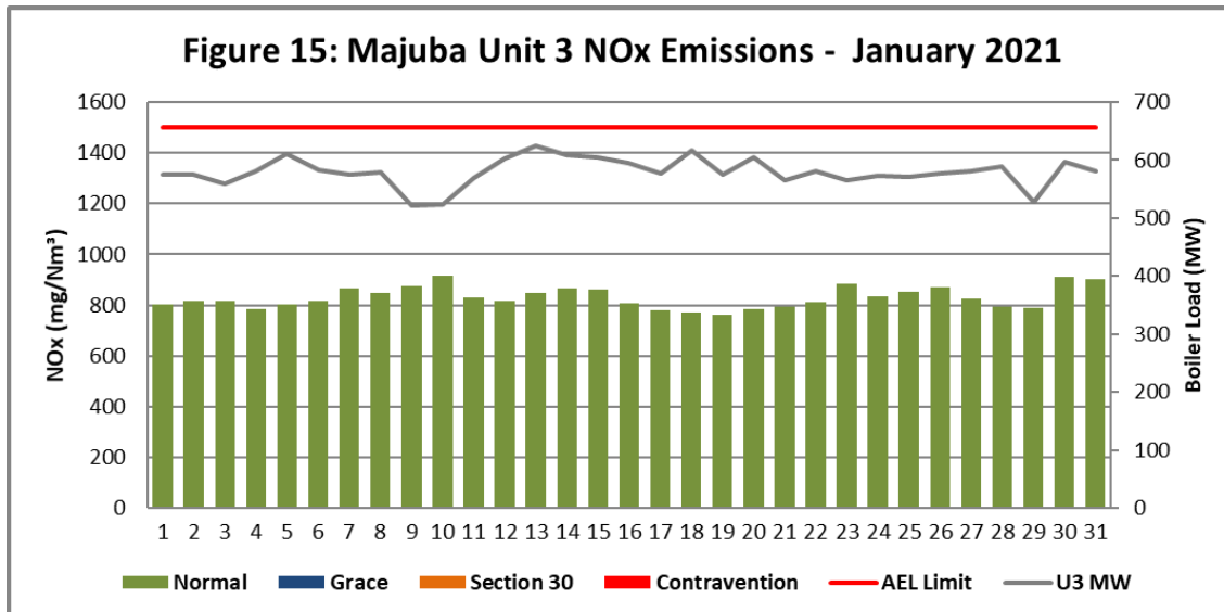
Figure 15. NOx emissions (daily averages) for the month of January 2021 against emission limit for Unit 3.
