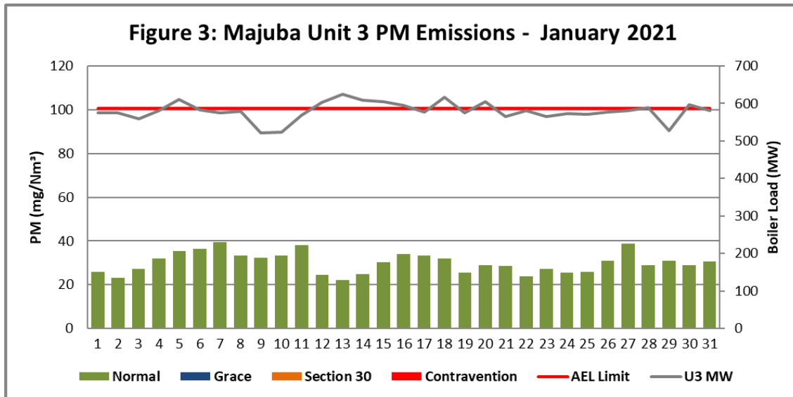
Figure 3. Particulate Matter emissions (daily averages) for the month of January 2021 against emission limit for Unit 3.
