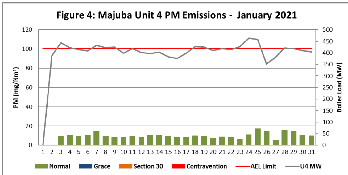
Figure 4. Particulate Matter emissions (daily averages) for the month of January 2021 against emission limit for Unit 4.
