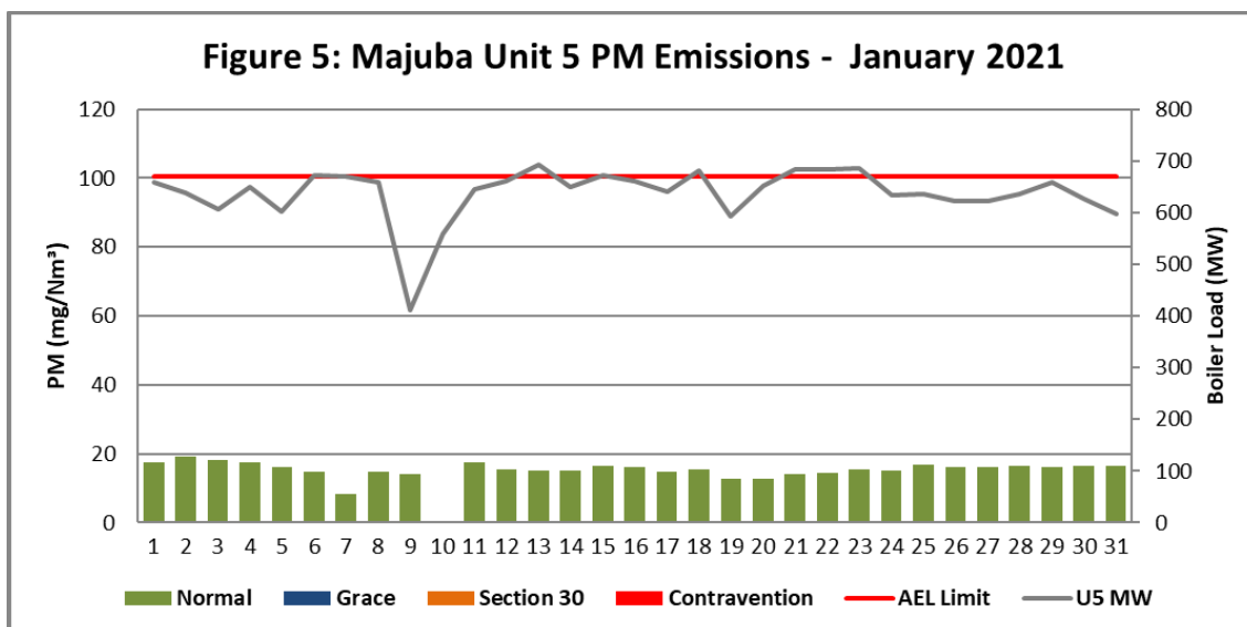
Figure 5. Particulate Matter emissions (daily averages) for the month of January 2021 against emission limit for Unit 5.
