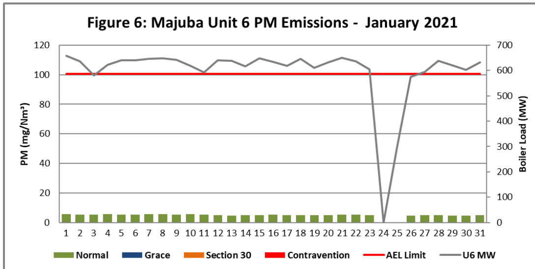
Figure 6. Particulate Matter emissions (daily averages) for the month of January 2021 against emission limit for Unit 6.
