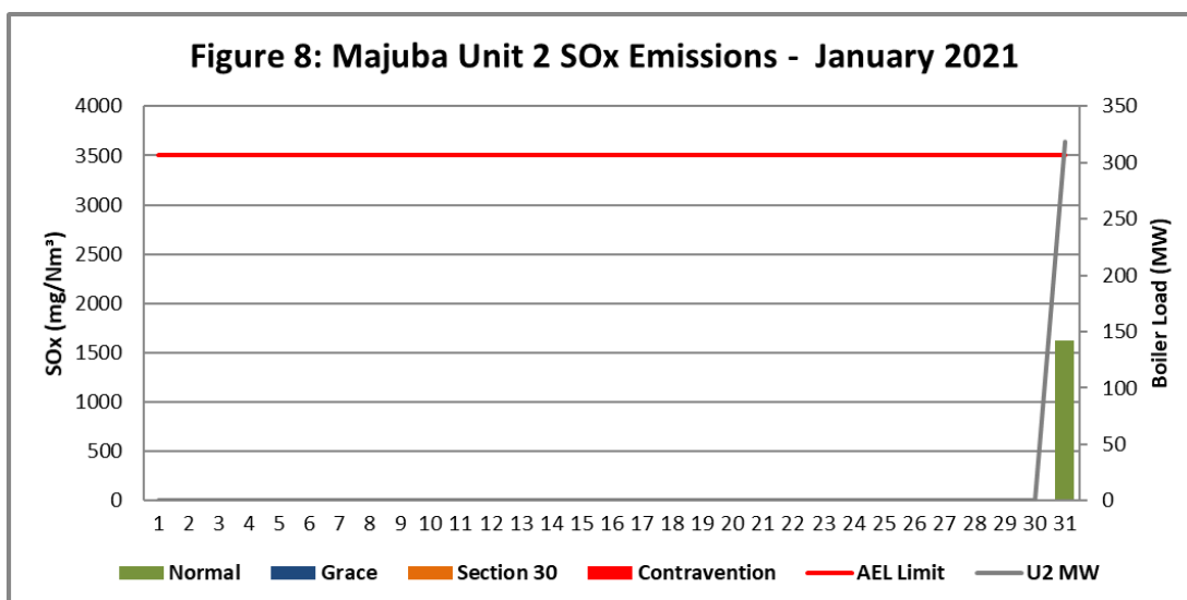
Figure 8. SOx emissions (daily averages) for the month of January 2021 against emission limit for Unit 2. The unit was on outage for most of the month and was returned to service on 30 January 2021.
