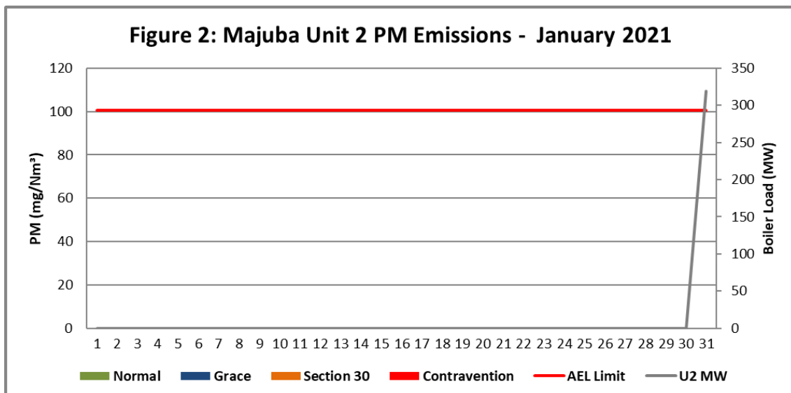
Figure 2. Particulate Matter emissions (daily averages) for the month of January 2021 against emission limit for Unit 2. The unit was on outage for most of the month and was returned to service on 30 January 2021.
