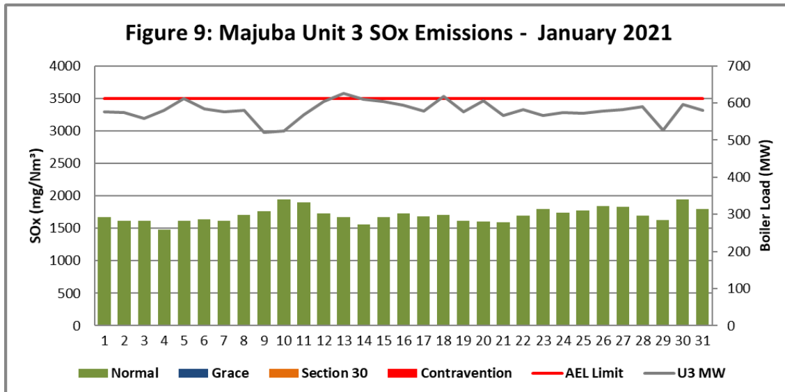
Figure 9. SOx emissions (daily averages) for the month of January 2021 against emission limit for Unit 3.
