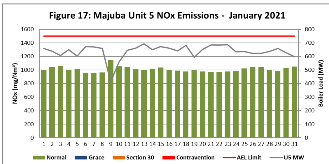
Figure 17. NOx emissions (daily averages) for the month of January 2021 against emission limit for Unit 5
