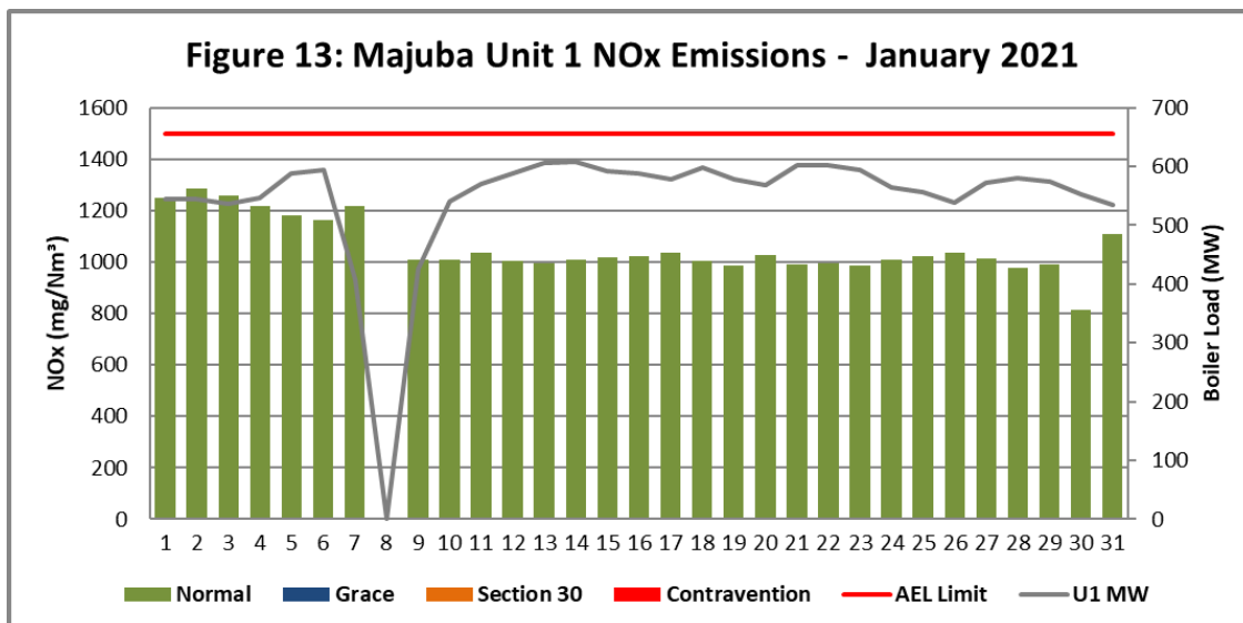
Figure 13. NOx emissions (daily averages) for the month of January 2021 against emission limit for Unit 1.
