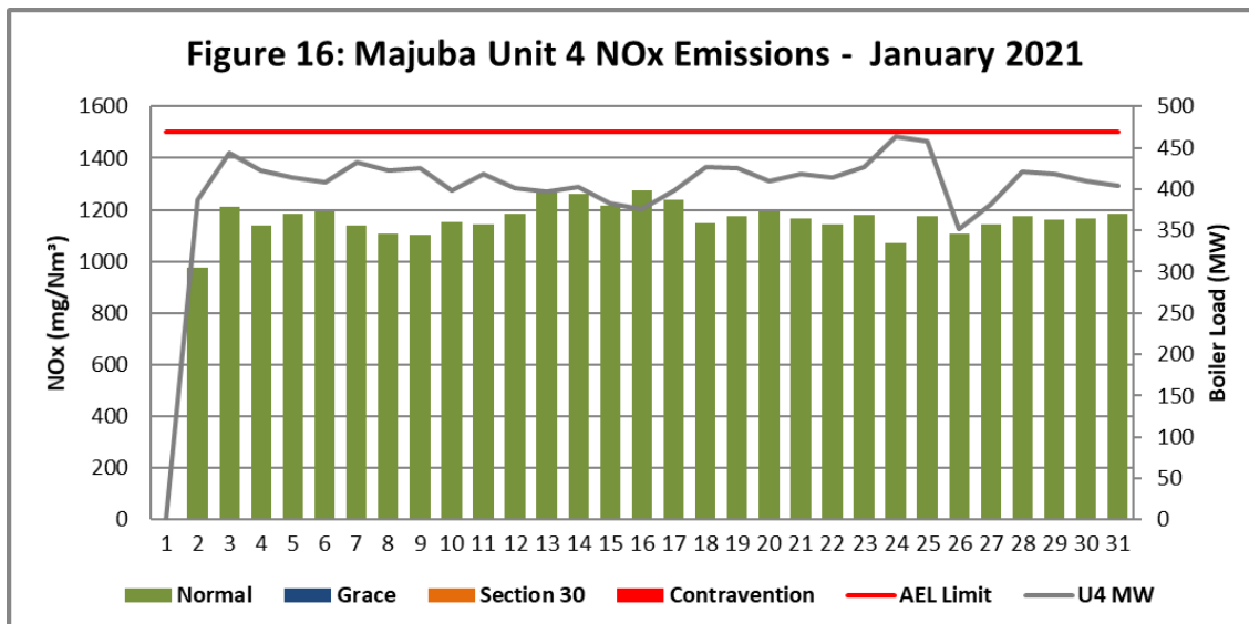
Figure 16. NOx emissions (daily averages) for the month of January 2021 against emission limit for Unit 4
