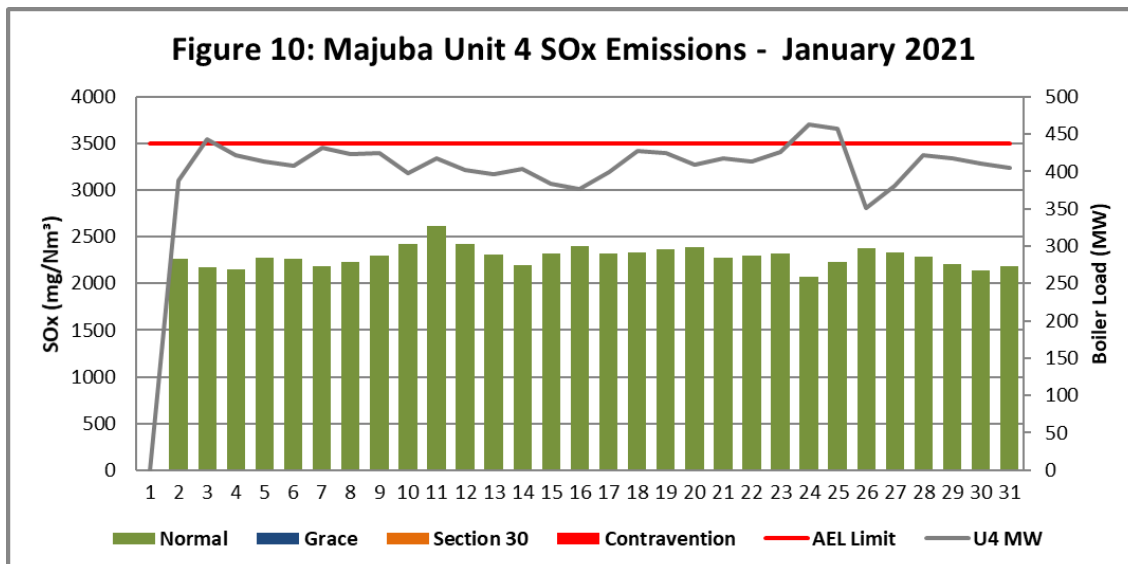
Figure 10. SOx emissions (daily averages) for the month of January 2021 against emission limit for Unit 4.
