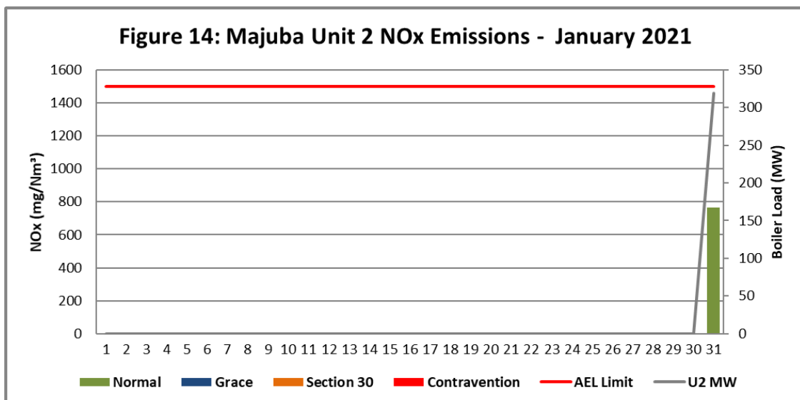
Figure 14. NOx emissions (daily averages) for the month of January 2021 against emission limit for Unit 2. The unit was on outage for most of the month and was returned to service on 30 January 2021.
