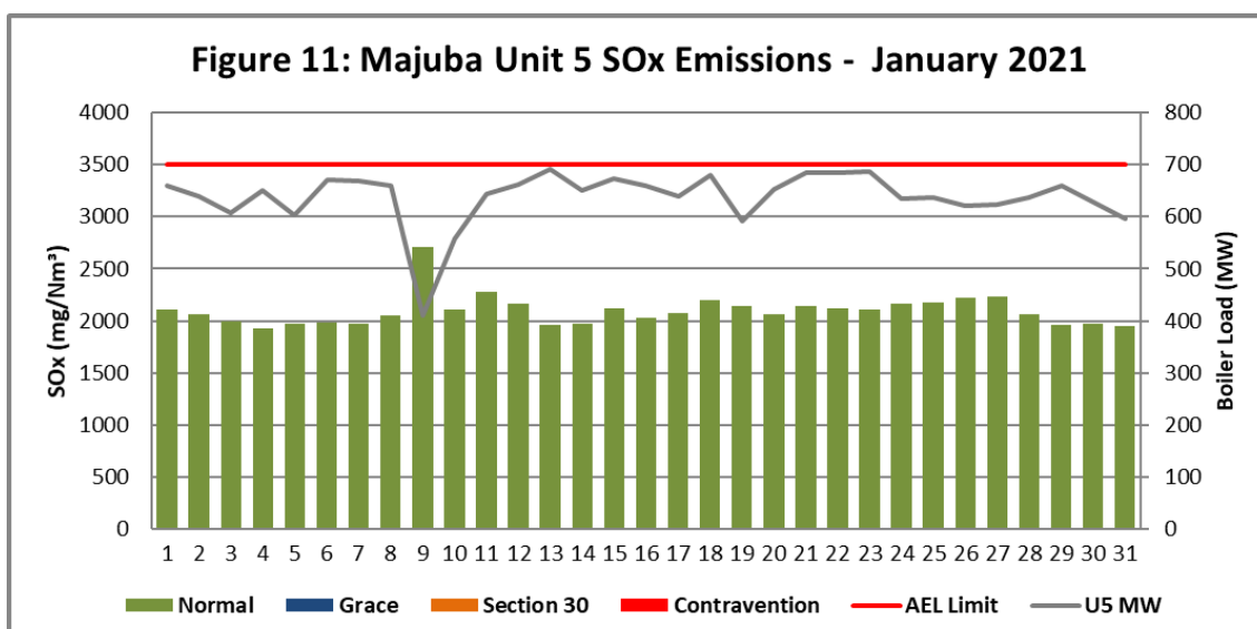
Figure 11. SOx emissions (daily averages) for the month of January 2021 against emission limit for Unit 5.
