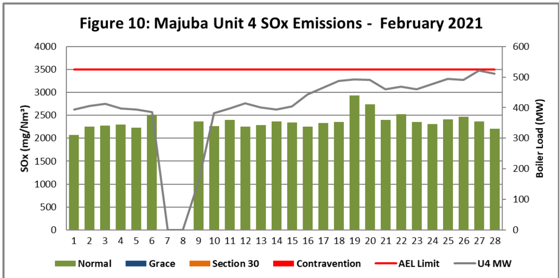
Figure 10. SOx emissions (daily averages) for the month of February 2021 against emission limit for Unit 4.
