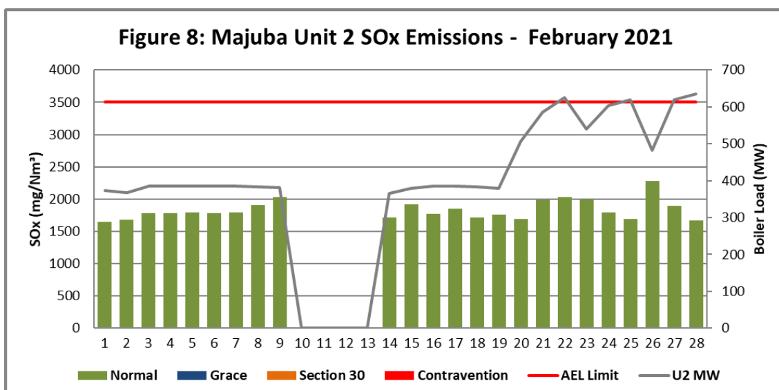
Figure 8. SOx emissions (daily averages) for the month of February 2021 against emission limit for Unit 2.
