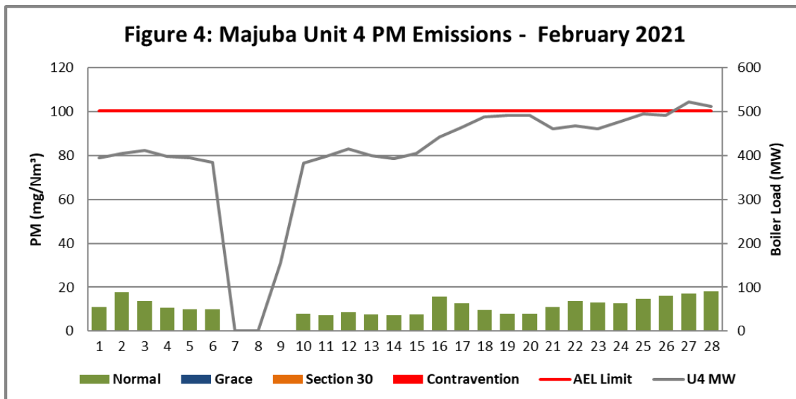
Figure 4. Particulate Matter emissions (daily averages) for the month of February 2021 against emission limit for Unit 4.
