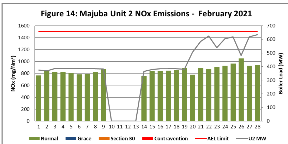
Figure 14. NOx emissions (daily averages) for the month of February 2021 against emission limit for Unit 2.
