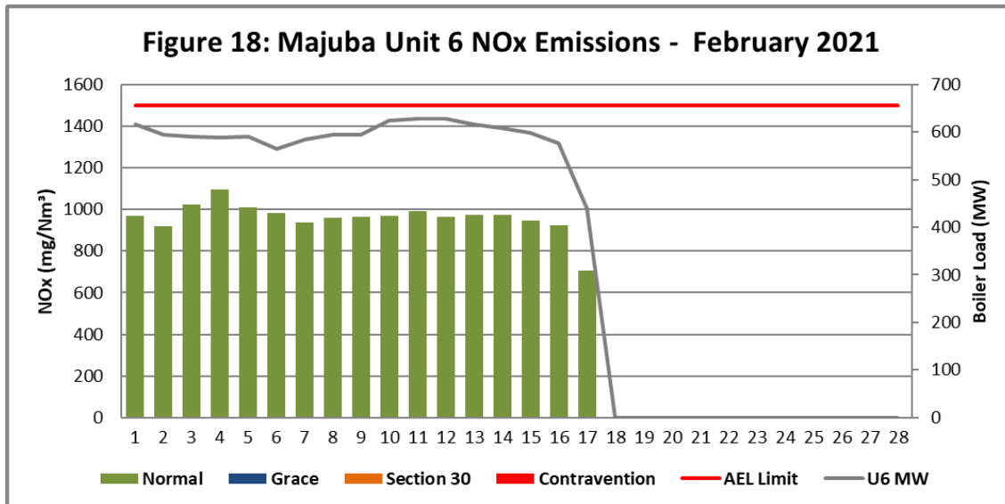
Figure 18. NOx emissions (daily averages) for the month February 2021 against emission limit for Unit 6
