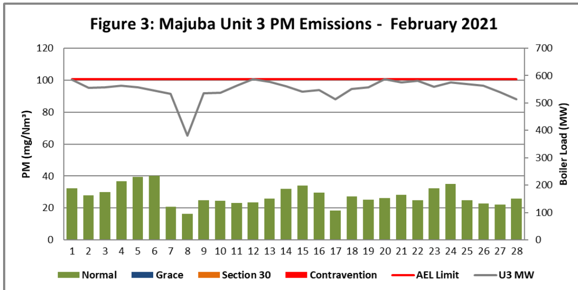
Figure 3. Particulate Matter emissions (daily averages) for the month of February 2021 against emission limit for Unit 3.
