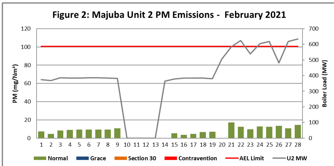
Figure 2. Particulate Matter emissions (daily averages) for the month of February 2021 against emission limit for Unit 2.
