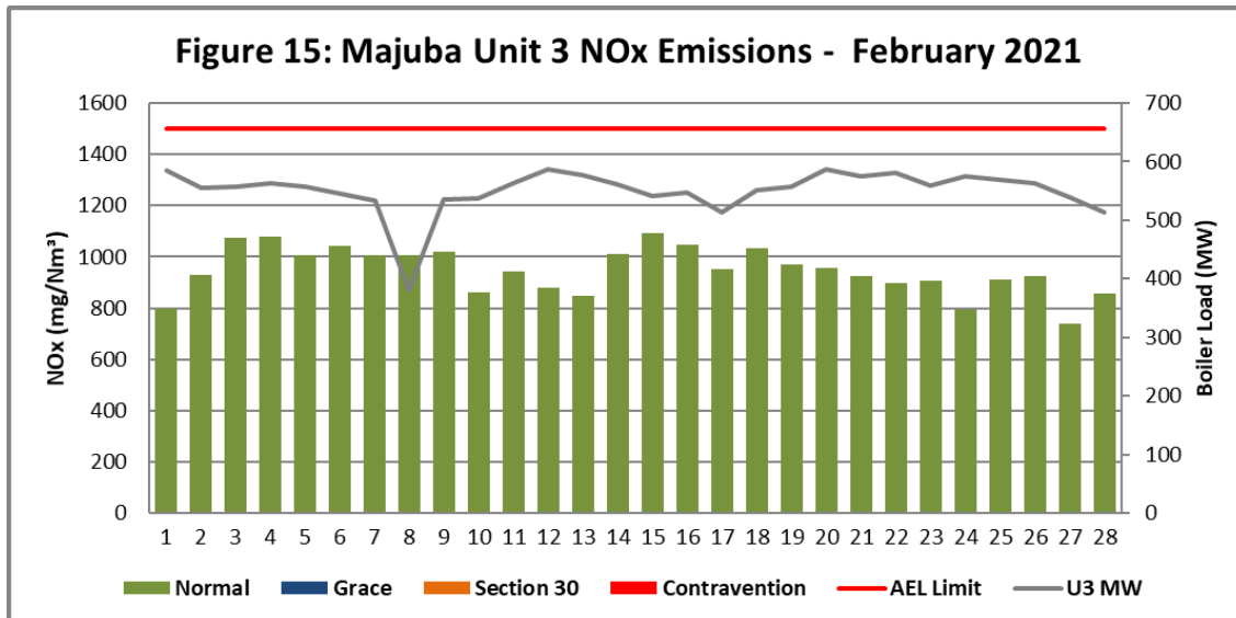
Figure 15. NOx emissions (daily averages) for the month of February 2021 against emission limit for Unit 3.
