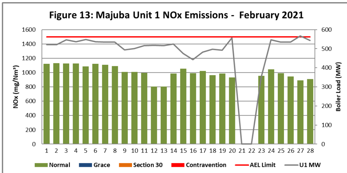
Figure 13. NOx emissions (daily averages) for the month of February 2021 against emission limit for Unit 1.
