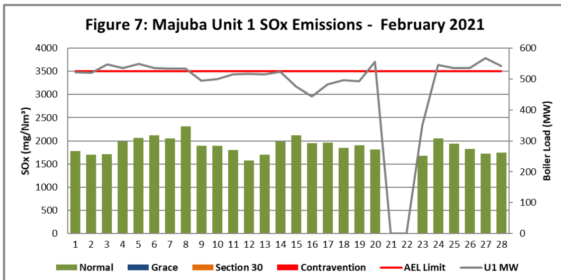
Figure 7. SOx emissions (daily averages) for the month of February 2021 against emission limit for Unit 1.
