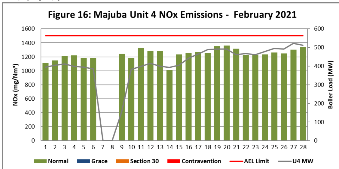
Figure 16. NOx emissions (daily averages) for the month of February 2021 against emission limit for Unit 4
