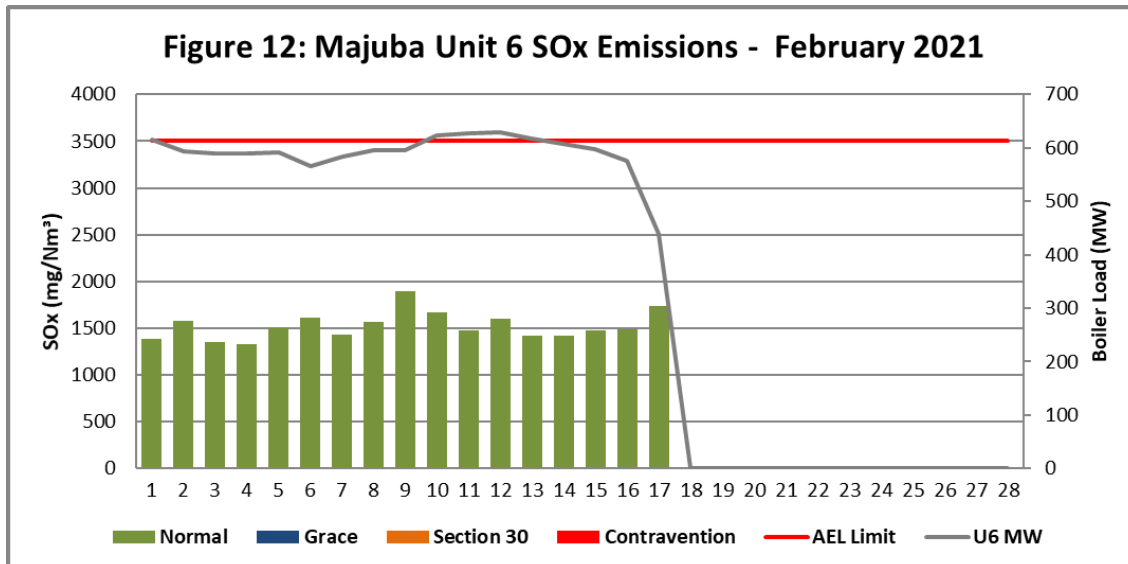
Figure 12. SOx emissions (daily averages) for the month of February 2021 against emission limit for Unit 6.
