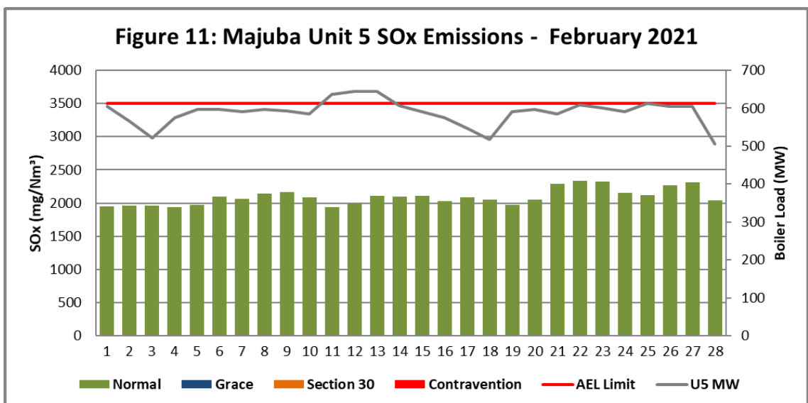
Figure 11. SOx emissions (daily averages) for the month of February 2021 against emission limit for Unit 5.
