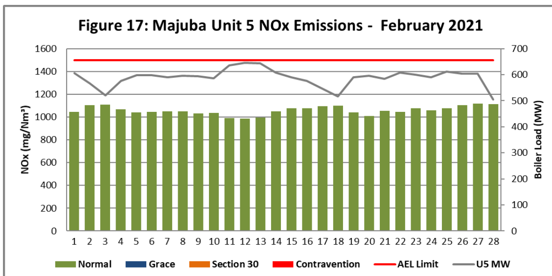
Figure 17. NOx emissions (daily averages) for the month of February 2021 against emission limit for Unit 5
