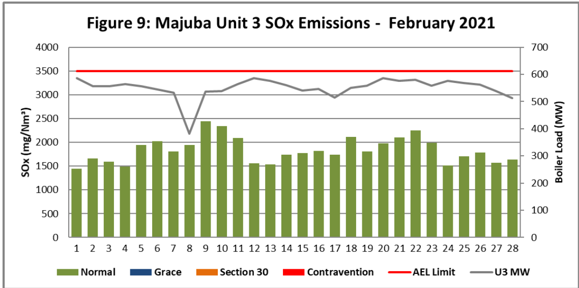
Figure 9. SOx emissions (daily averages) for the month of February 2021 against emission limit for Unit 3.
