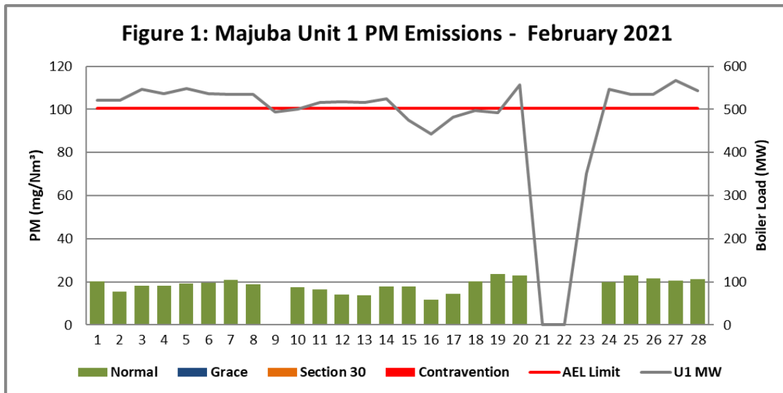
Figure 1. Particulate Matter emissions (daily averages) for the month of February 2021 against emission limit for Unit 1.
