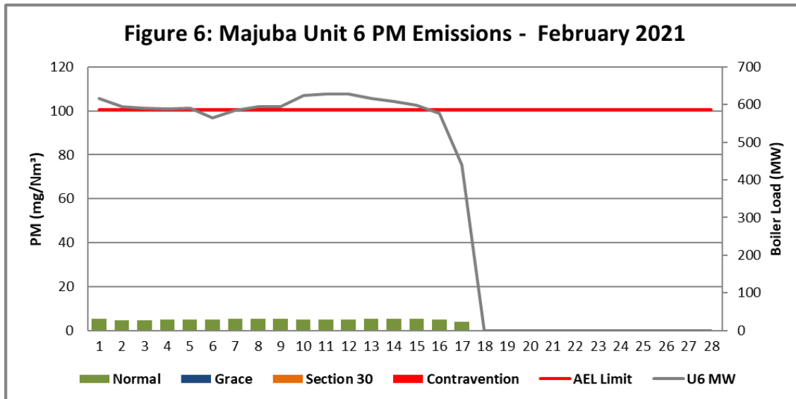
Figure 6. Particulate Matter emissions (daily averages) for the month of February 2021 against emission limit for Unit 6.
