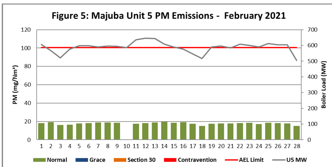
Figure 5. Particulate Matter emissions (daily averages) for the month of February 2021 against emission limit for Unit 5.
