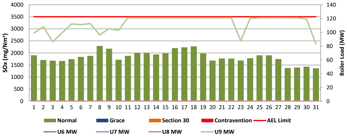
Figure 4: Komati West Stack SOx Emissions - July 2021
