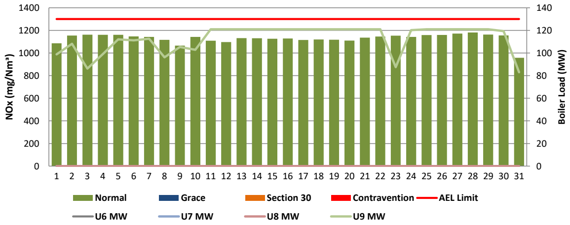
Figure 6: Komati West Stack NOx Emissions - July 2021
