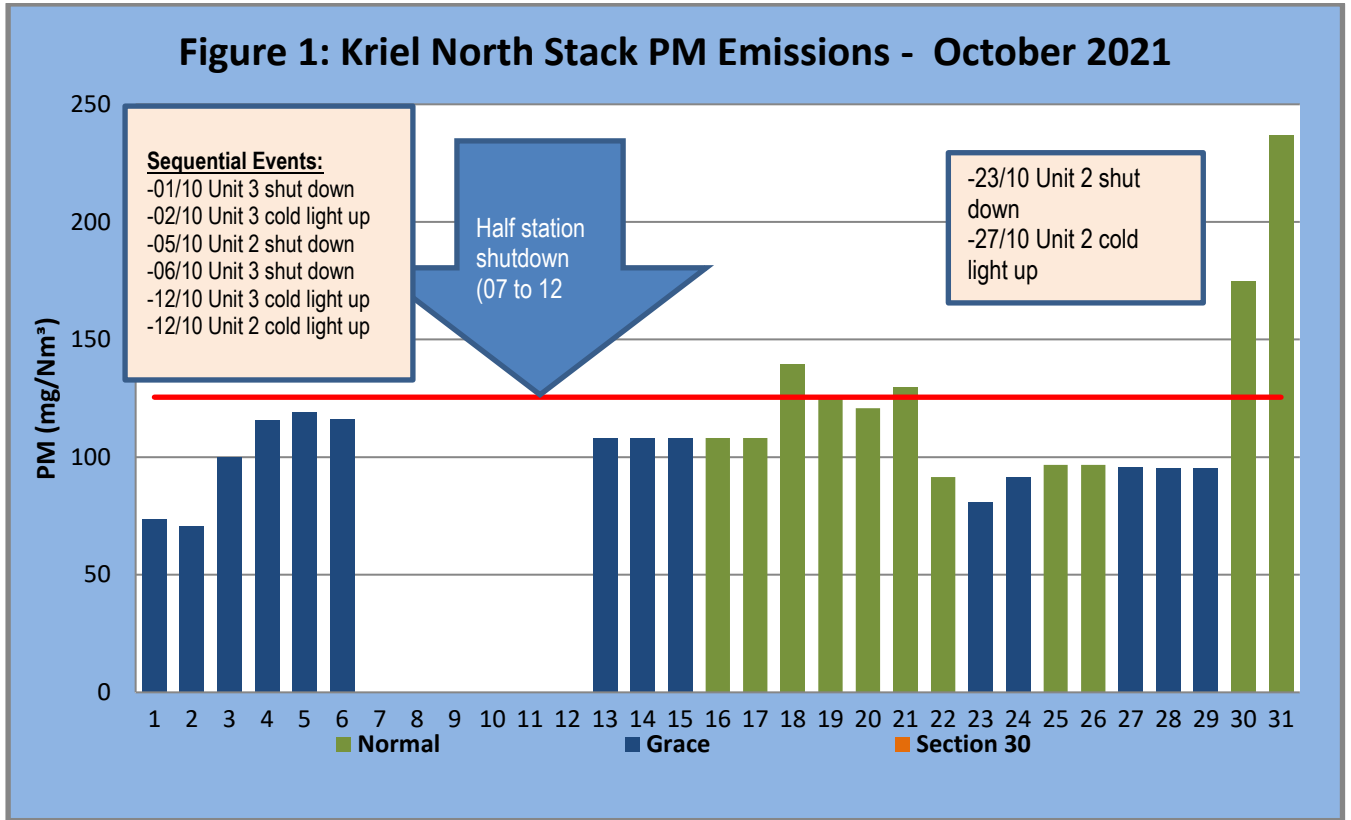
Figure 1: PM emissions for the month of October 2021 against emission limit for the North Stack. Monthly average was 112.2 mg/Nm 3
