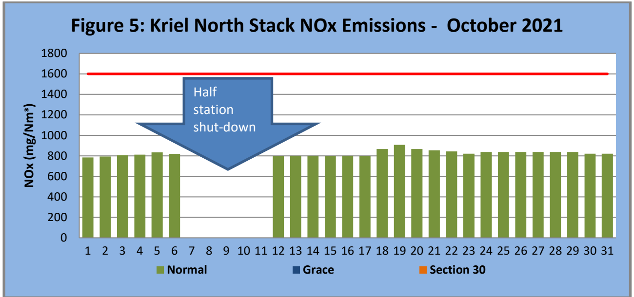
Figure 5. NO x emissions for the month of October 2021 against emission limit for the North Stack. The NO x Limit is 1600mg/Nm 3 .
