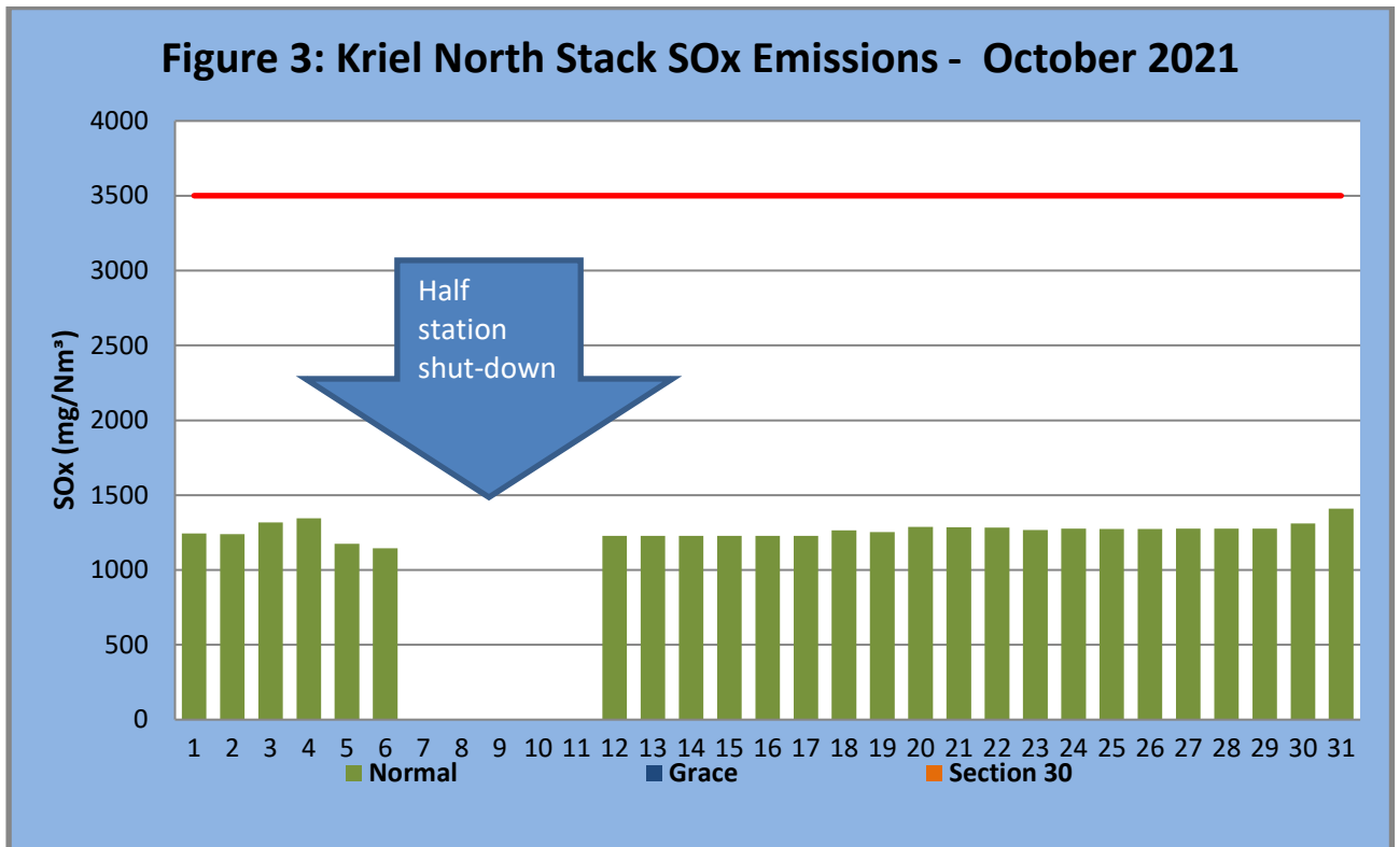
Figure 3. SO 2 emissions for the month of October 2021 against emission limit for the North Stack. The SO x Limit is 3500mg/Nm 3 .
