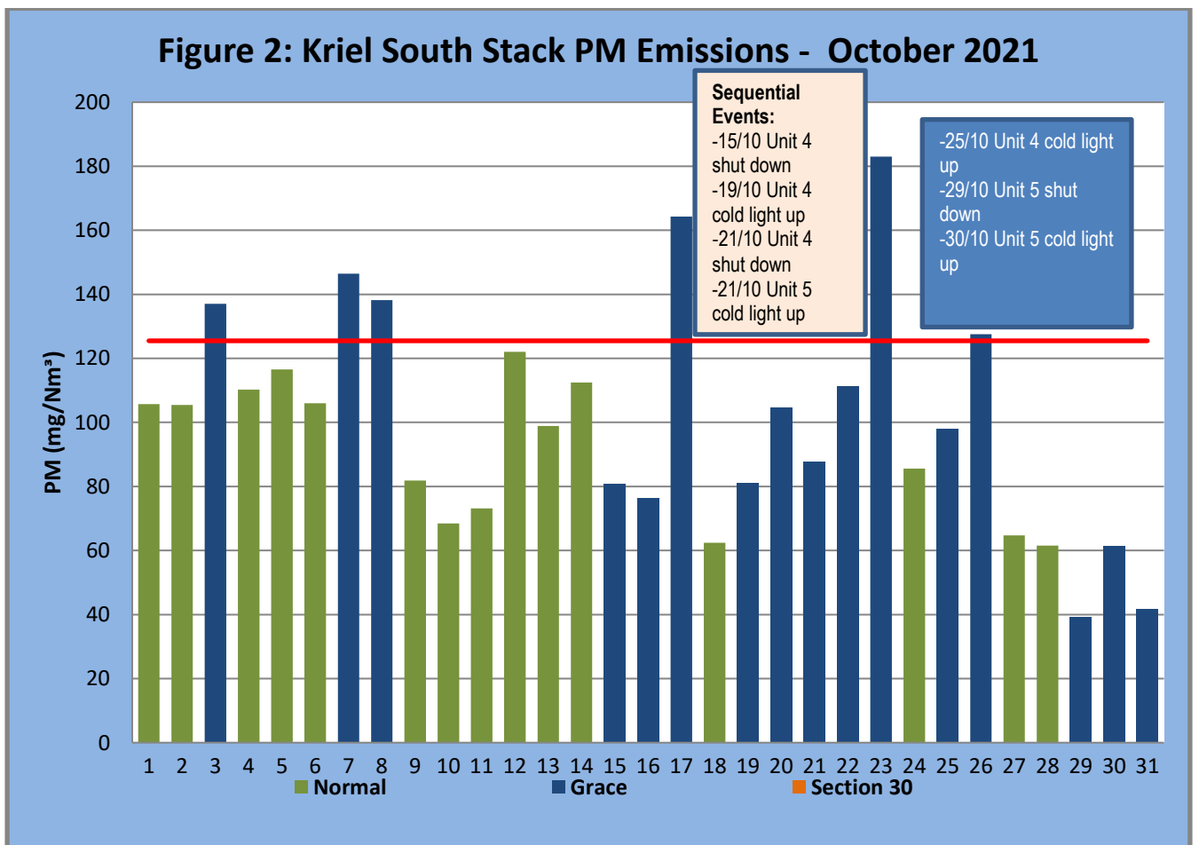
Figure 2: PM emissions for the month of October 2021 against emission limit for the South Stack. Monthly average was 98.5 mg/Nm 3
