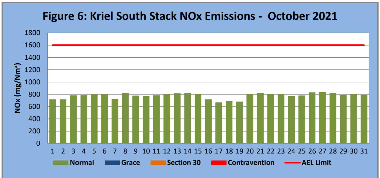
Figure 6. NO x emissions for the month of October 2021 against emission limit for the South Stack. The NO x Limit is 1600mg/Nm 3 .
