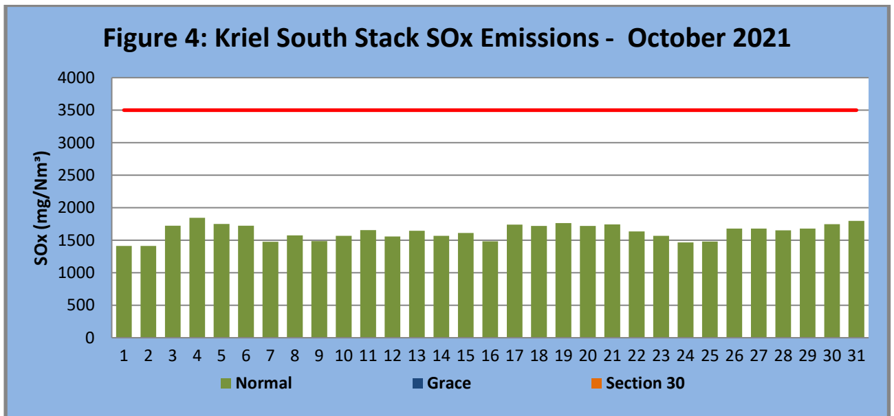
Figure 4. SO 2 emissions for the month of October 2021 against emission limit for the South Stack. The SO x Limit is 3500mg/Nm 3 .
