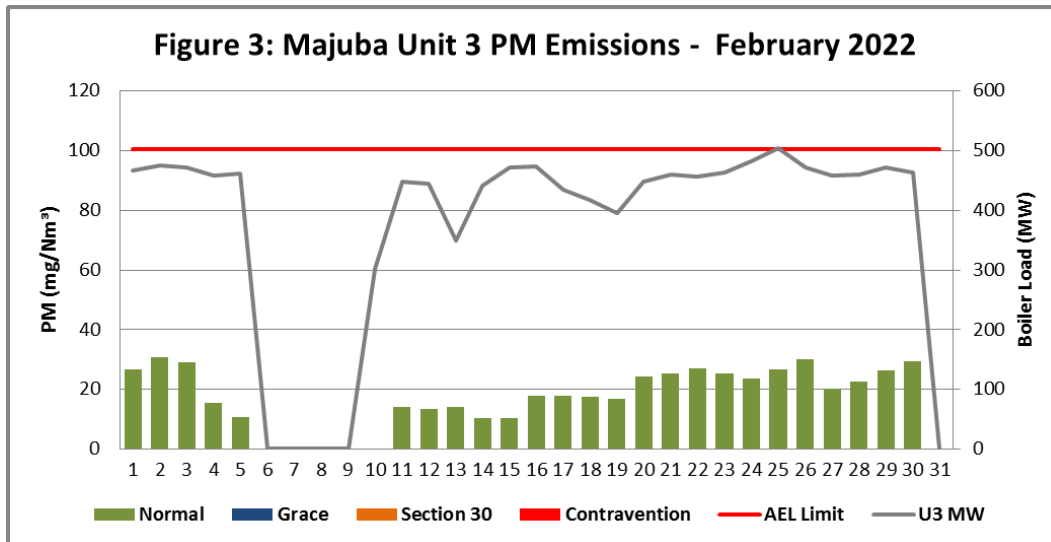
Figure 3. Particulate Matter emissions (daily averages) for the month of February 2022 against emission limit for Unit 3.
