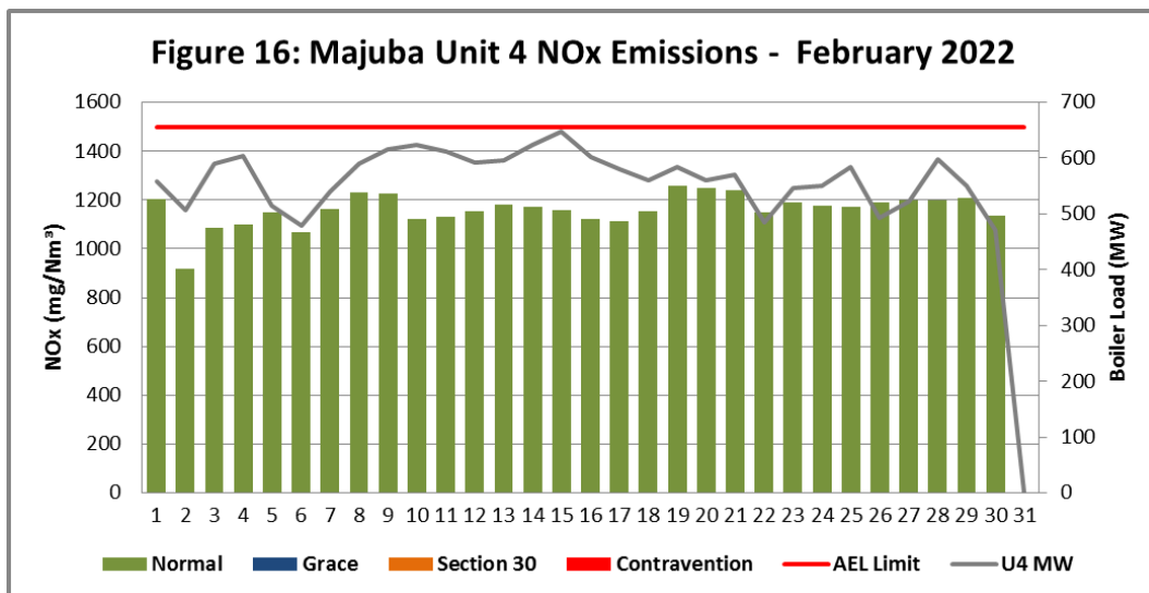
Figure 16. NOx emissions (daily averages) for the month of February 2022 against emission limit for Unit 4
