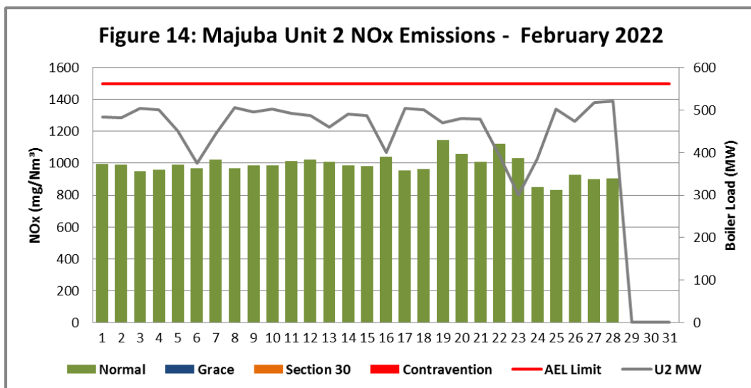
Figure 14. NOx emissions (daily averages) for the month of February 2022 against emission limit for Unit 2.
