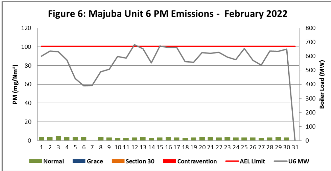
Figure 6. Particulate Matter emissions (daily averages) for the month of February 2022 against emission limit for Unit 6.
