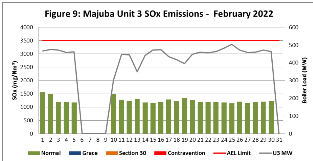
Figure 9. SOx emissions (daily averages) for the month of February 2022 against emission limit for Unit 3.
