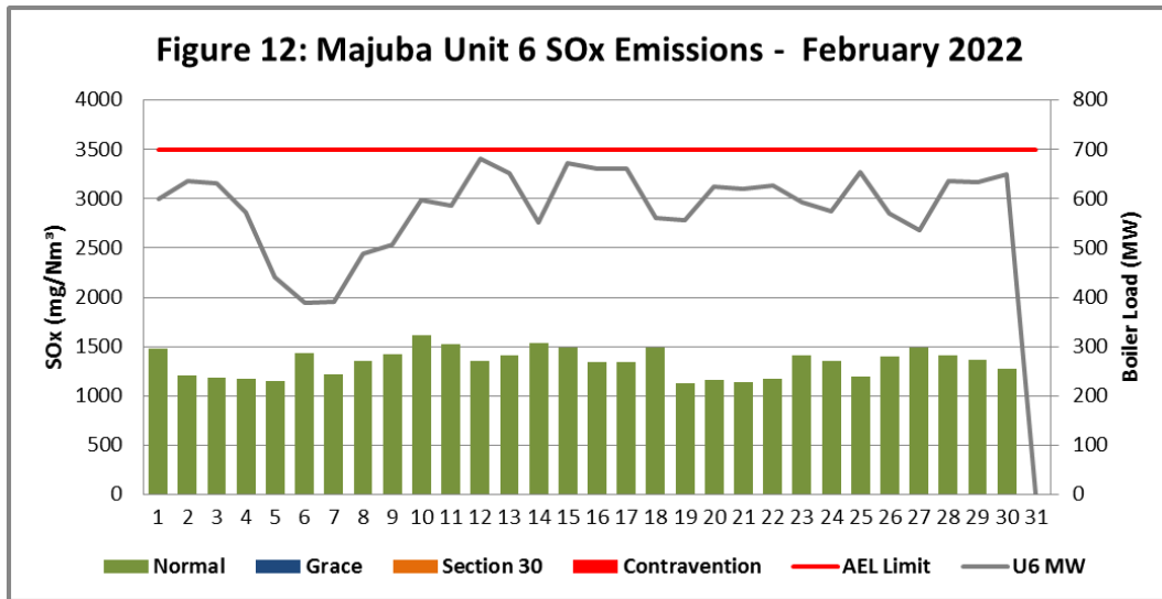
Figure 12. SOx emissions (daily averages) for the month of February 2022 against emission limit for Unit 6.
