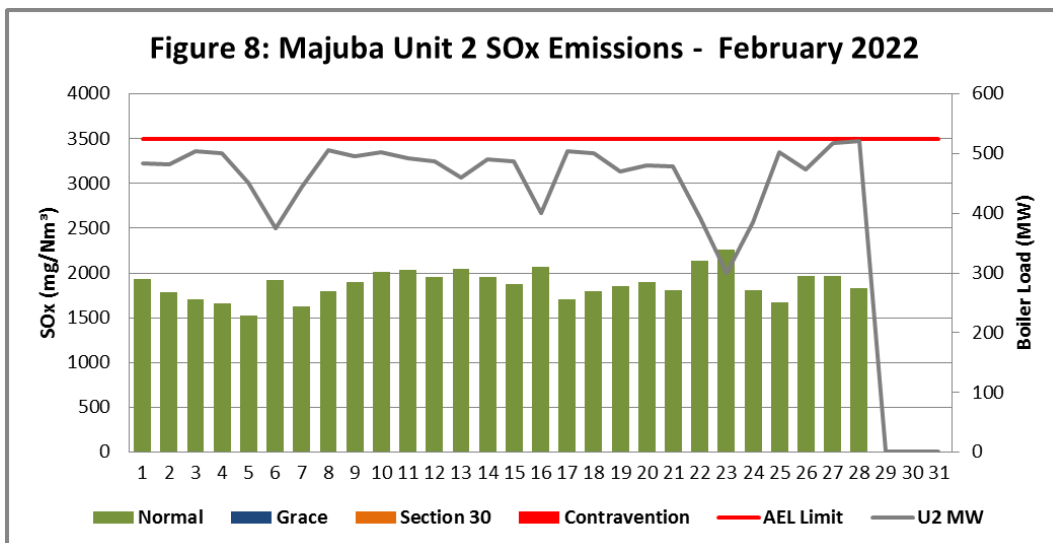
Figure 8. SOx emissions (daily averages) for the month of February 2022 against emission limit for Unit 2.
