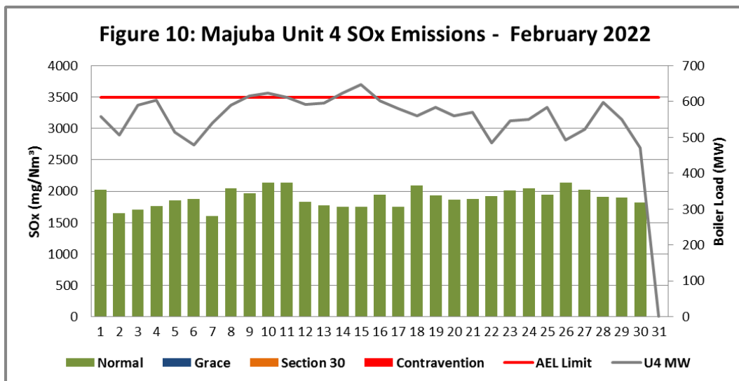
Figure 10. SOx emissions (daily averages) for the month of February 2022 against emission limit for Unit 4.
