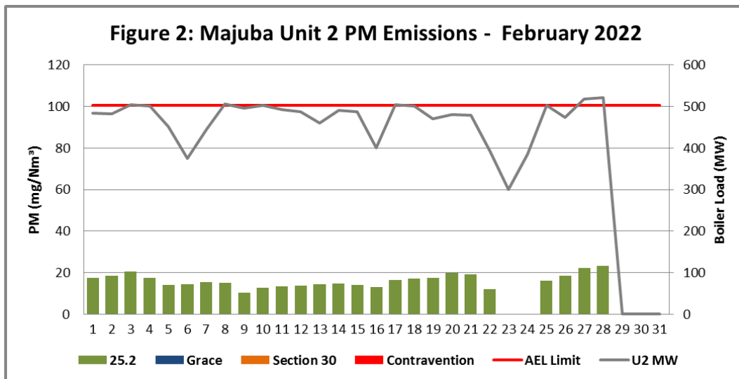
Figure 2. Particulate Matter emissions (daily averages) for the month of February 2022 against emission limit for Unit 2.
