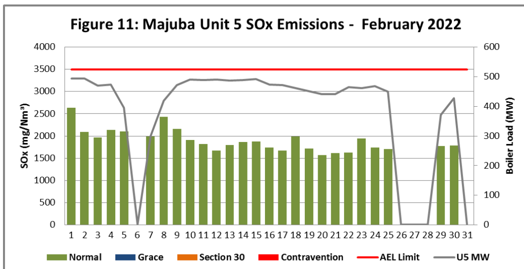
Figure 11. SOx emissions (daily averages) for the month of February 2022 against emission limit for Unit 5.
