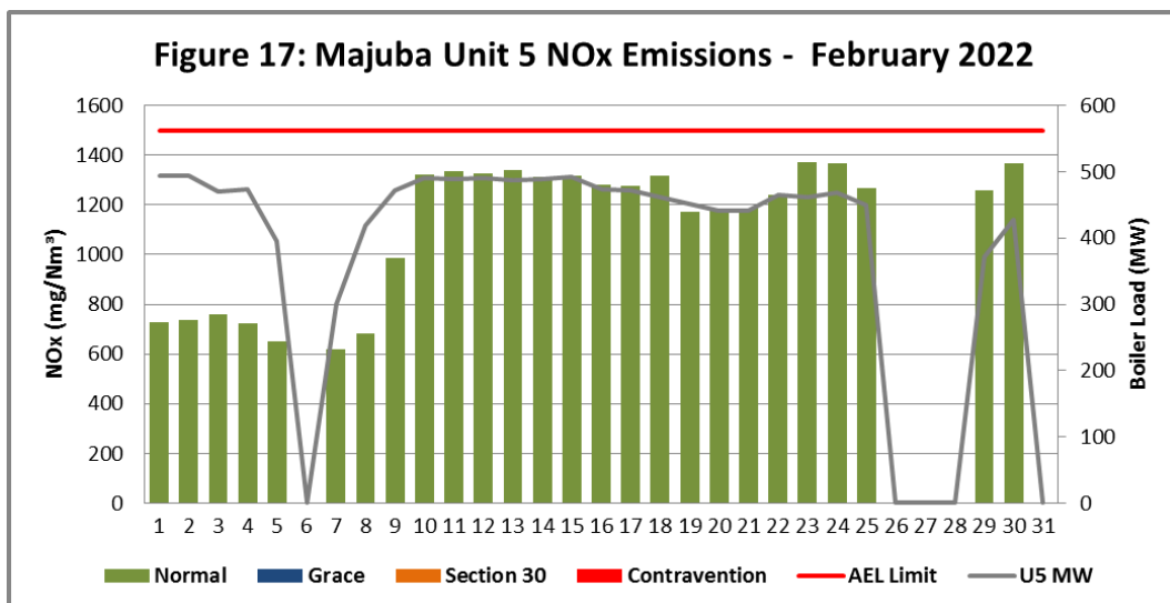
Figure 17. NOx emissions (daily averages) for the month of February 2022 against emission limit for Unit 5
