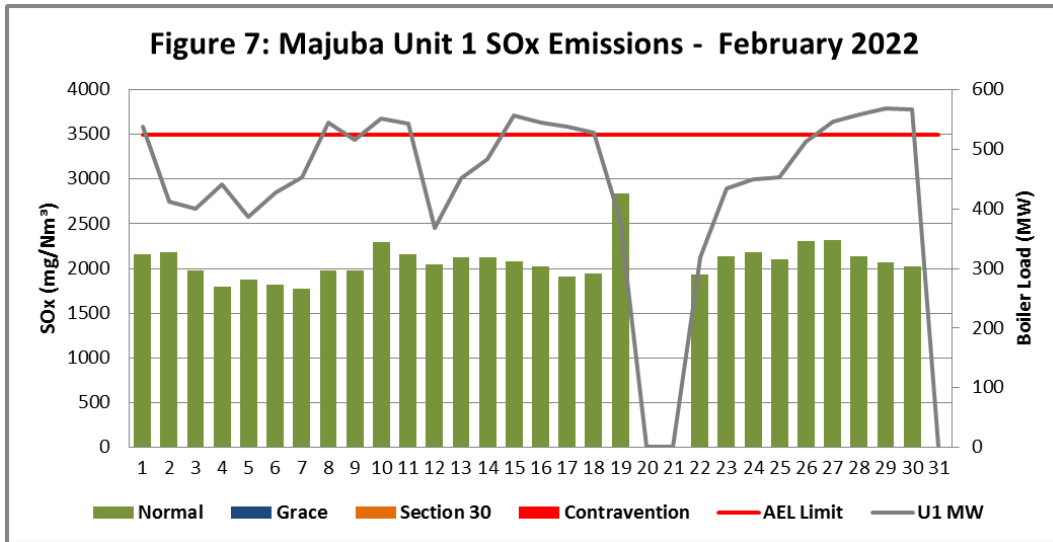
Figure 7. SOx emissions (daily averages) for the month of February 2022 against emission limit for Unit 1.
