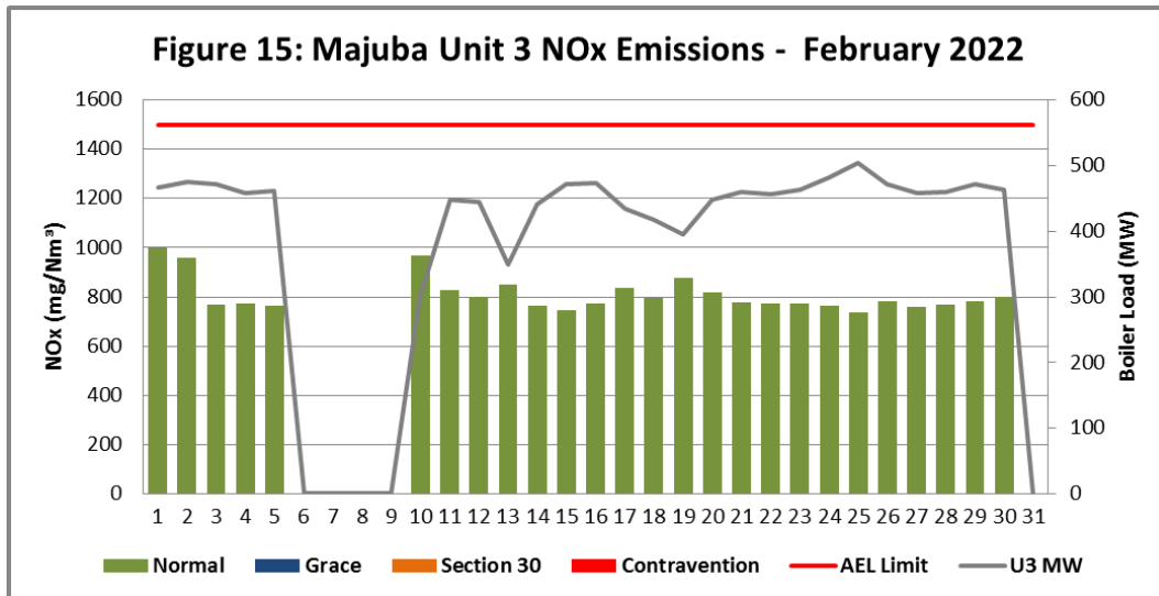
Figure 15. NOx emissions (daily averages) for the month of February 2022 against emission limit for Unit 3.
