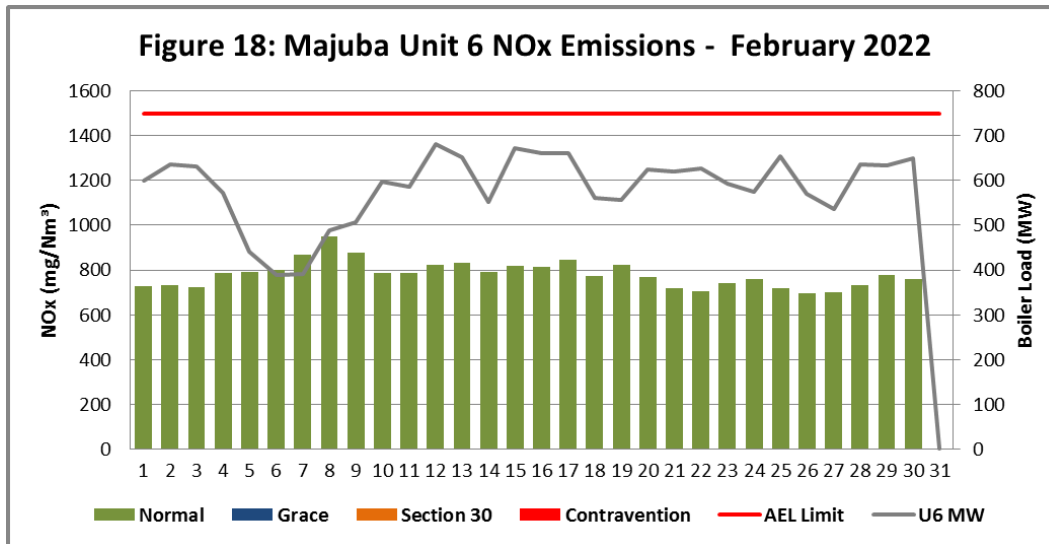
Figure 18. NOx emissions (daily averages) for the month February 2022 against emission limit for Unit 6
