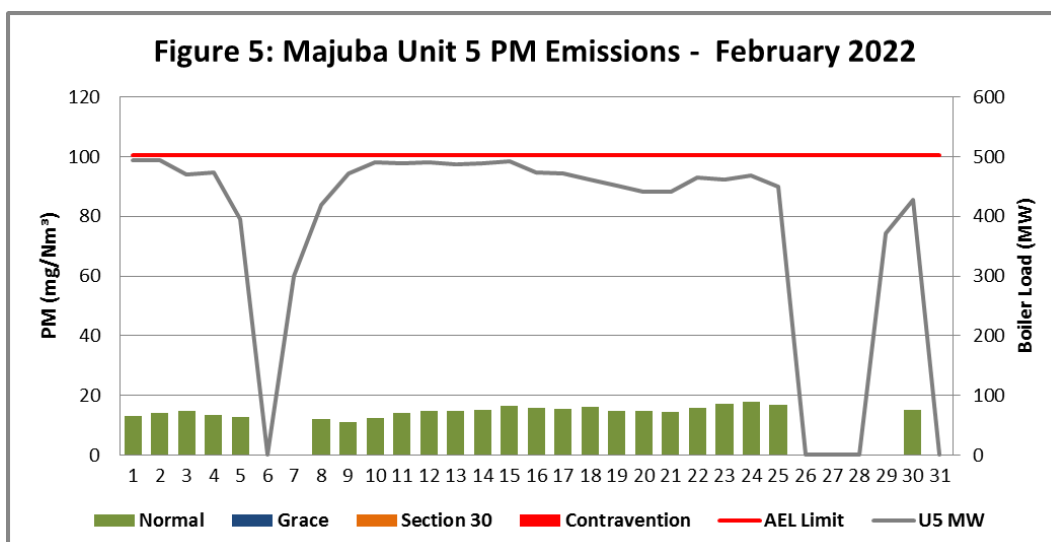
Figure 5. Particulate Matter emissions (daily averages) for the month of February 2022 against emission limit for Unit 5.
