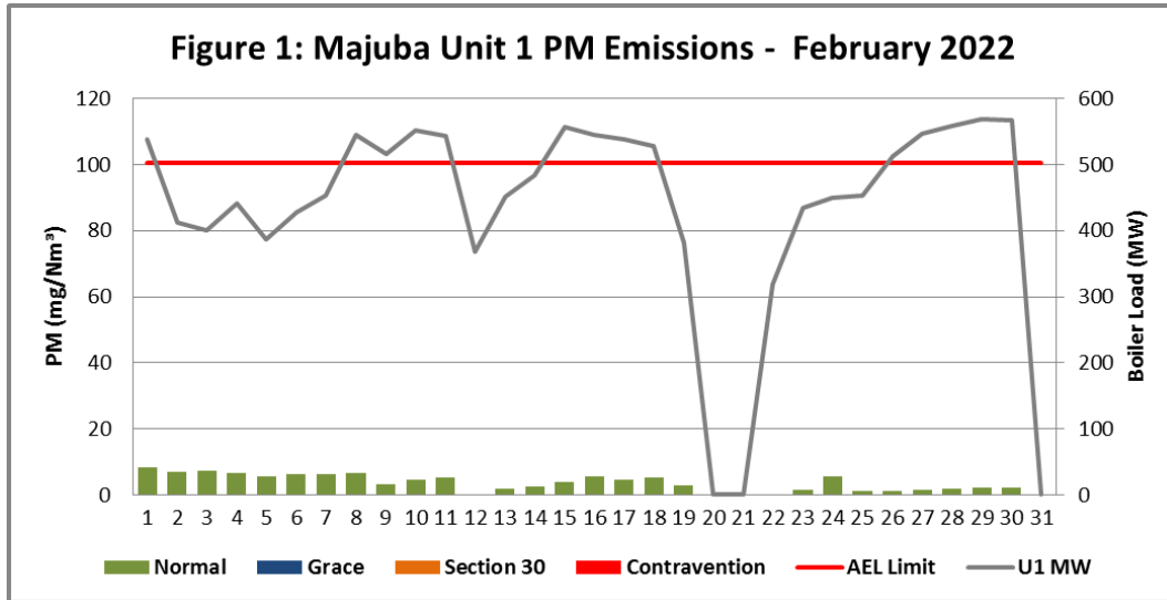
Figure 1. Particulate Matter emissions (daily averages) for the month of February 2022 against emission limit for Unit 1.
