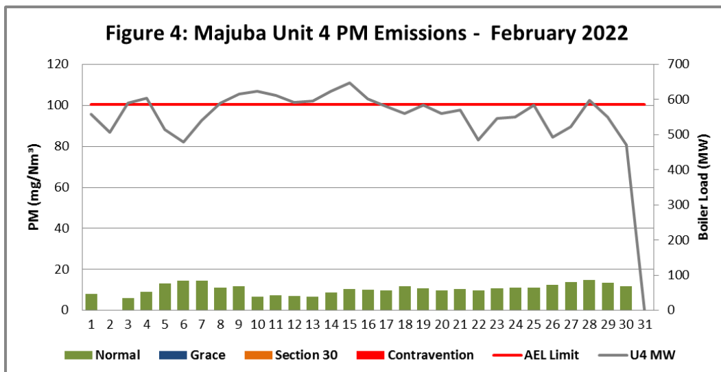
Figure 4. Particulate Matter emissions (daily averages) for the month of February 2022 against emission limit for Unit 4.
