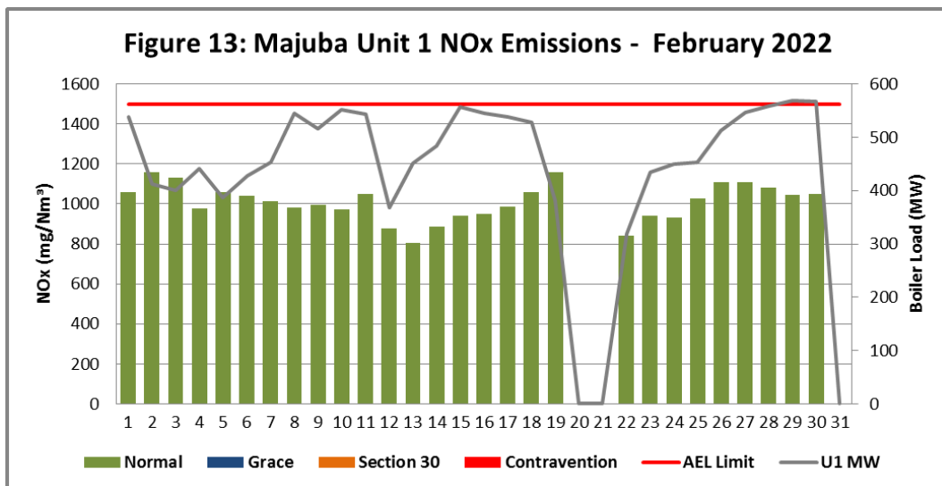
Figure 13. NOx emissions (daily averages) for the month of February 2022 against emission limit for Unit 1.
