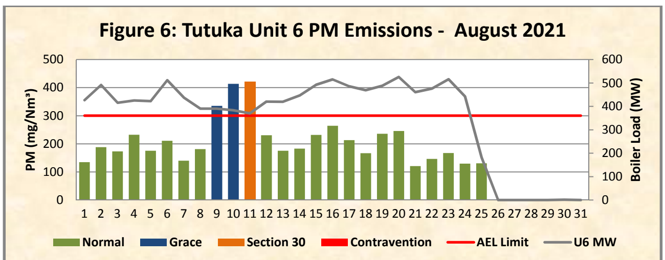
Figure 6: Unit 6 Daily Average PM emissions for the month of August 2021 (against the emission limit and load Generated)
