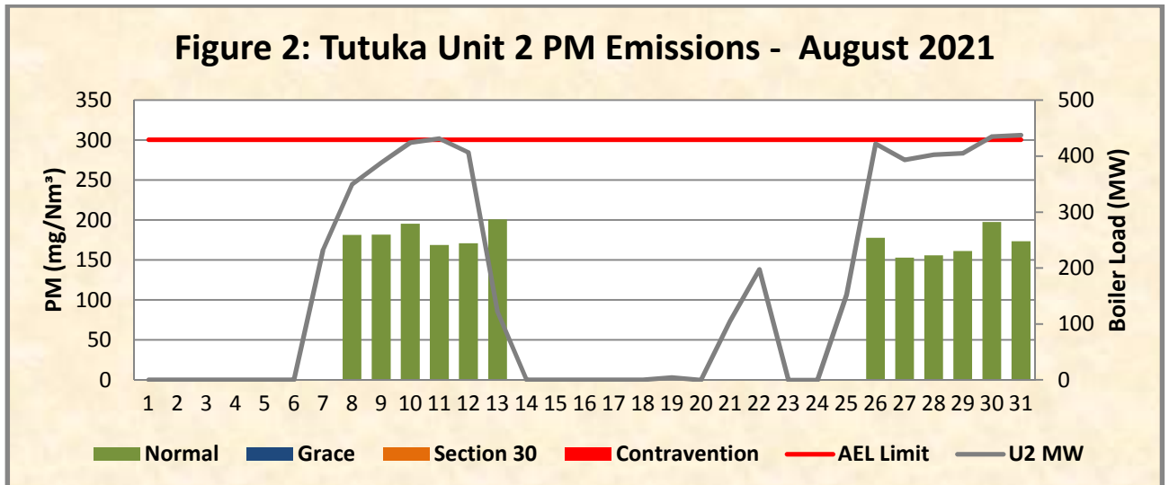
Figure 2: Unit 2 Daily Average PM emissions for the month of August 2021 (against the emission limit and load Generated)
