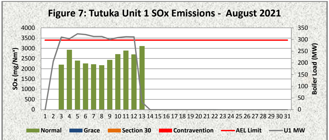
Figure 7: Unit 1 Daily Average SOx emissions for the month of August 2021 (against the emission limit and load Generated)
