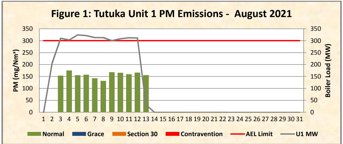
Figure 1: Unit 1 Daily Average PM emissions for the month of August 2021 (against the emission limit and load Generated)
