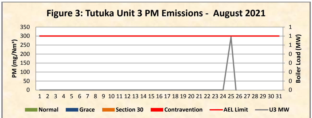
Figure 3: Unit 3 Daily Average PM emissions for the month of August 2021 (against the emission limit and load Generated)
