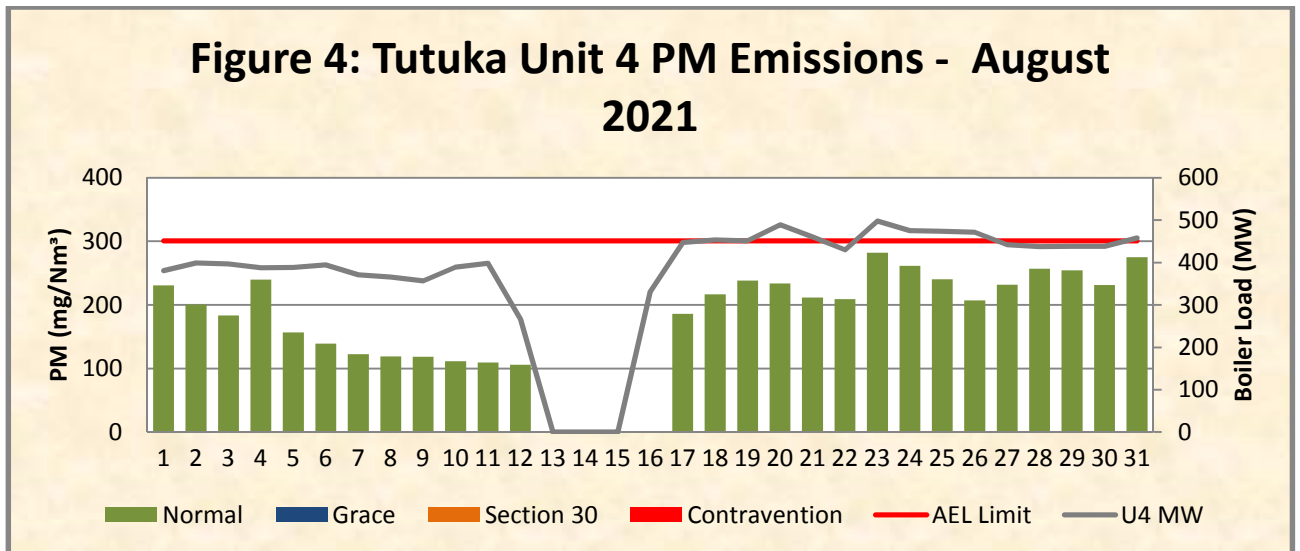
Figure 4: Unit 4 Daily Average PM emissions for the month of August 2021 (against the emission limit and load Generated)
