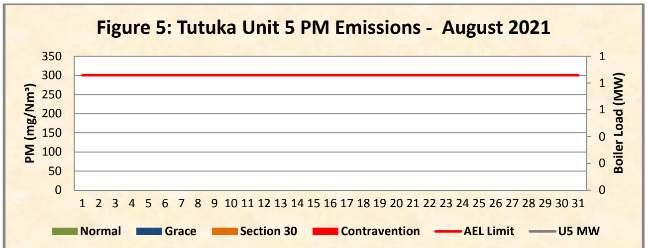
Figure 5: Unit 5 Daily Average PM emissions for the month of August 2021 (against the emission limit and load Generated)
