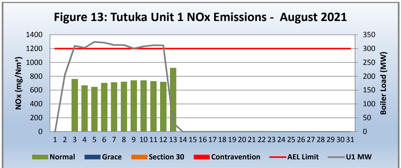
Figure 13: Unit 1 Daily Average NOx emissions for the month of August 2021 (against the emission limit and load Generated)
