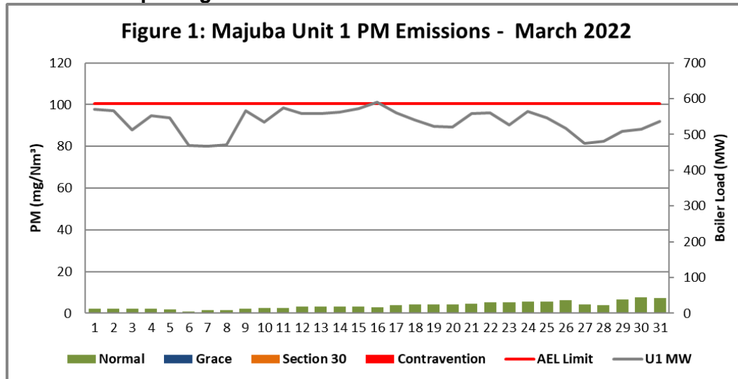
Figure 1. Particulate Matter emissions (daily averages) for the month of March 2022 against emission limit for Unit 1.
