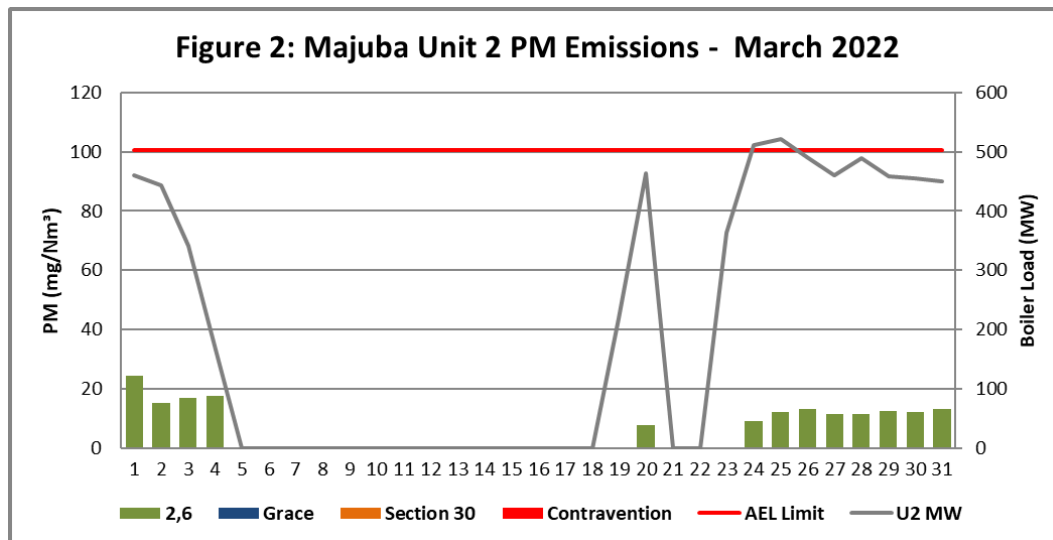
Figure 2. Particulate Matter emissions (daily averages) for the month of March 2022 against emission limit for Unit 2.
