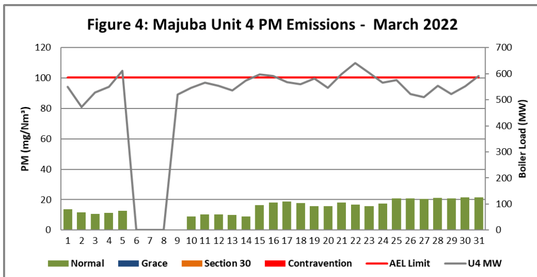
Figure 4. Particulate Matter emissions (daily averages) for the month of March 2022 against emission limit for Unit 4.
