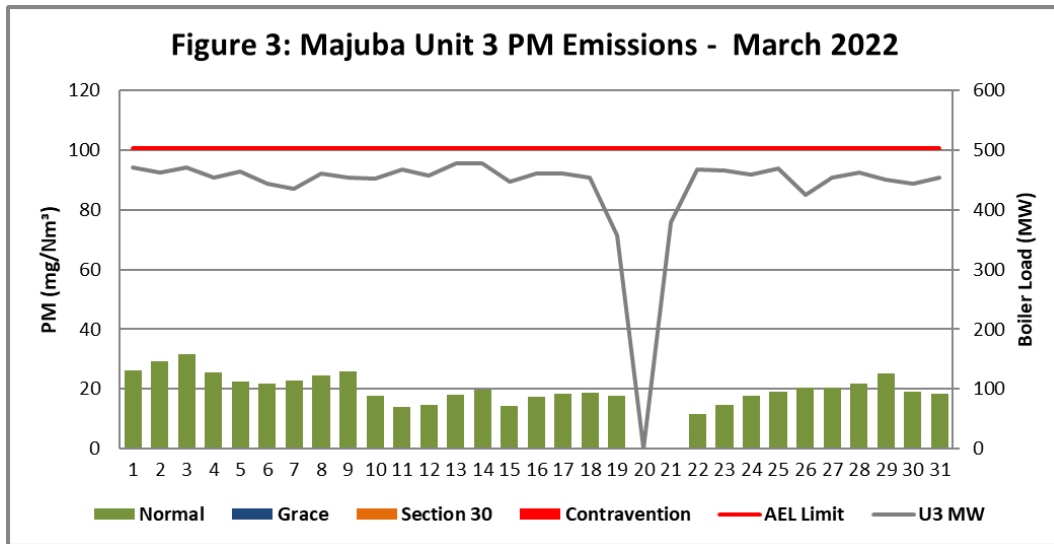
Figure 3. Particulate Matter emissions (daily averages) for the month of March 2022 against emission limit for Unit 3.
