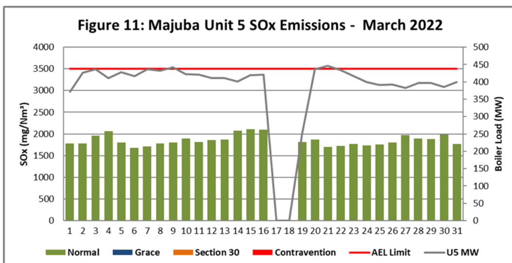
Figure 11. SOx emissions (daily averages) for the month of March 2022 against emission limit for Unit 5.
