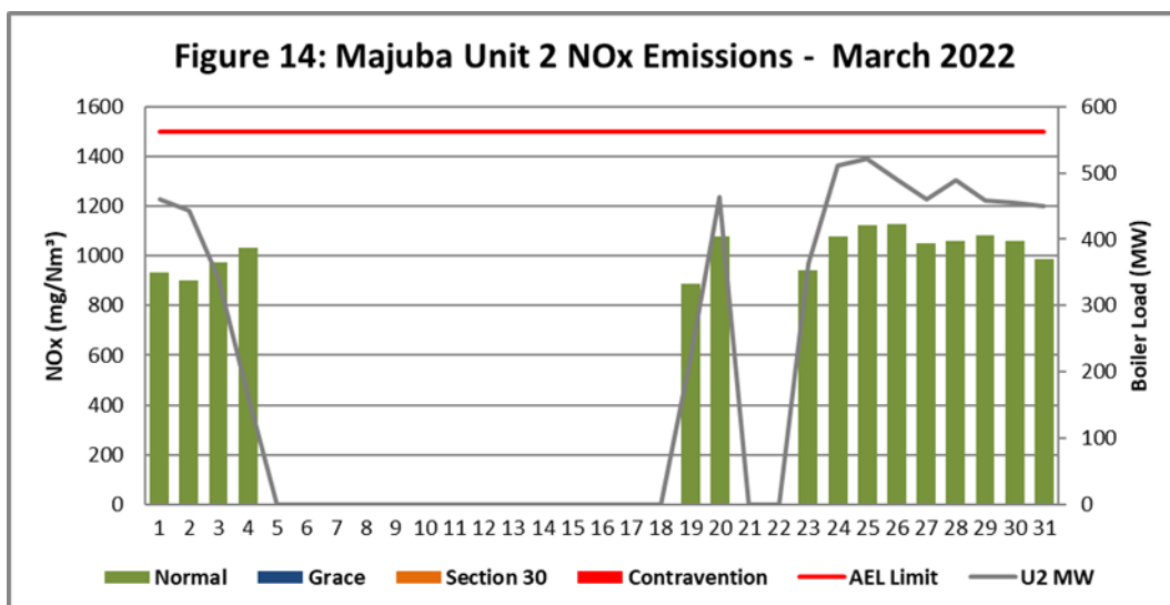
Figure 14. NOx emissions (daily averages) for the month of March 2022 against emission limit for Unit 2.
