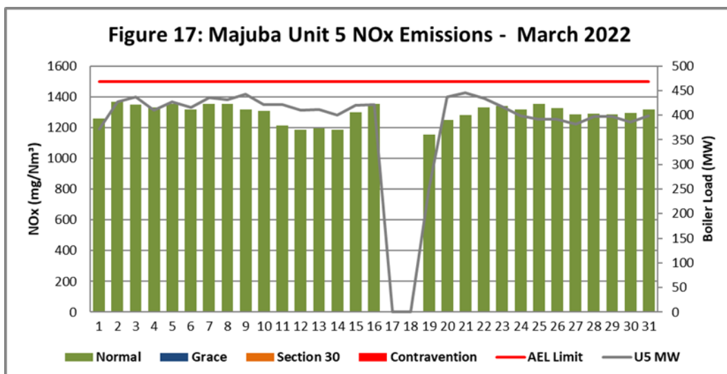
Figure 17. NOx emissions (daily averages) for the month of March 2022 against emission limit for Unit 5
