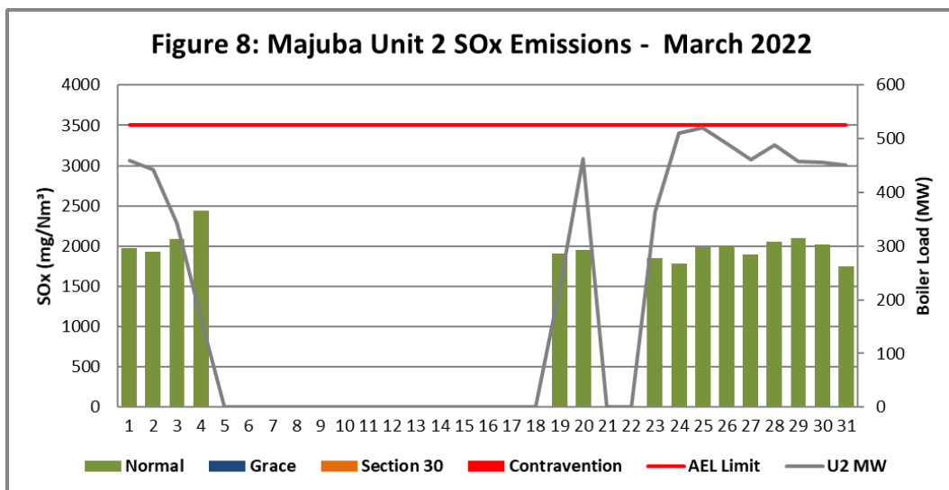
Figure 8. SOx emissions (daily averages) for the month of March 2022 against emission limit for Unit 2.
