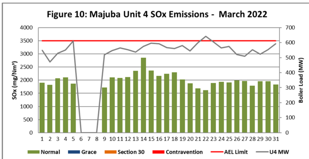
Figure 10. SOx emissions (daily averages) for the month of March 2022 against emission limit for Unit 4.
