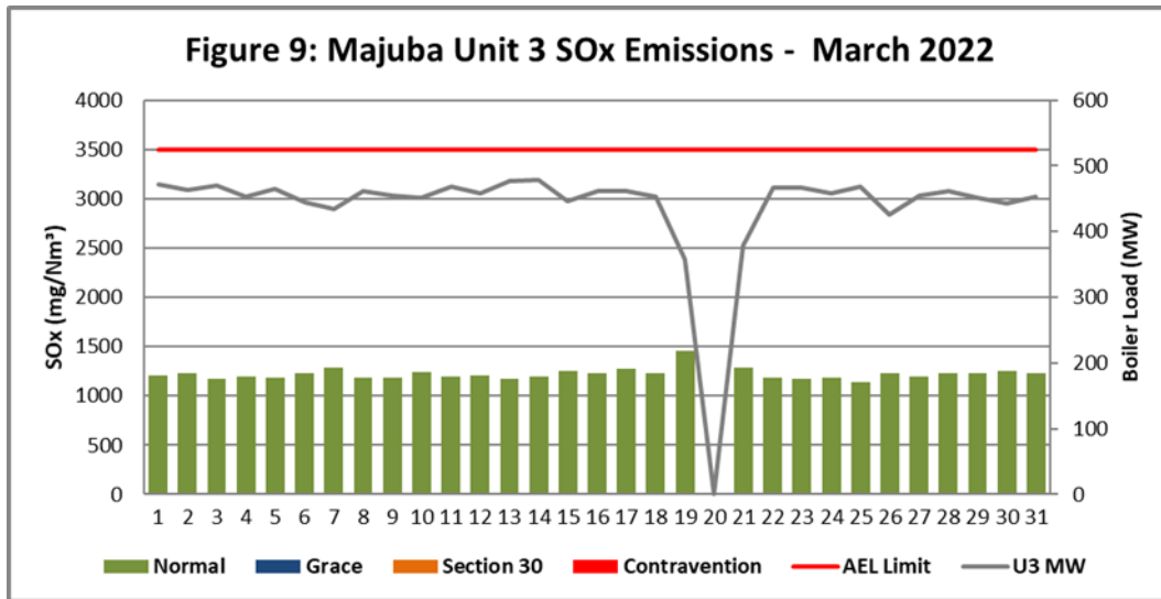
Figure 9. SOx emissions (daily averages) for the month of March 2022 against emission limit for Unit 3.
