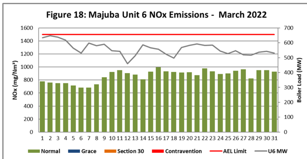
Figure 18. NOx emissions (daily averages) for the month March 2022 against emission limit for Unit 6
