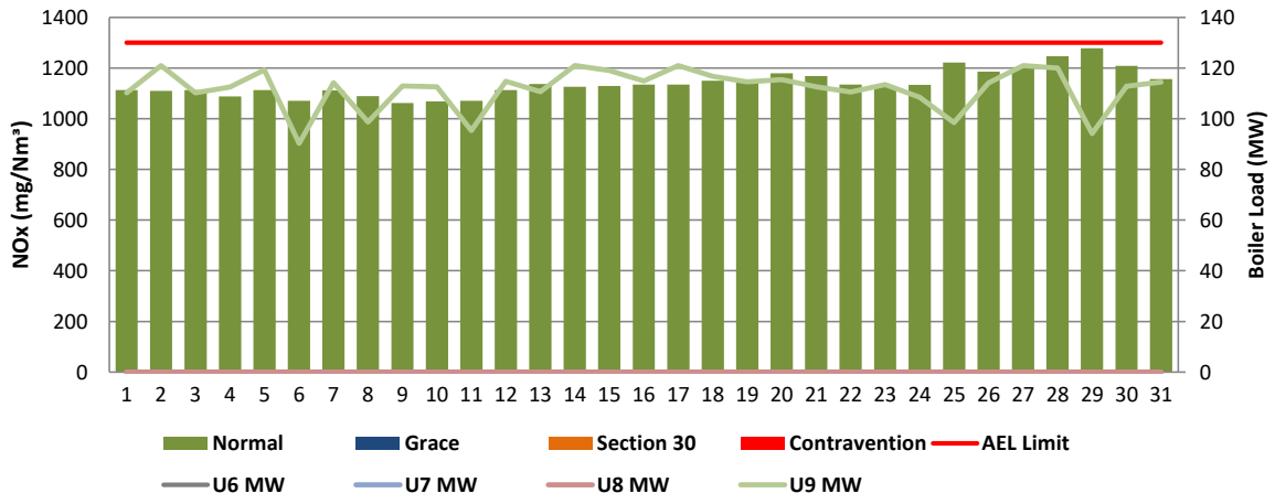
Figure 6: Komati West Stack NOx Emissions - May 2022
