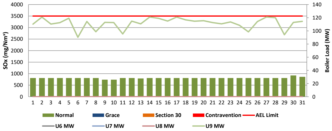
Figure 4: Komati West Stack SOx Emissions - May 2022
