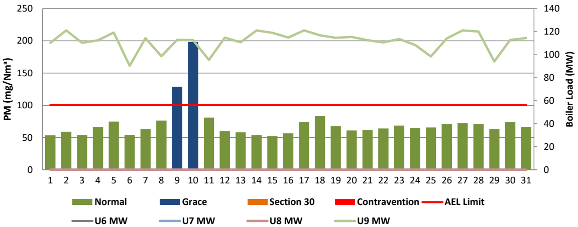
Figure 2: Komati West Stack PM Emissions - May 2022
