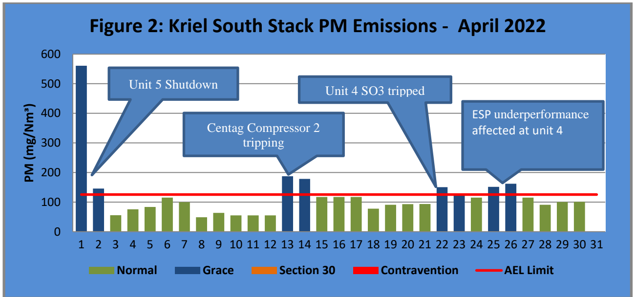
Figure 2: PM emissions for the month of April 2022 against emission limit for the South Stack. Monthly average was 120.1 mg/Nm 3
