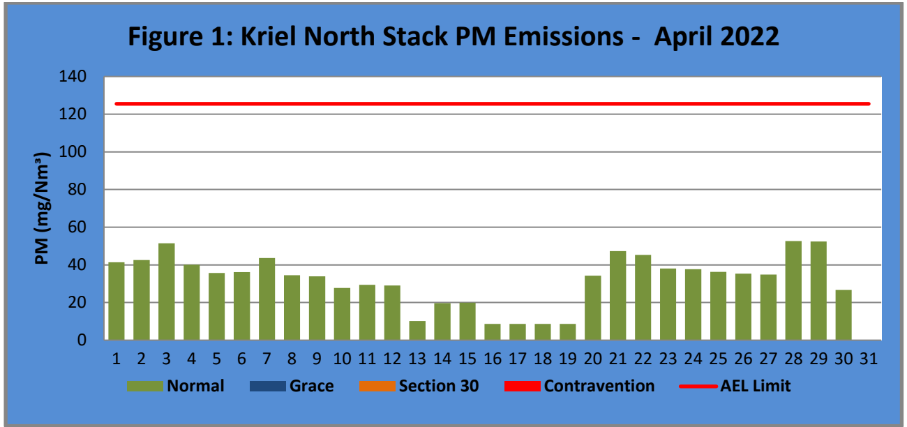
Figure 1: PM emissions for the month of April 2022 against emission limit for the North Stack. Monthly average was 32.4 mg/Nm 3
