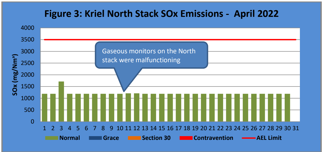
Figure 3. SO 2 emissions for the month of April 2022 against emission limit for the North Stack. The SO x Limit is 3500mg/Nm 3 .
