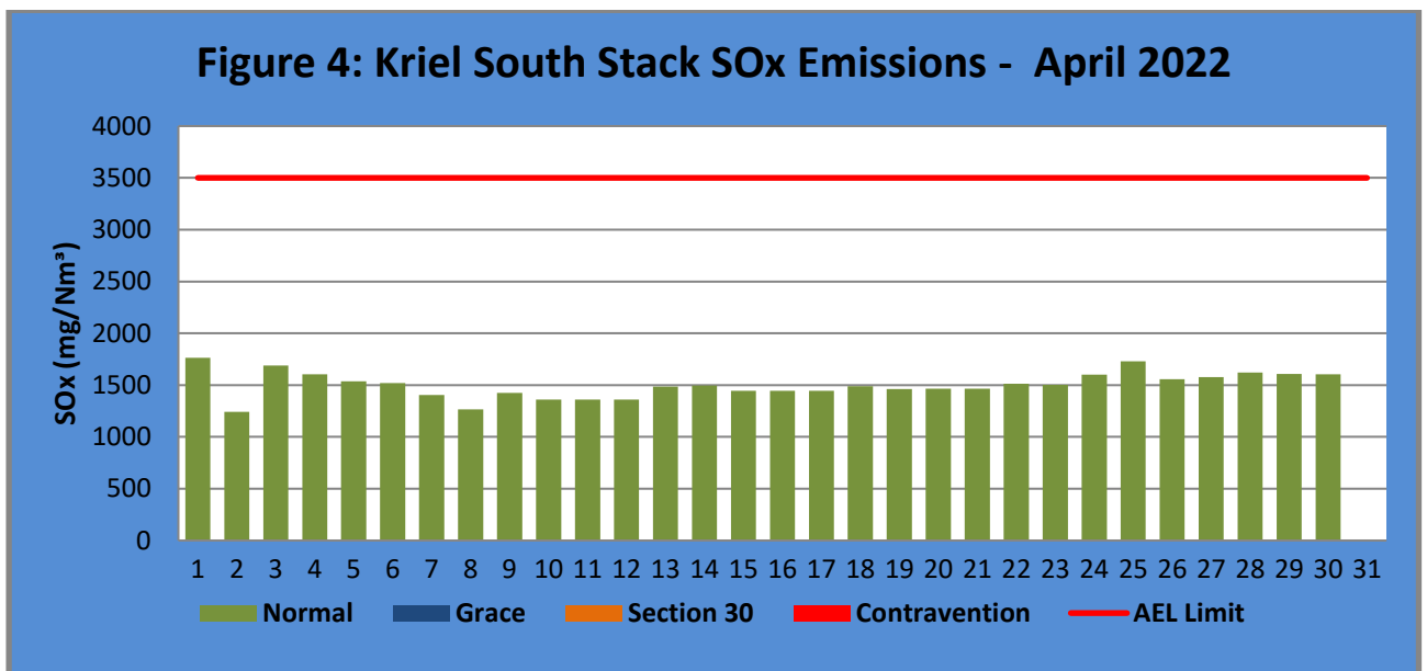
Figure 4. SO 2 emissions for the month of April 2022 against emission limit for the South Stack. The SO x Limit is 3500mg/Nm 3 .
