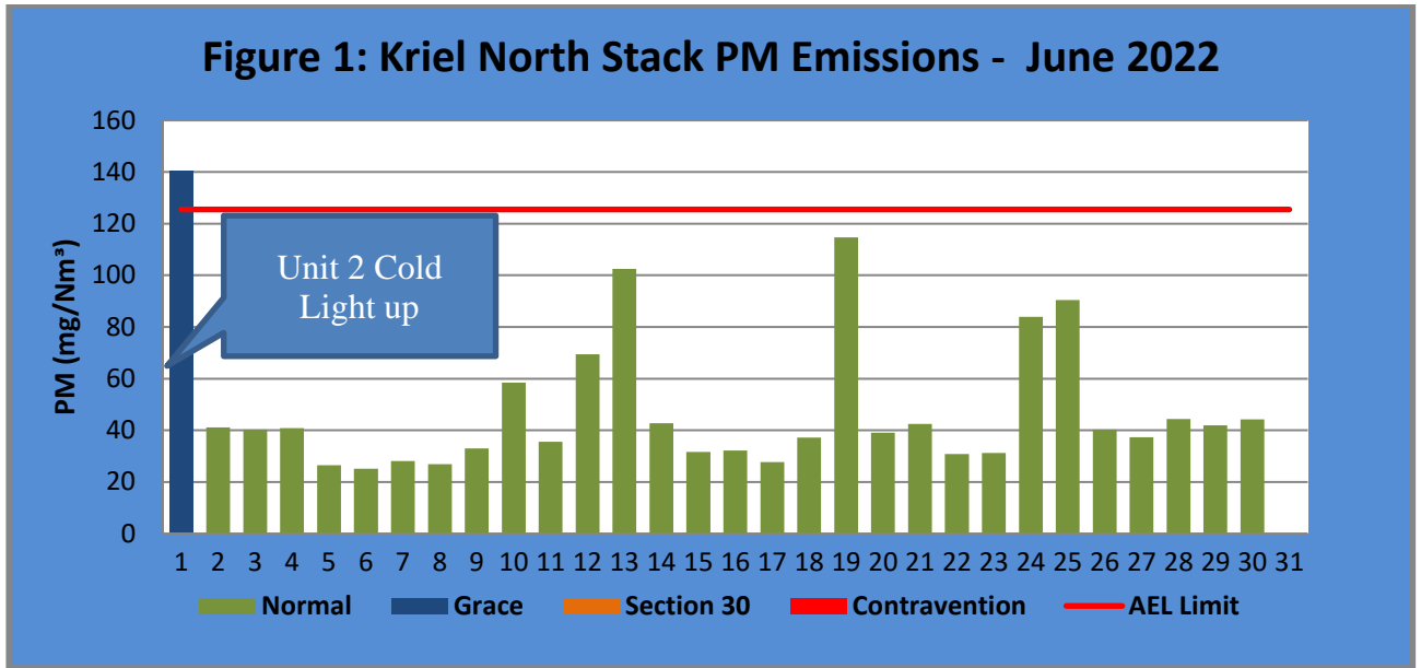
Figure 1: PM emissions for the month of June 2022 against emission limit for the North Stack. Monthly average was 49.3 mg/Nm 3
