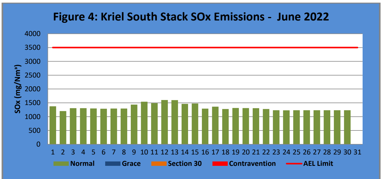
Figure 4. SO 2 emissions for the month of June 2022 against emission limit for the South Stack. The SO x Limit is 3500mg/Nm 3 .
