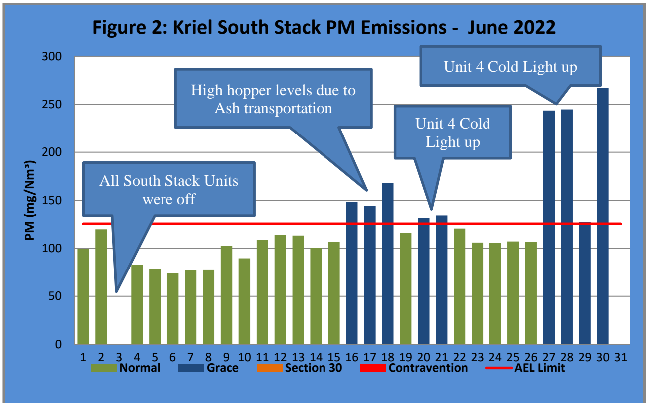
Figure 2: PM emissions for the month of June 2022 against emission limit for the South Stack. Monthly average was 124.6 mg/Nm 3
