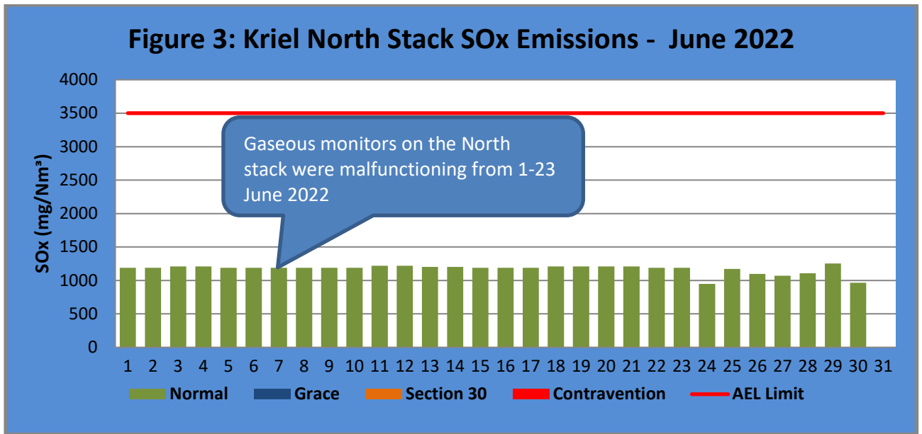
Figure 3. SO 2 emissions for the month of June 2022 against emission limit for the North Stack. The SO x Limit is 3500mg/Nm 3 .
