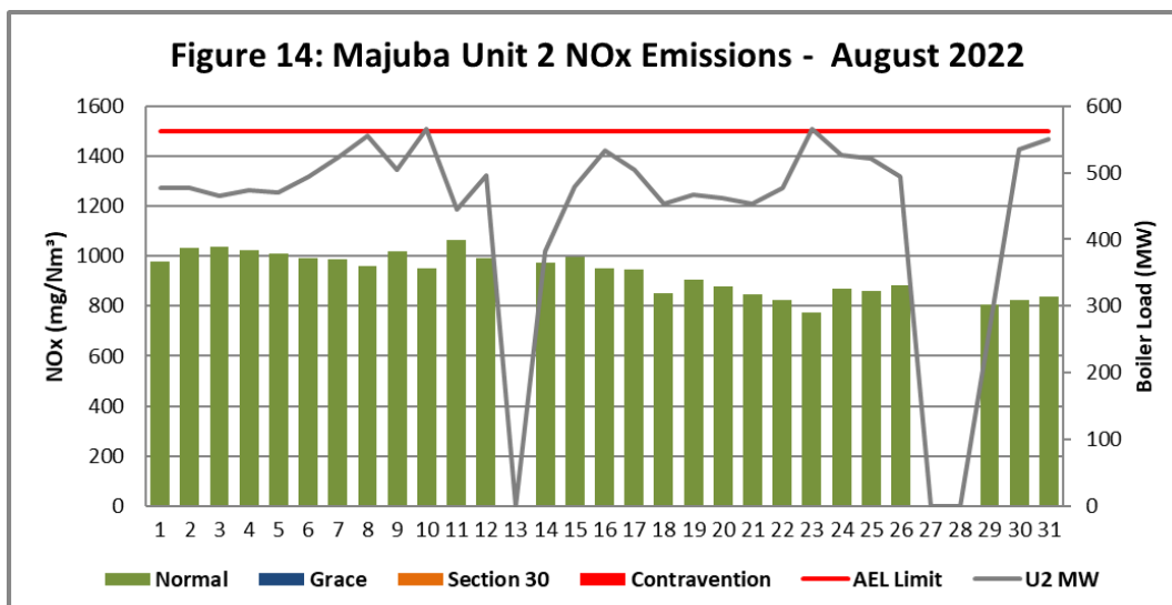
Figure 14. NOx emissions (daily averages) for the month of August 2022 against emission limit for Unit 2.
