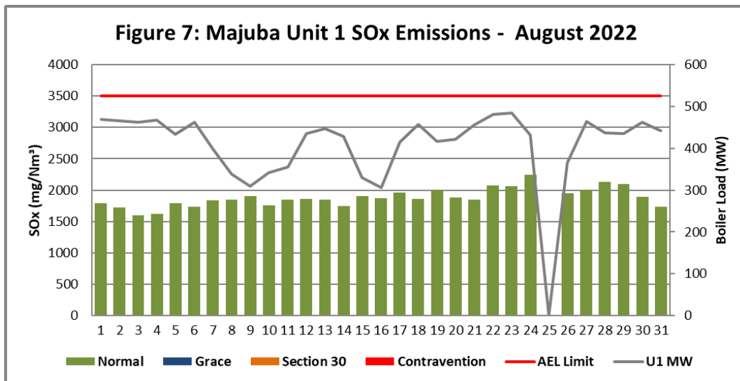
Figure 7. SOx emissions (daily averages) for the month of August 2022 against emission limit for Unit 1.
