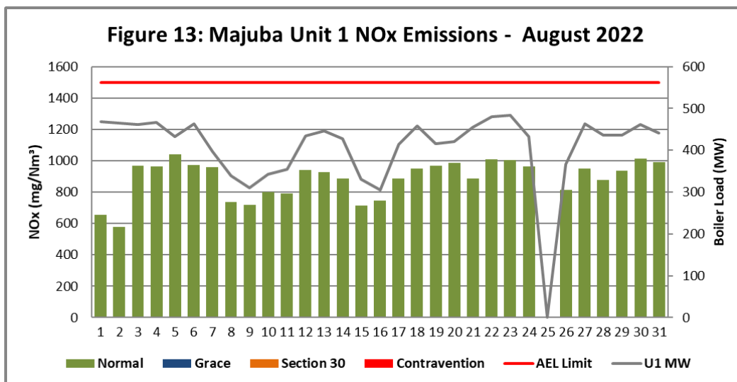
Figure 13. NOx emissions (daily averages) for the month of August 2022 against emission limit for Unit 1.
