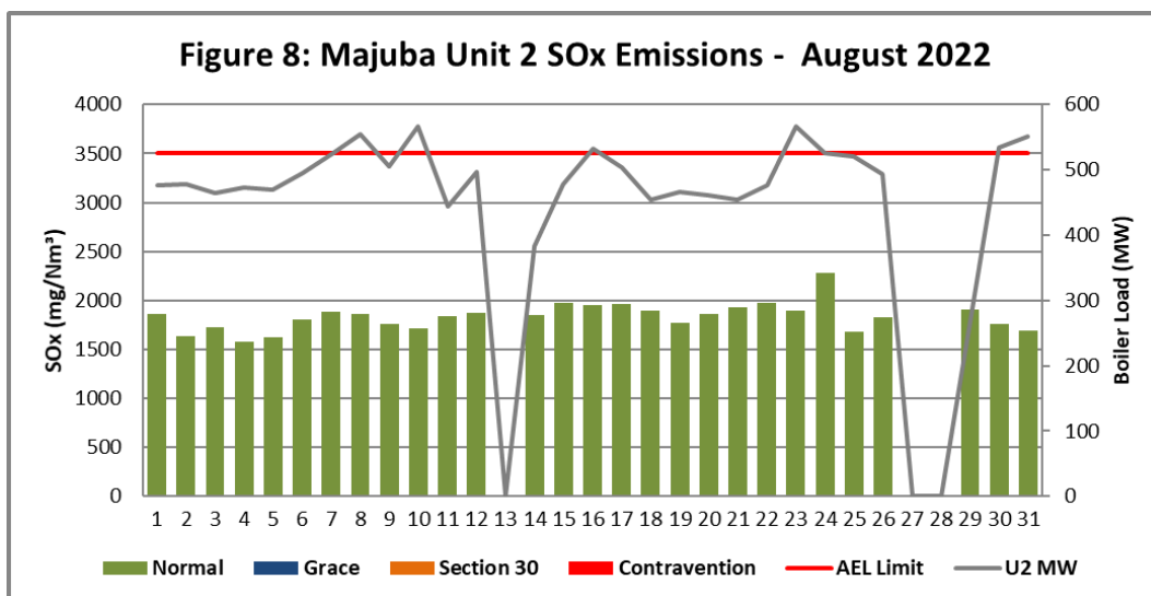
Figure 8. SOx emissions (daily averages) for the month of August 2022 against emission limit for Unit 2.
