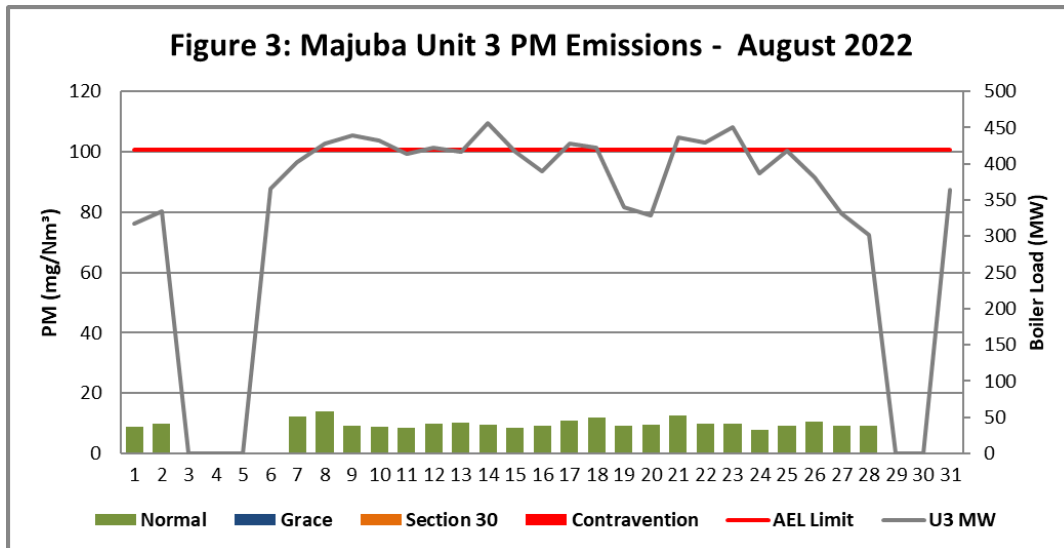
Figure 3. Particulate Matter emissions (daily averages) for the month of August 2022 against emission limit for Unit 3.
