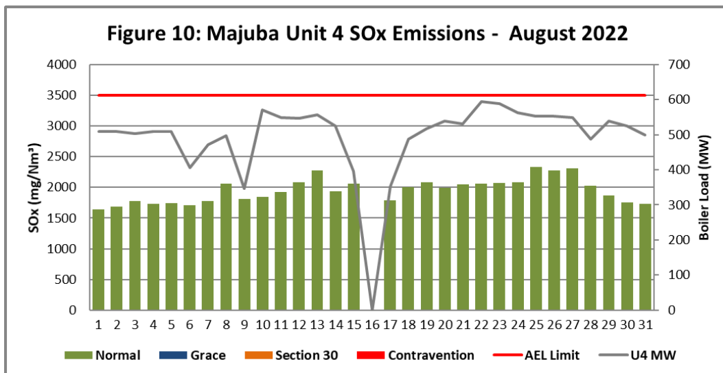
Figure 10. SOx emissions (daily averages) for the month of August 2022 against emission limit for Unit 4.
