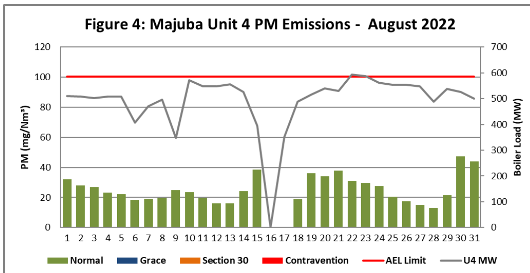
Figure 4. Particulate Matter emissions (daily averages) for the month of August 2022 against emission limit for Unit 4.
