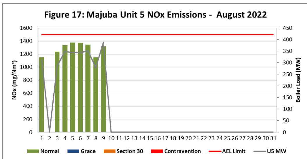
Figure 17. NOx emissions (daily averages) for the month of August 2022 against emission limit for Unit 5
