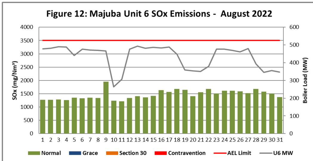
Figure 12. SOx emissions (daily averages) for the month of August 2022 against emission limit for Unit 6.
