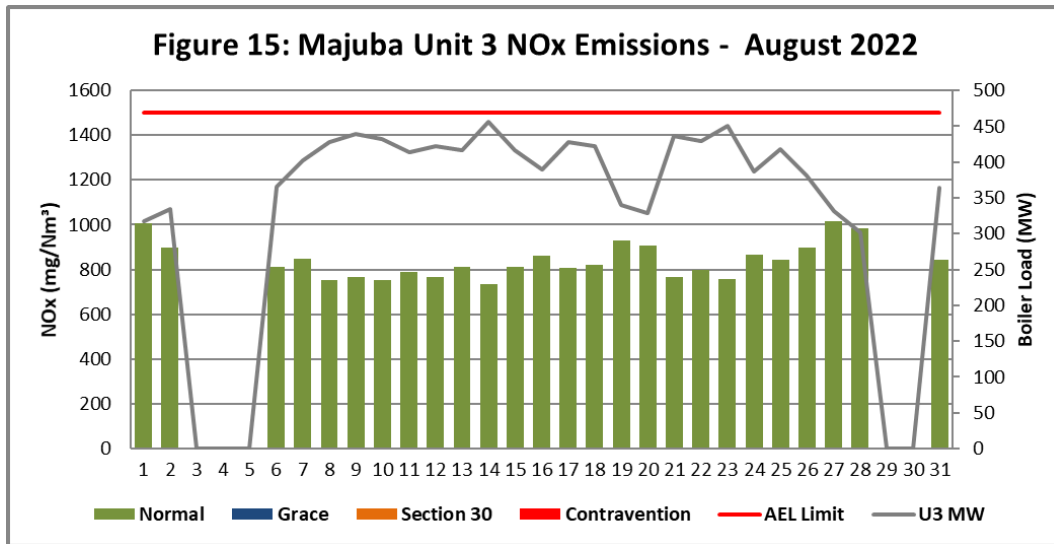
Figure 15. NOx emissions (daily averages) for the month of August 2022 against emission limit for Unit 3.
