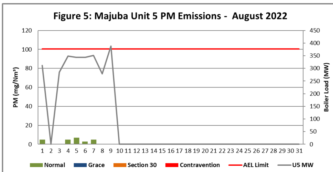
Figure 5. Particulate Matter emissions (daily averages) for the month of August 2022 against emission limit for Unit 5.
