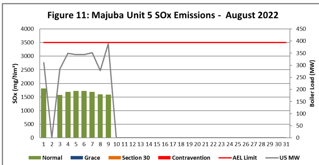
Figure 11. SOx emissions (daily averages) for the month of August 2022 against emission limit for Unit 5.
