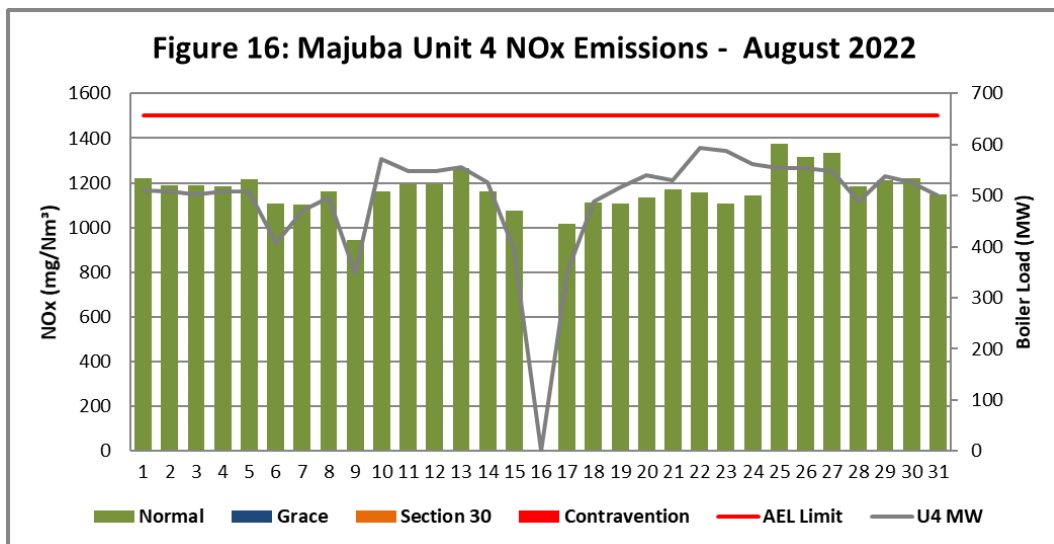
Figure 16. NOx emissions (daily averages) for the month of August 2022 against emission limit for Unit 4
