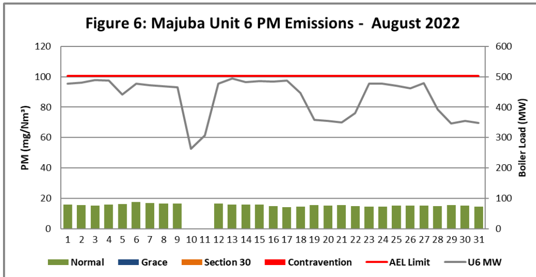
Figure 6. Particulate Matter emissions (daily averages) for the month of August 2022 against emission limit for Unit 6.
