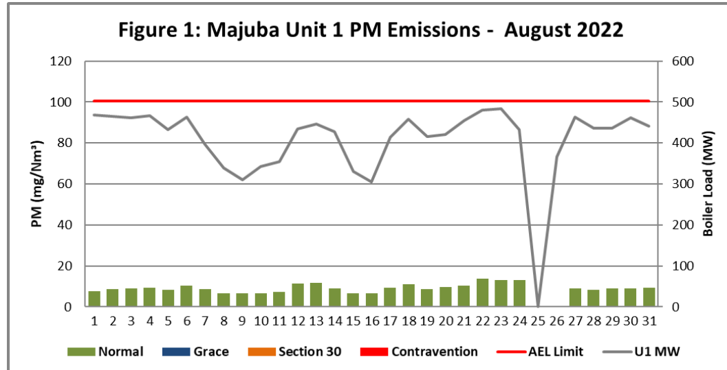
Figure 1. Particulate Matter emissions (daily averages) for the month of August 2022 against emission limit for Unit 1.
