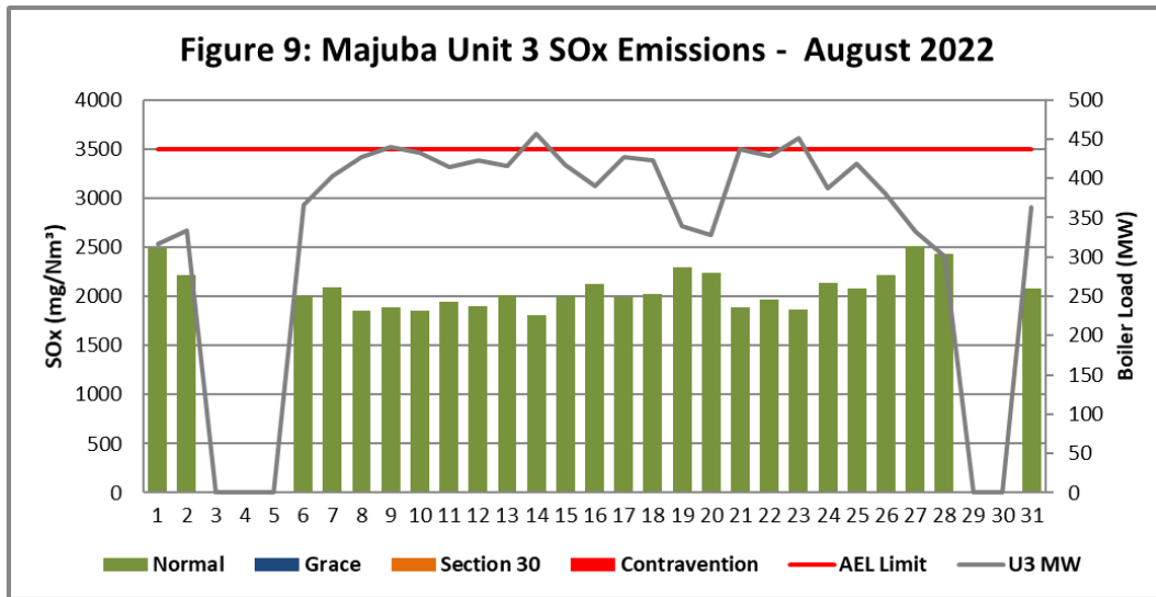
Figure 9. SOx emissions (daily averages) for the month of August 2022 against emission limit for Unit 3.
