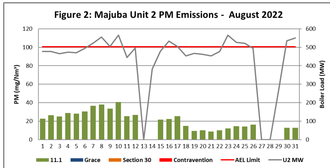
Figure 2. Particulate Matter emissions (daily averages) for the month of August 2022 against emission limit for Unit 2.
