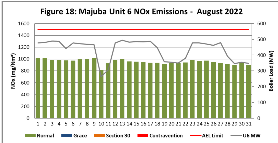
Figure 18. NOx emissions (daily averages) for the month August 2022 against emission limit for Unit 6
