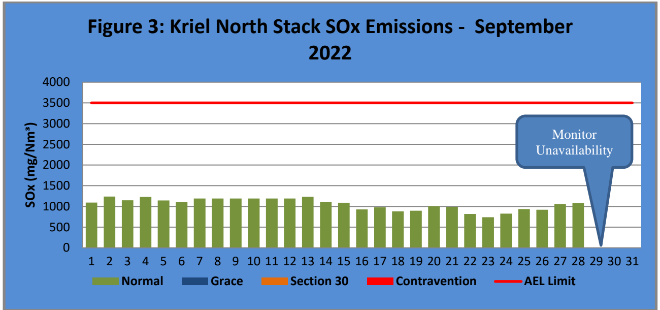
Figure 3. SO x emissions for the month of September 2022 against emission limit for the North Stack. The SO x Limit is 3500mg/Nm 3 .
