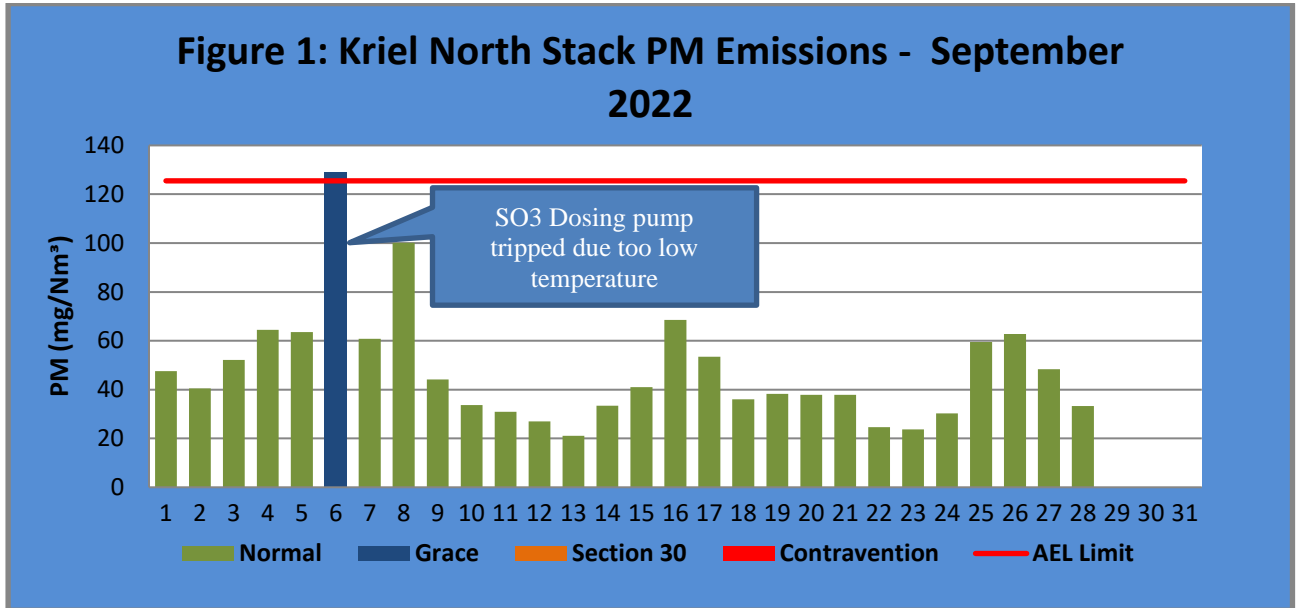
Figure 1: PM emissions for the month of September 2022 against emission limit for the North Stack. Monthly average was 48.0 mg/Nm3
