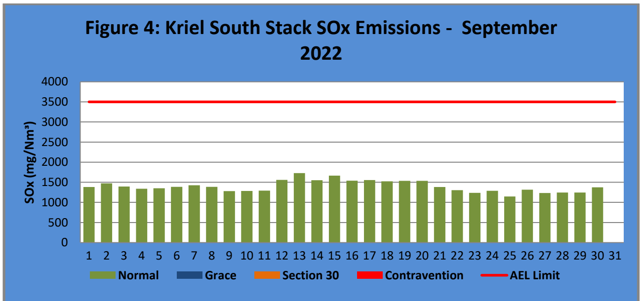
Figure 4. SO x emissions for the month of September 2022 against emission limit for the South Stack. The SO x Limit is 3500mg/Nm 3 .
