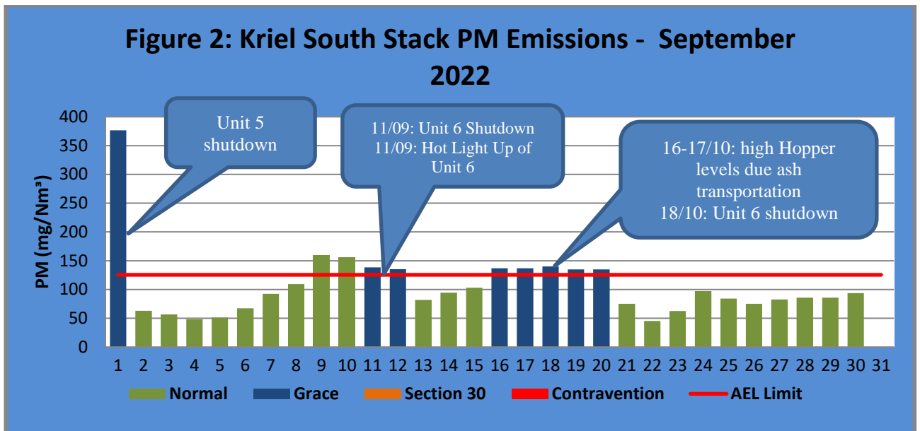
Figure 2: PM emissions for the month of September 2022 against emission limit for the South Stack. Monthly average was 106.8 mg/Nm3
