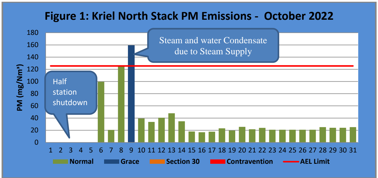
Figure 1: PM emissions for the month of October 2022 against emission limit for the North Stack. Monthly average was 37.3 mg/Nm 3
