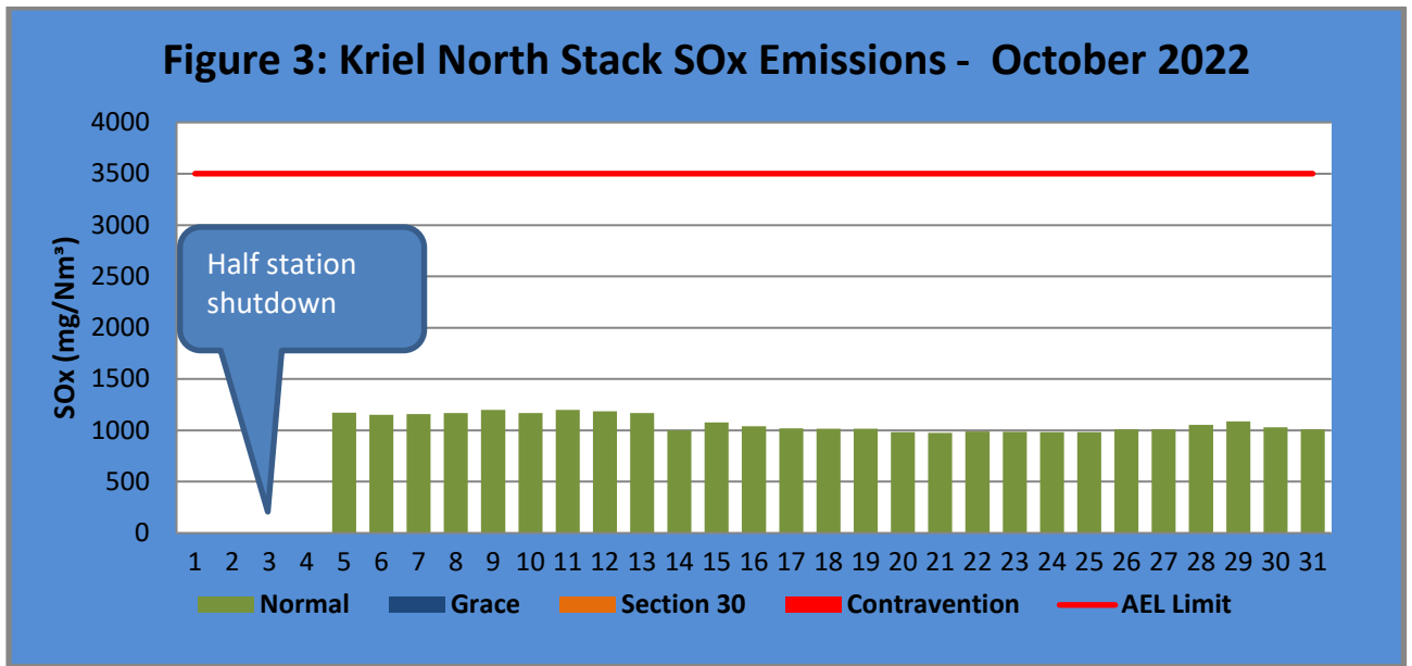
Figure 3. SO 2 emissions for the month of October 2022 against emission limit for the North Stack. The SO x Limit is 3500mg/Nm 3 .
