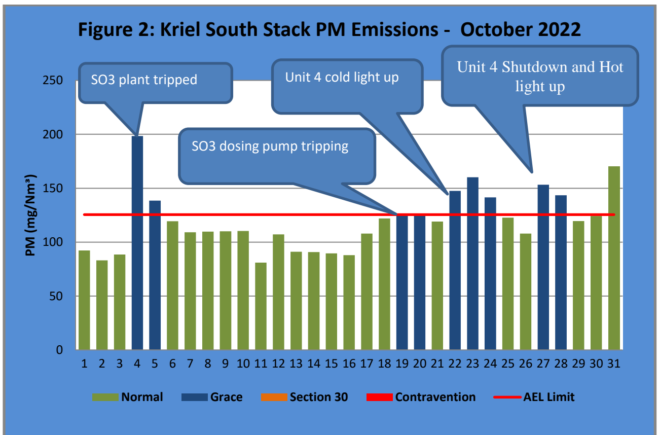
Figure 2: PM emissions for the month of October 2022 against emission limit for the South Stack. Monthly average was 119.3 mg/Nm 3
