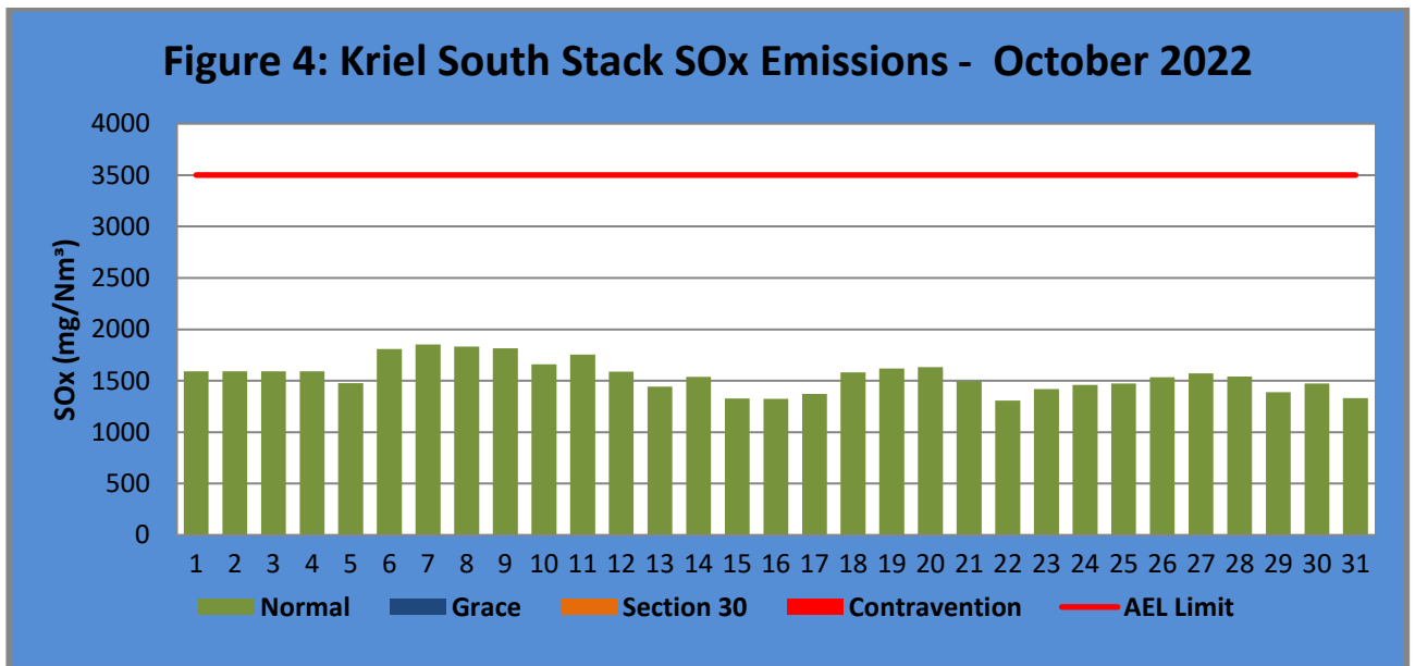
Figure 4. SO 2 emissions for the month of October 2022 against emission limit for the South Stack. The SO x Limit is 3500mg/Nm 3 .
